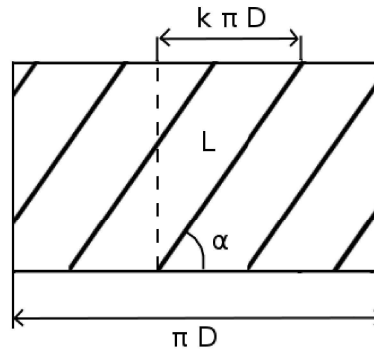
Fig.II.15_ braided geometry
