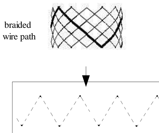
Fig III.23_ Plane representation of the braided wire path on a cylindrical braid surface
