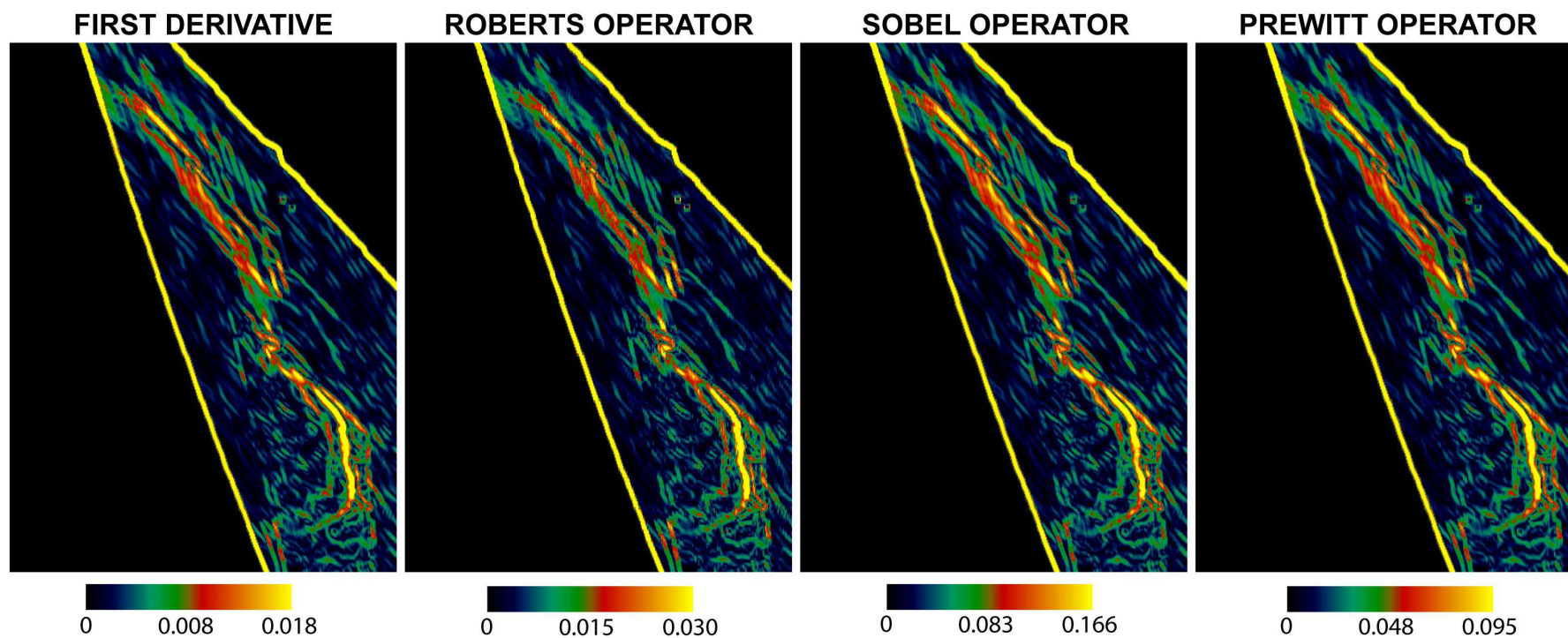
FIGURE 8.5 – Comparison of contours detected by the gradient method and by the Sobel/Roberts/Prewitt edge detection operators on the VIMS T38 image at 5\ \mu\text{m} . Pixels in each panel are color-coded according to the value of the corresponding operator. All these operators give similar edge detections (Table 8.2).
