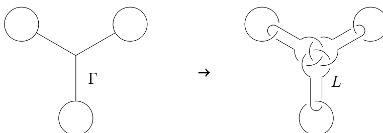
Figure 1: The standard Y-graph
