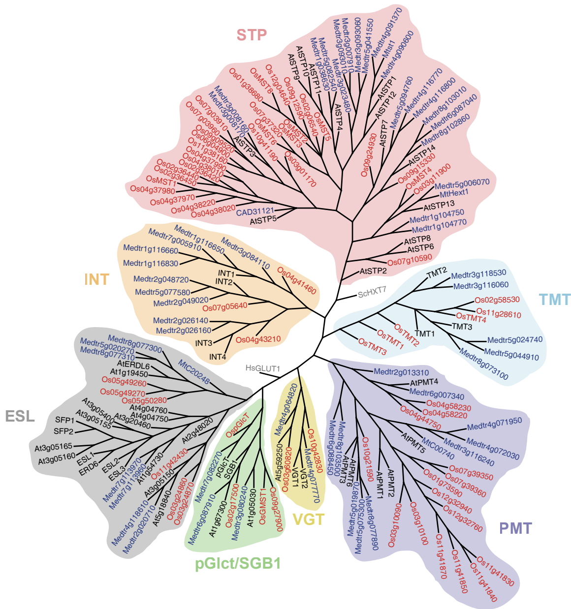
Figure 36. Phylogenetic tree of the MST family in A. thaliana , M. truncatula and rice
