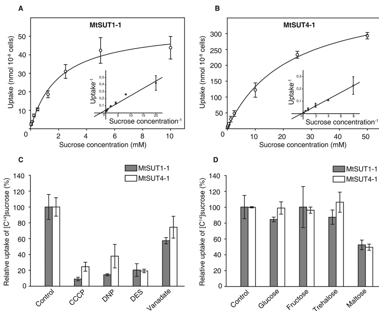
Figure 3. Biochemical Characterization of MtSUT1-1 and MtSUT4-1.
