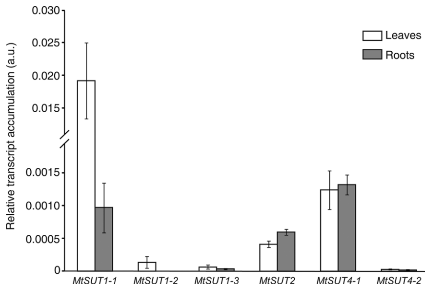
Figure 4. Analysis of Transcript Level of MtSUT Genes. Quantitative reverse transcription polymerase chain reaction (q-RT-PCR) analysis of MtSUT1-1 , MtSUT1-2 , MtSUT1-3 , MtSUT2 , MtSUT4-1 , and MtSUT4-2 in leaves (white bar) and roots (tinted bar) of plants treated with high-phosphate 1.3 mM conditions (HP). Data are expressed in arbitrary units (a.u.).
