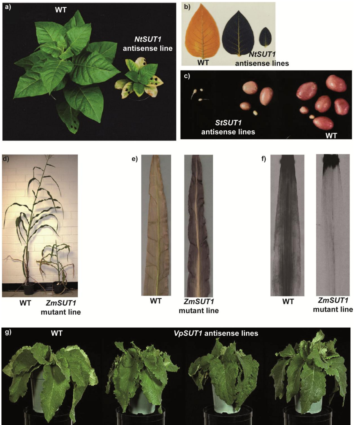
Fig 9. A single SUT protein is necessary for phloem loading in apoplasmic loader plants a) Phenotype of wild type and NtSUT1 antisense tobacco plants (Burkle et al. 1998). b) Starch accumulation in leaves of wild type and NtSUT1 antisense tobacco plants shown by Lugol's iodine staining. c) Reduction of tuber yield in potato tubers in StSUT1 antisense line \alpha SUT43 and \alpha SUT13 (Riesmeier et al. 1994). d) Phenotype of wild type and ZmSUT1 insertional mutant maize plants (Slewinski et al. 2009). e) Starch accumulation in leaves of wild type and ZmSUT1 mutant plants shown by Lugol's iodine staining. f) Autoradiographs showing the blockage of [ ^{14} C]sucrose export from ZmSUT1 mutant leaves. g) No phenotype differences were observed in the symplasmic loader ( Verbascum phoeniceum ) between wild type and VpSUT1 antisense lines (Zhang and Turgeon 2009).
