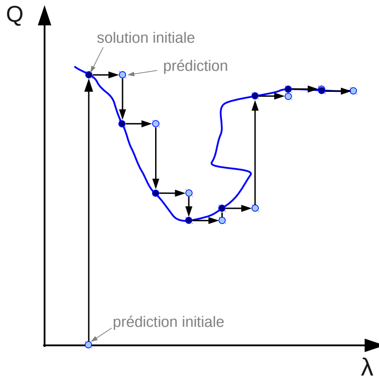
FIGURE 2.3: Continuation incrémentale
