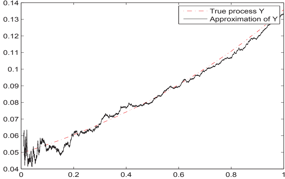
Figure 3.1: Approximation of process \widehat{Y} to Y .
