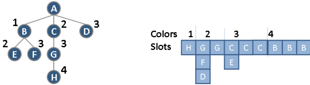
(a) Example of colored tree.
