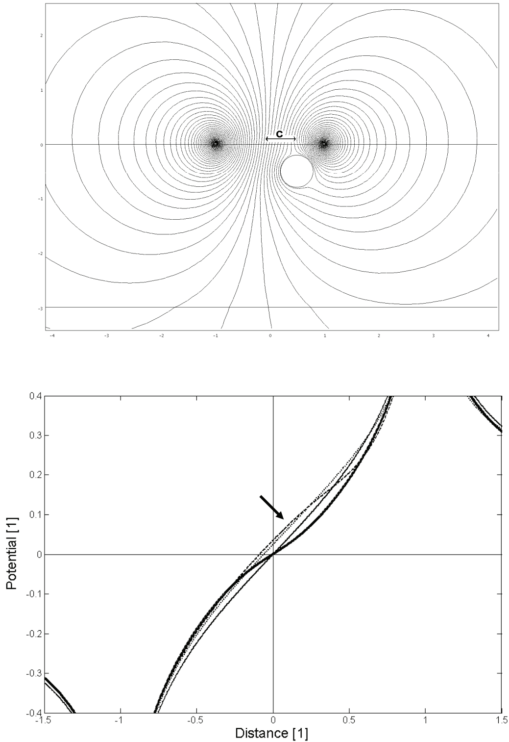
Figure 62: Potential distribution near a dipole lying on a stratified medium comprising a spherical heterogeneity. Top: equipotential lines in a plane containing the dipole axis and the heterogeneity centre, and perpendicular to the surface, with \epsilon_1=1 , \epsilon_2=2 , \epsilon_3=3 , a=2 , and b=3 . Bottom: potential profiles along the dipole axis, with c=0 (solid); c=0.5 (dashed); c=1 (dotted); and without heterogeneity (thick solid). The arrow shows the region of maximum sensitivity that is the most suitable location for the receivers.
