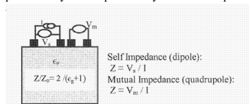
Figure 1. Principle of ground complex permittivity measurement with self and mutual impedance probes.
