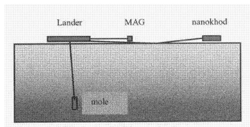
Figure 5. Tentative set-up of a permittivity instrument on BepiColombo.
