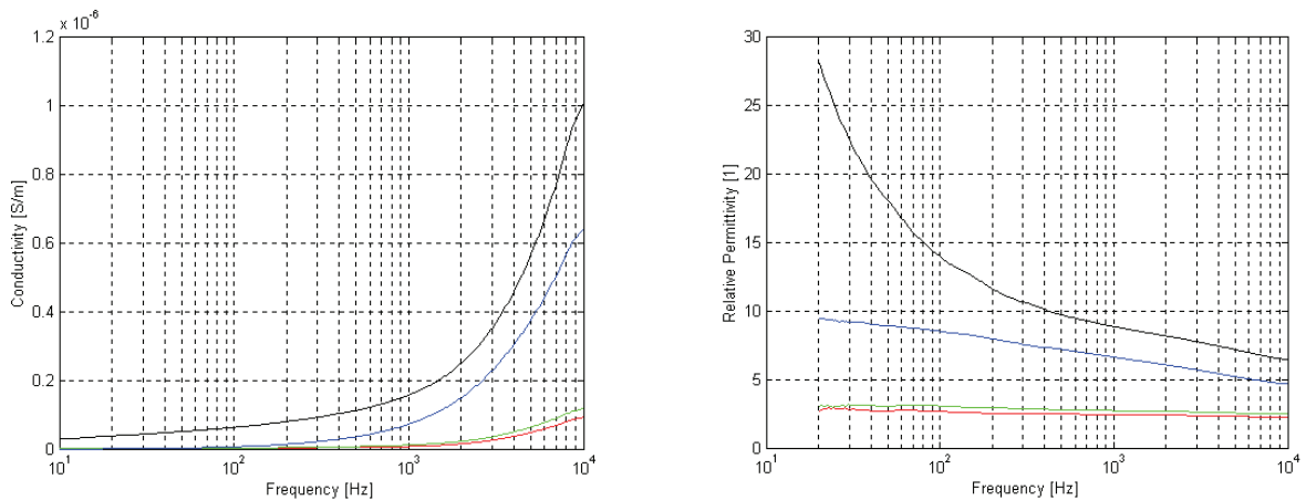
Figure 53: Same caption as for Figure 52, but at a temperature T = -25^\circ\text{C} .
