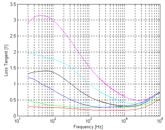
Fig. 5. Loss tangent of the JSC Mars-1 simulant, for \theta = 0.1 , \phi = 0.54 and temperature: T = -55^\circ\text{C} (red), -40^\circ\text{C} (green), -25^\circ\text{C} (blue), -10^\circ\text{C} (black), +5^\circ\text{C} (cyan), and +20^\circ\text{C} (magenta).
