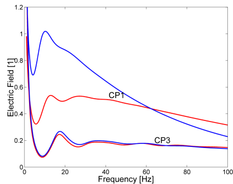
Figure 4. Electric field as a function of frequency for the two conductivity profiles and cavity configurations ( R_{\text{int}}=R_T-100\text{km} – red, R_{\text{int}}=R_T – blue). The soil properties, whenever applicable, use default values. The electromagnetic source is a small pulsating sphere located at an altitude of 35 km and the angular separation (the angle between the source and the receiver as seen by an observer at the centre of the planet) is 45^\circ .
