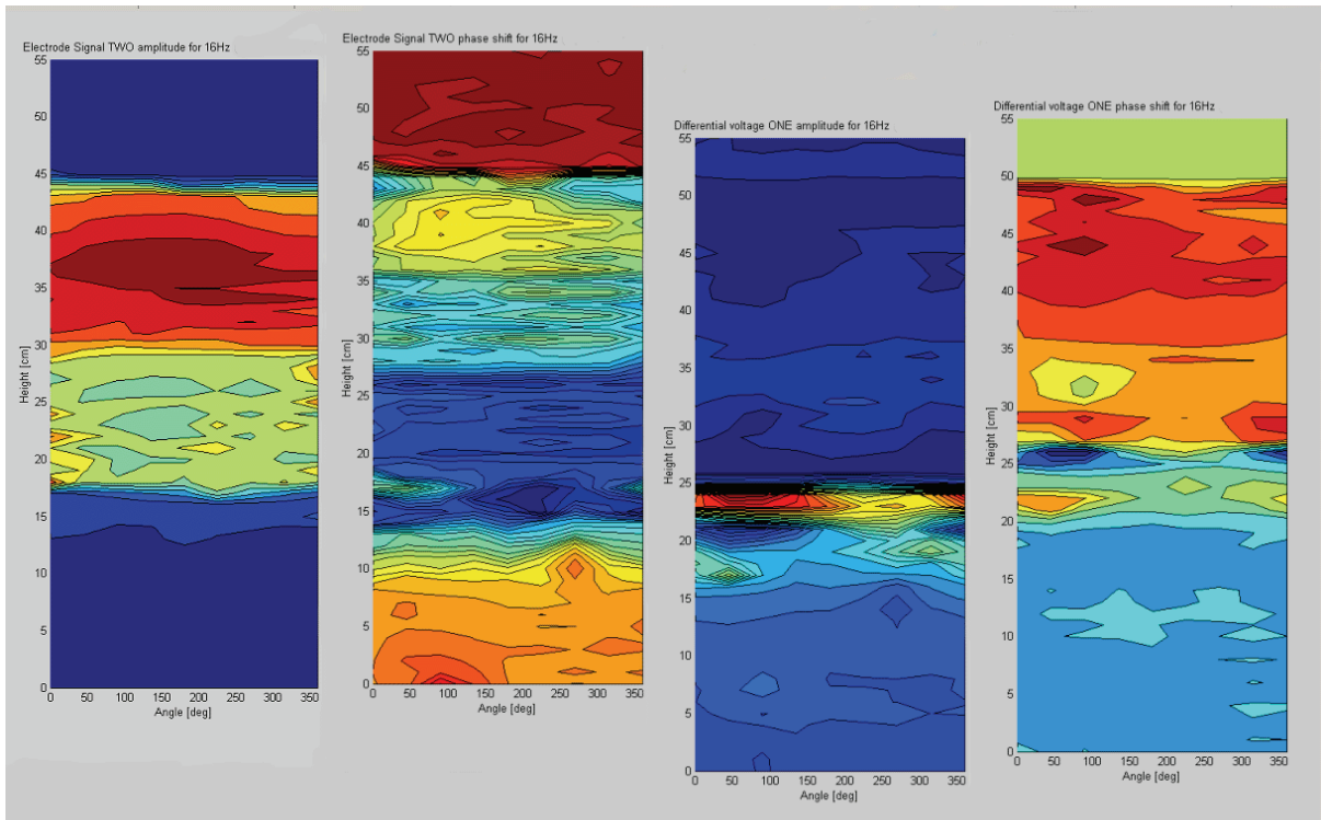
Figure 57: 2D raw electric maps of the stratified medium recorded with the electrodes of larger size (sectors of 270^\circ ), at 16 Hz. Depth is plotted against angle; the arbitrary colour code represents either amplitude or phase. From left to right: amplitude of the Tx signal; phase shift of the Tx signal; Rx amplitude; Rx phase shift.
