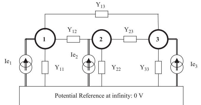
Fig. 3. Equivalent circuit of a system of three conductors in an uniform medium (the currents injected by the instrument in the medium, I_{e1} \dots I_{e3} , are represented by double lines).
