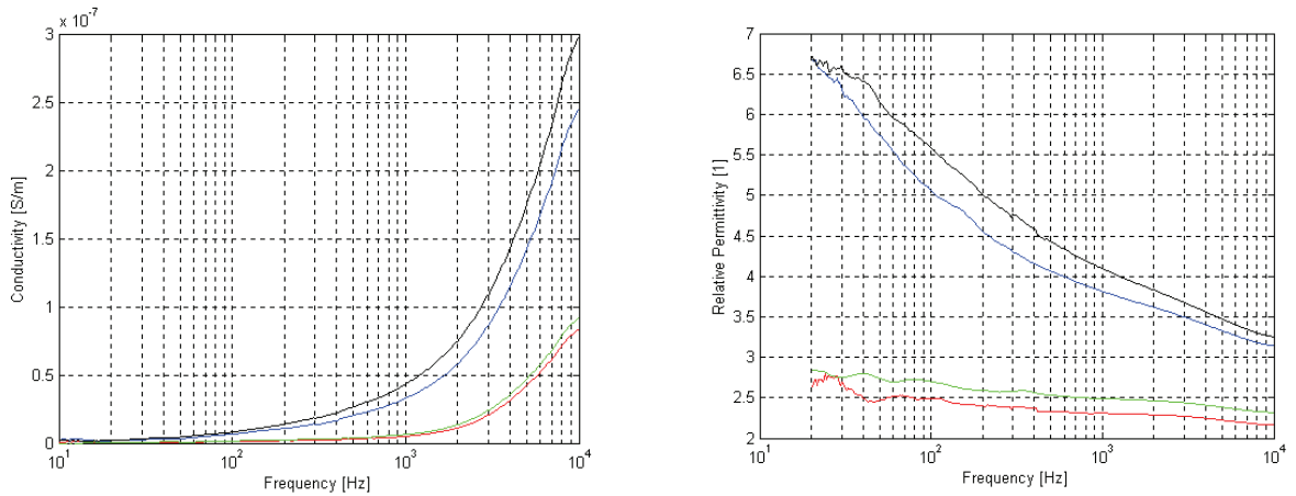
Figure 52: Conductivity (left) and relative dielectric constant (right) of the JSC Mars-1 simulant as functions of frequency, at \phi = 0.54 and T = -55^\circ\text{C} , with different gravimetric water contents: \theta < 0.005 (red), \theta = 0.01 (green), \theta = 0.05 (blue), and \theta = 0.1 (black).
