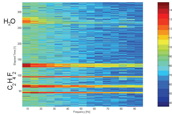
Figure 29: Dynamic spectrum, elapsed time against frequency, in the range 3-99 Hz, obtained by spraying fresh water and difluoroethane ( C_2H_4F_2 ) hazes on the antenna. The colour scale, in arbitrary units, represents the potential measured with the digital processor unit.
