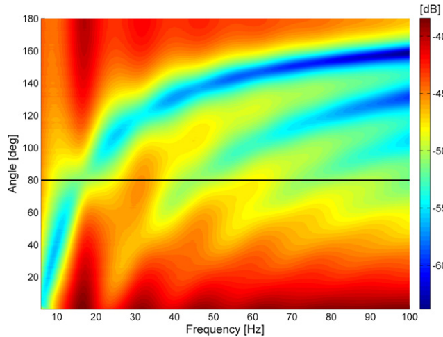
Fig. 9. Map of the electric field amplitude (arbitrary normalized units) received from an isotropic EM source located at 200 km altitude, versus frequency, as a function of angular distance, at the altitude of 100 km (see text).
