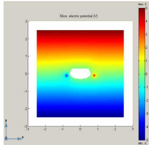
Figure 4 - Slice in the plane z=0 that shows the electric potential distribution generated by the two relaxation probes and the vertical electric field (Model B).
