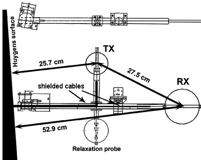
Fig. 6. Boom configuration and sensor lay-out, with the characteristic distances used in the SCD code.
