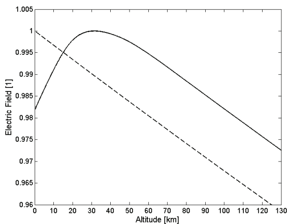
Figure 7: Electric field amplitude as a function of altitude in a lossless Venus cavity with PEC boundaries, where R_{int}=R_v , R_{ext}=R_v+h , and h=130 km, for R_v=6052 km. The permittivity is given by a specific profile (solid line) or is assumed to be that of vacuum (dashed line). The field magnitude is normalized to that of the vertical component on the surface in vacuum. See Figure 6 for details about the permittivity profile.
