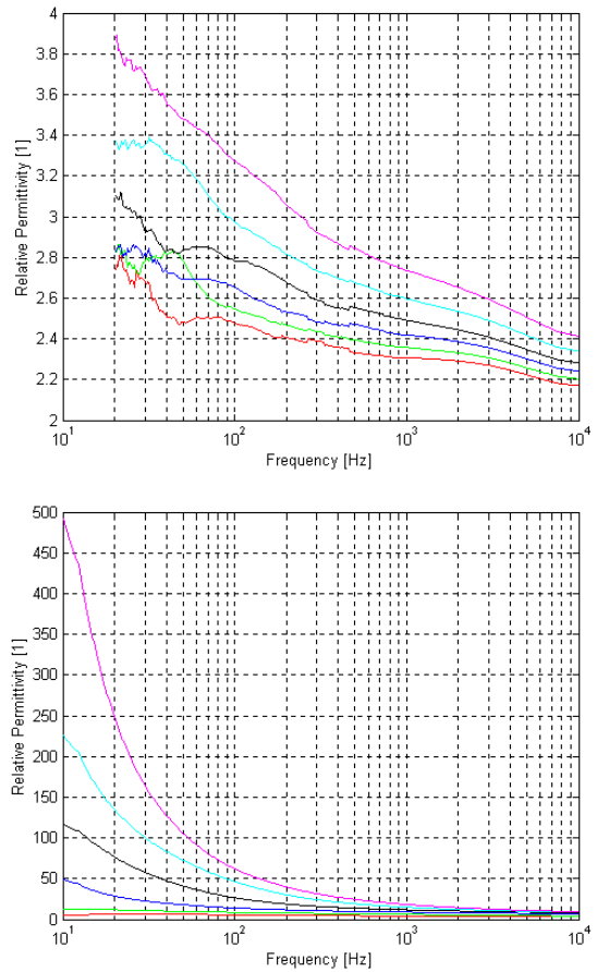
Fig. 4. Relative dielectric constant of the JSC Mars-1 simulant with gravimetric water contents \theta < 0.005 (top) and \theta = 0.1 (bottom), as functions of frequency, for \phi = 0.54 and temperatures: T = -55^\circ\text{C} (red), -40^\circ\text{C} (green), -25^\circ\text{C} (blue), -10^\circ\text{C} (black), +5^\circ\text{C} (cyan), and +20^\circ\text{C} (magenta).
