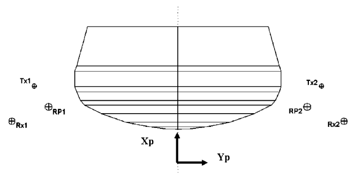
Fig. 4. Geometrical model of Huygens and MIP–RP electrodes used in Comsol Multiphysics™ software (Huygens revolution axis: Xp).
