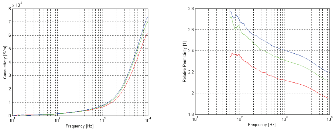
Figure 51: Conductivity (left) and relative dielectric constant (right) of the dry JSC Mars-1 simulant ( \theta < 0.005 ), as functions of frequency, at a temperature T = +20^\circ\text{C} , for different porosities: \phi = 0.58 (red), \phi = 0.54 (green), and \phi = 0.52 (blue).
