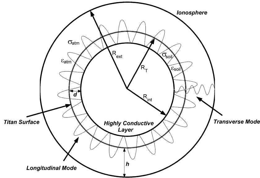
Fig. 1. Sketch of the model used for calculating the Schumann resonance on Titan. R_T : Titan radius; R_{int} : liquid layer radius; R_{ext} : ionosphere radius; h : altitude of the ionosphere; d : depth of the solid–liquid interface layer; \epsilon_{soil} , \epsilon_{atm} , \sigma_{soil} , \sigma_{atm} : permittivities and conductivities of the soil and atmosphere, respectively.
