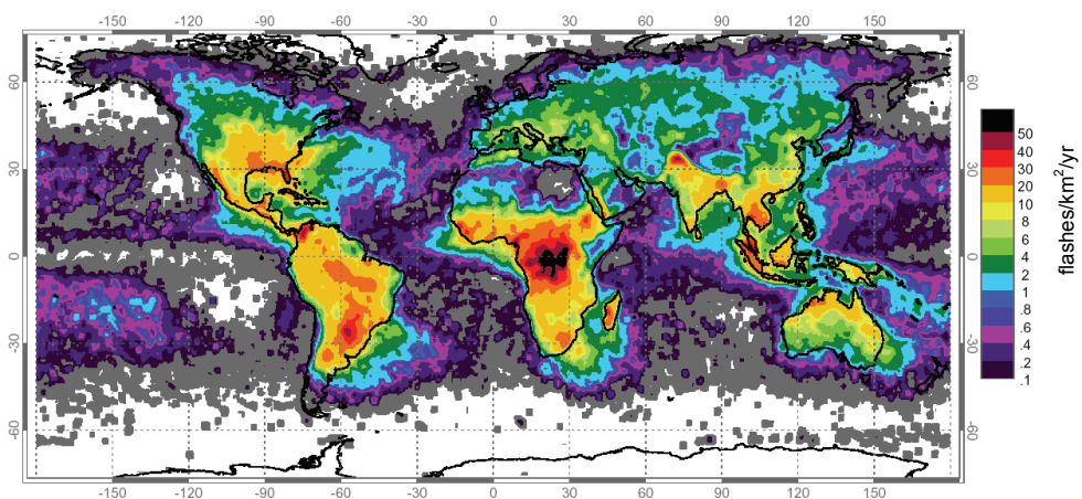
Figure 2: Satellite observation of global lightning distribution. (Credit: GSFC-NASA, National Space Science and Technology Centre Lightning Team).
