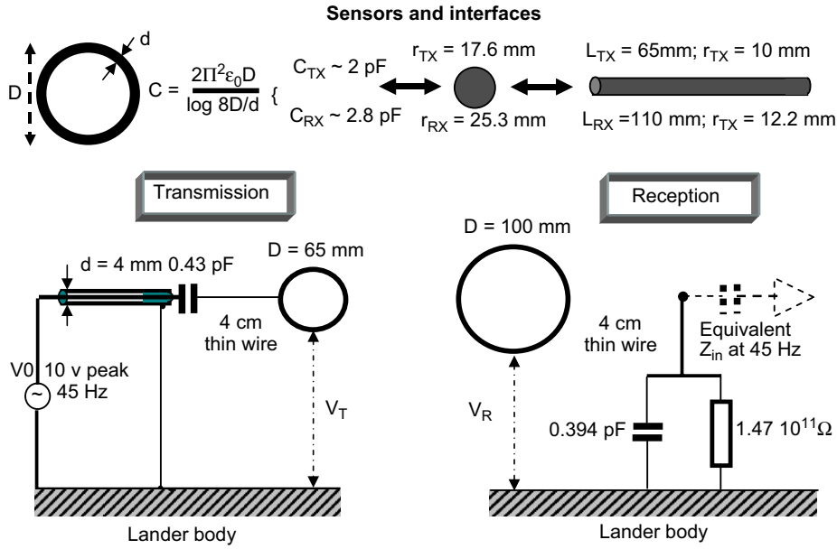
Fig. 7. Modelling of the rings and equivalent circuits of the transmission and reception units. Rings are represented by either spheres or cylinders of equivalent capacitance (see text).
