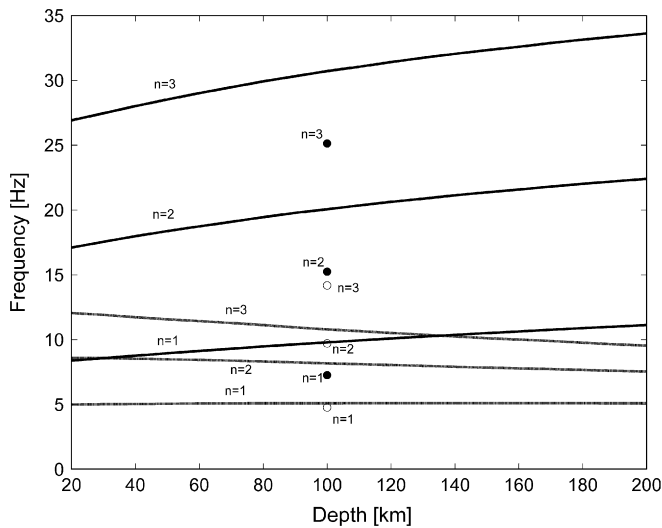
Fig. 6. The three lowest eigenfrequencies of the cavity as functions of the PEC depth, for \sigma_{\text{atm}} = \text{CP1} , \epsilon_{\text{soil}} = 3 , and \sigma_{\text{soil}} = 10^{-9} \text{ S m}^{-1} (lines and symbols as in Fig. 4).
