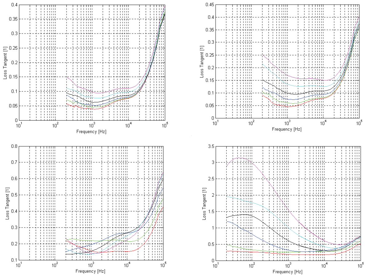
Figure 55: Loss tangent of the JSC Mars-1 simulant, with gravimetric water content \theta < 0.005 (top left), \theta = 0.01 (top right), \theta = 0.05 (bottom left), and \theta = 0.1 (bottom right), as function of frequency, for \phi = 0.54 and at different temperatures: T = -55^\circ\text{C} (red), -40^\circ\text{C} (green), -25^\circ\text{C} (blue), -10^\circ\text{C} (black), +5^\circ\text{C} (cyan), and +20^\circ\text{C} (magenta).
