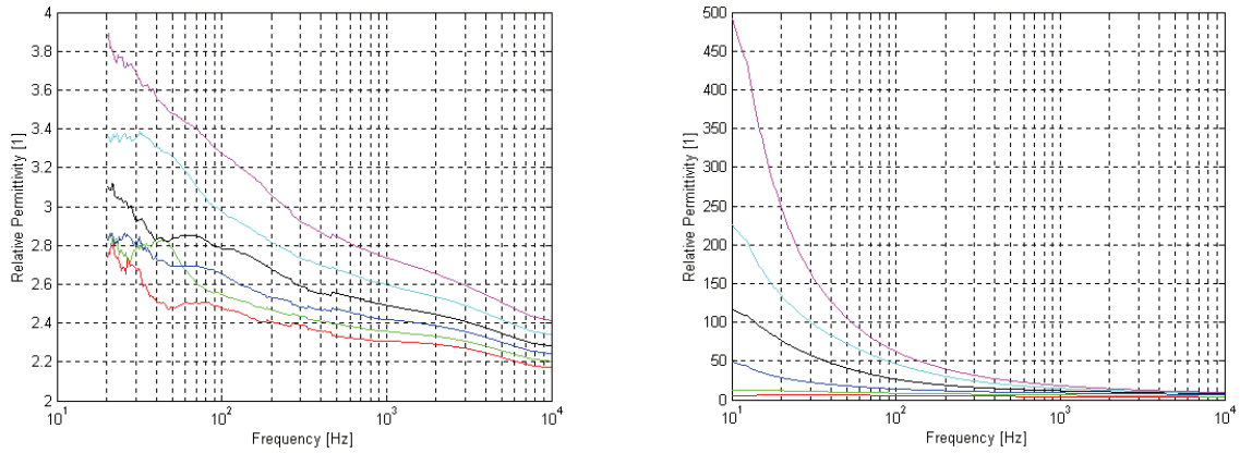
Figure 54: Relative dielectric constant of the JSC Mars-1 simulant with gravimetric water contents \theta < 0.005 (left) and \theta = 0.1 (right), as functions of frequency, for \phi = 0.54 and at different temperatures: T = -55^\circ\text{C} (red), -40^\circ\text{C} (green), -25^\circ\text{C} (blue), -10^\circ\text{C} (black), +5^\circ\text{C} (cyan), and +20^\circ\text{C} (magenta).
