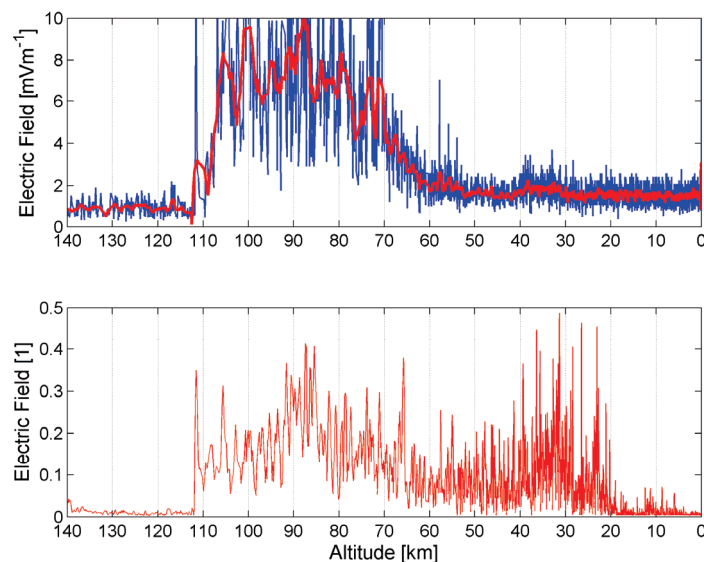
Figure 31: Comparison between the 36 Hz signal and the electric field theoretical profile derived from the Schumann model in the range 0-140 km. Top : Electric field profile measured at 36 Hz. Bottom : Electric field theoretical profile taking into account the antenna tilt.
