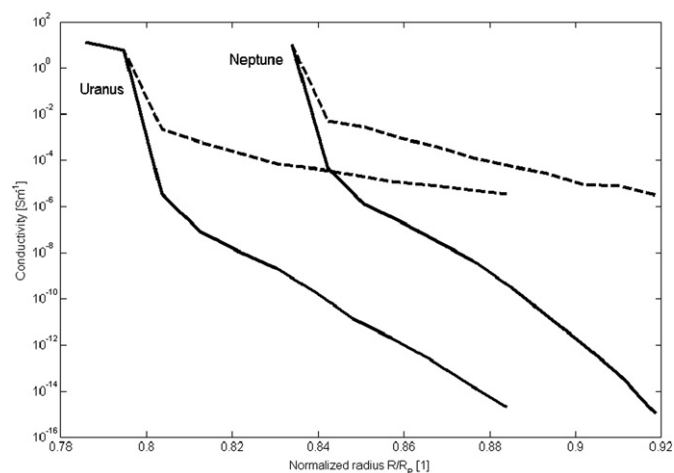
Fig. 9. Conductivity profiles of Uranus and Neptune interiors for gravimetric water contents of 0% (solid) and 15% (dashed).
