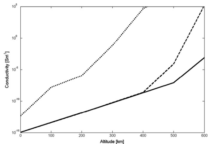
Fig. 10. Atmospheric conductivity profiles of Uranus (solid—ingress; dashed—egress) and Neptune (dotted).
