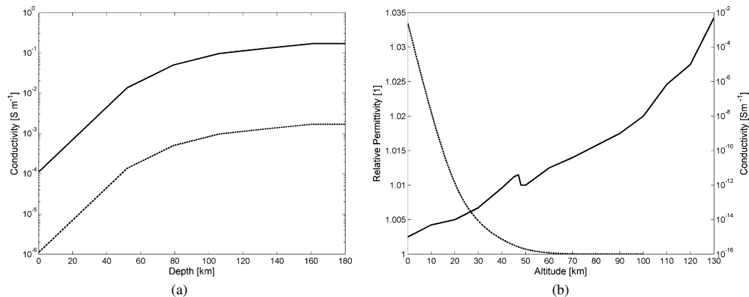
Fig. 2. Dielectric parameters of the venusian cavity. Left: Conductivities as functions of depth for high (solid) and low (dashed) surface conductivities; right: conductivity (solid) and permittivity (dashed) of the atmosphere.
