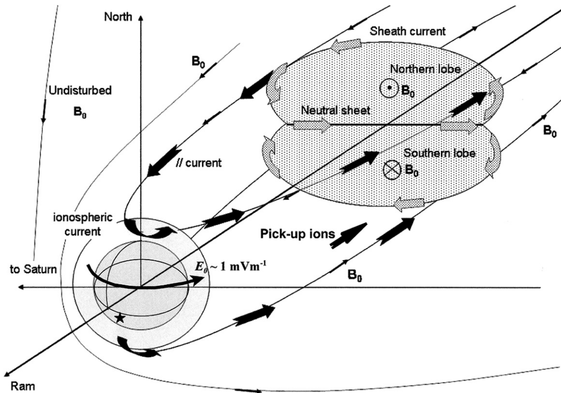
Fig. 7. Sketch of the wake interaction between Titan and Saturn's magnetosphere, and the induced driven current system (Huygens landing is site pointed out by a star).
