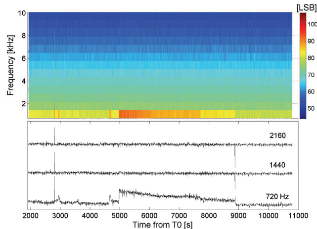
Figure 21: Electric signal measured with the PWA receivers in the VLF range below 60 km and on the surface. Top : Dynamic spectrum with frequency resolution of 360 Hz. The spectral levels are given by the colour scales shown on the right hand side in LSB units. Bottom : Spectral lines below 2.2 kHz shown in arbitrary units and shifted for better visualization. A significant amplitude increase is observed at about 5000 s and the spike at 8870 s corresponds to touchdown.
