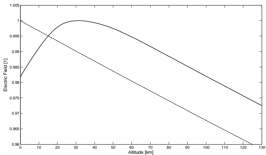
Figure 5: Electric field amplitude as a function of altitude in a lossless cavity with PEC boundaries, where R_{int}=R_v , R_{ext}=R_v+h , and h=130 km. The permittivity is given by the profile of Fig. 2 (solid line) or is assumed to be that of vacuum (dashed line). The electric field maximum is reached at 31.5 km.
