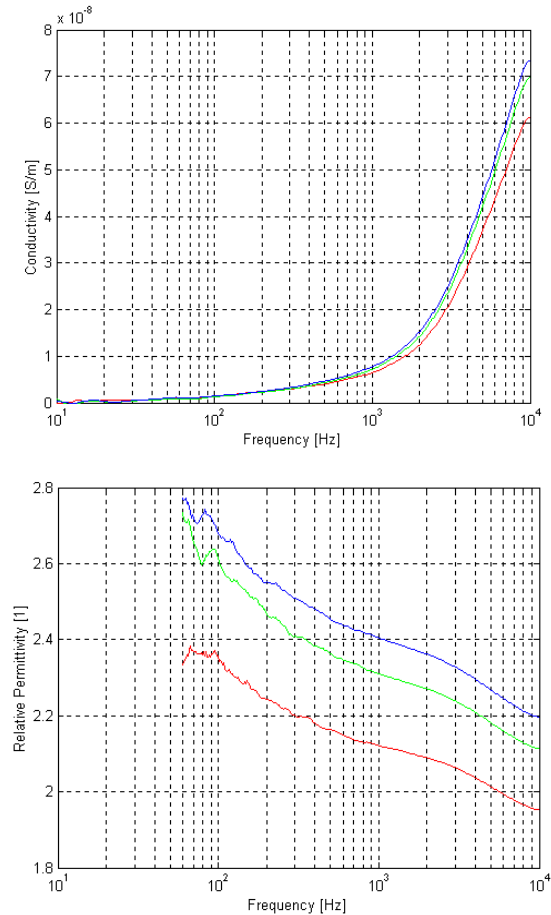
Fig. 2. Conductivity (top) and relative dielectric constant (bottom) of the dry JSC Mars-1 simulant ( \theta=0.005 ), at T=+20^\circ\text{C} , for different porosities: \phi=0.58 (red), \phi=0.54 (green), and \phi=0.52 (blue).
