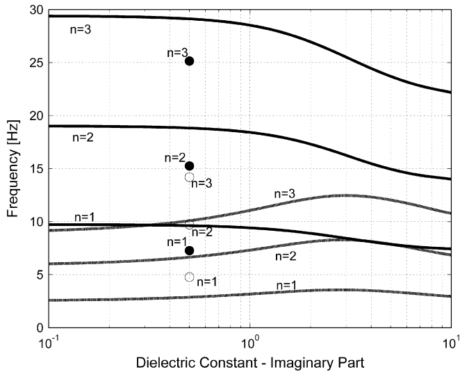
Fig. 5. Same caption as in Fig. 4, but \epsilon_{\text{soil}} = 3 , and the eigenfrequencies are plotted against the imaginary part of the soil dielectric constant.
