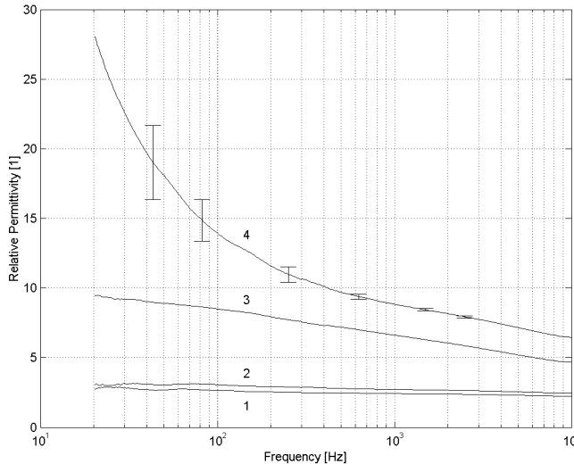
Figure 2. Relative dielectric constant of the JSC Mars-1 simulant as function of frequency, at \phi=0.54 , with different gravimetric water contents: \theta < 0.005 (1), \theta=0.01 (2), \theta=0.05 (3), and \theta=0.1 (4) for T=-25^{\circ}\text{C} .
