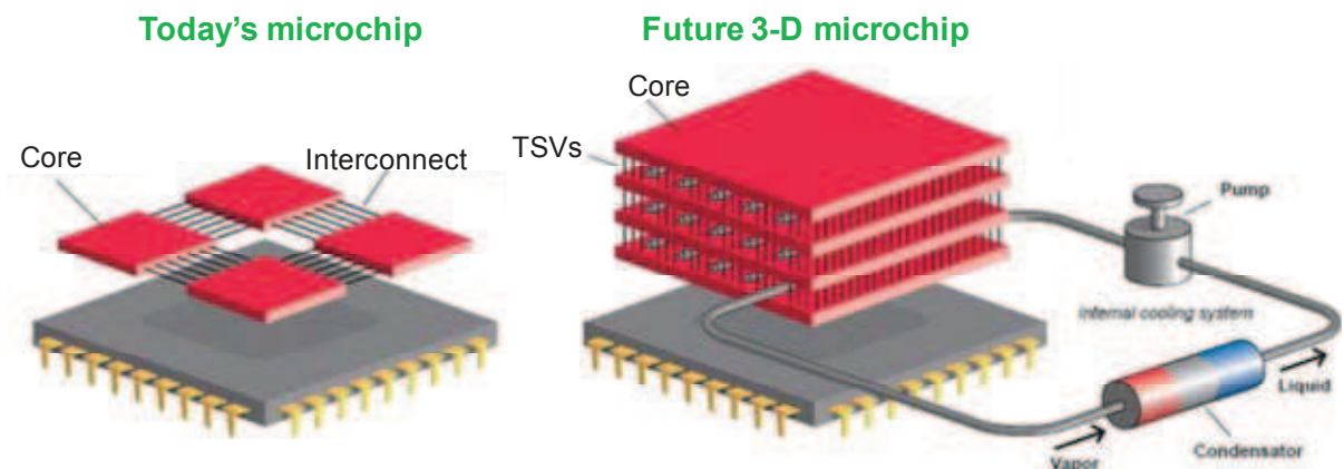
Fig. 2| Scheme presenting the difference between today's multicores technology and future developing architecture. Adapted from EPFL.LTCM, John R. Thome; infograph: Pascal Codéray.
