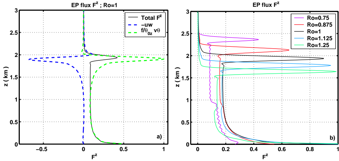
FIG. 3.7 – a) Vertical Eliassen-Palm (EP) flux F^z (black) and its two components \rho_0 \frac{f}{\theta_{0z}} \overline{v' \theta'} (green) and (-\rho_0 \overline{u' w'}) (blue) averaged in time in experiment. The profiles are normalized by the maximum of \rho_0 \frac{f}{\theta_{0z}} \overline{v' \theta'} . b) Vertical Eliassen-Palm (EP) flux F^z in experiment L but for different values of Ro . All the profiles are normalized by the maximum of F^z for Ro=1 , which is localized at the surface.
