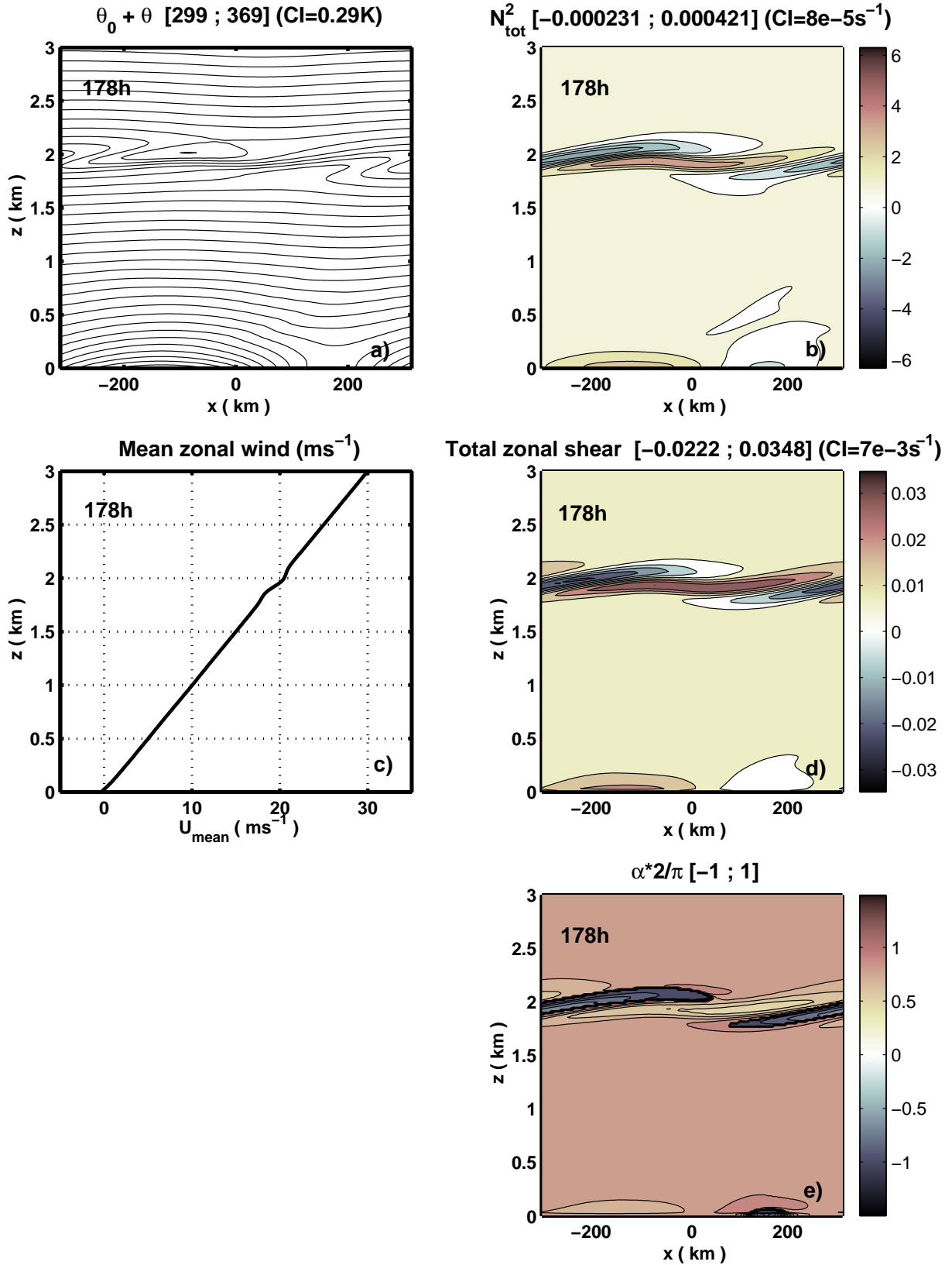
FIG. 3.14 – Stability diagnostics in experiment NL at t=178\text{h} : a) total potential temperature, b) total local Brunt-Väisälä constant, c) total horizontal mean zonal wind, d) total local zonal shear, and e) the image of the Richardson number \frac{2}{\pi} * \alpha = \arctan(4\text{Ri}) .
