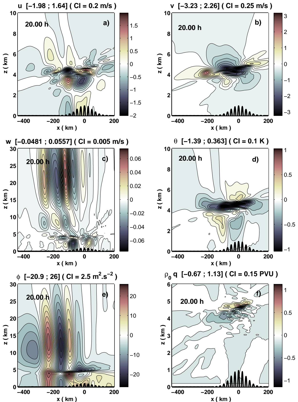
FIG. 4.28 – Total large scale response to the orography at t=20\text{h} for experiment M2 ( H_0 = 150\text{m} ): a) zonal velocity, b) meridional velocity, c) vertical velocity, d) potential temperature, e) geopotential perturbation and f) PV anomaly.
