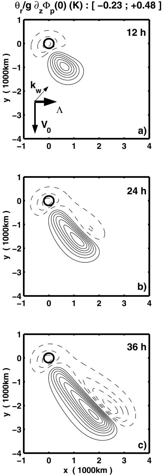
FIG. 6. Evolution of the potential temperature anomaly at the surface (\theta_r/g)\partial_z\phi_p(0) , same parameters as in Fig. 2; (a) t = 12 h, (b) t = 24 h, and (c) t = 36 h. Negative values are dashed and CI = 0.5 K.
