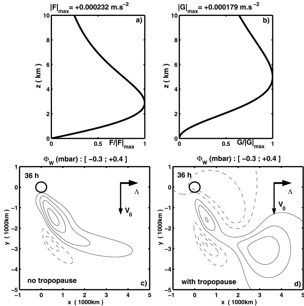
FIG. 14. Cold front simulations with an orographic spectrum representative of the Alps. (a) Vertical profile of \bar{F}(z) , (b) vertical profile of \bar{G}(z) , (c) \phi_w at t = 36 \text{ h} with no tropopause, and (d) \phi_w at t = 36 \text{ h} with tropopause at D = 10 \text{ km} . Negative values are dashed and \text{CI} = 0.1 \text{ mb} .
