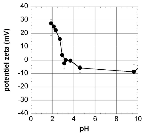
(c) Pyrolusite, \beta\text{-MnO}_2 .
