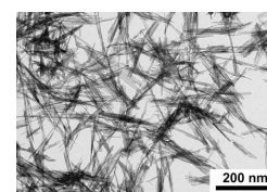
Groutite, \alpha\text{-MnOOH} . DRX: \blacklozenge . JCPDS no. 24-0713.
