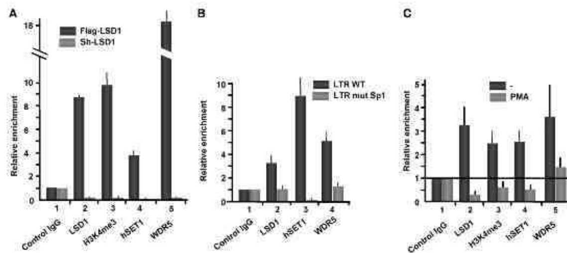
Figure 7. LSD1 favours hSET1 and WDR5 recruitment at the HIV-1 proximal promoter. (A) ChIP experiments were performed on HEK 293T cells transfected with the HIV-1 LTR-LUC reporter vector in the presence of the pFLAG-LSD1, the shRNA-LSD1 or the respective pcDNA3-FLAG and pcDNA3-control vectors. Cells were subjected to ChIP assays with the indicated antibodies. Specific enrichments were calculated relative to the control IgG and relative enrichments in the context of LSD1 over-expression or depletion were expressed relative to the value obtained with the pcDNA3-FLAG or the pcDNA3-control vectors, respectively. Specific enrichments in the HIV-1 proximal promoter region were quantified by real-time PCR. (B) HEK 293T cells were transfected with the pLTR-LUC (1 789) or with the pLTR-LUC (1 789) mut Sp1 vector 48 h before being subjected to ChIP experiments with the indicated antibodies. Input and immunoprecipitated DNAs were quantified by real-time PCR using primers targeting the Sp1-binding sites region of the HIV-1 promoter. The amounts of immunoprecipitated material were normalized to the input DNA and presented relative to the non specific control IgG. (C) Microglial cells were infected with the VSV-pseudotyped pNL4.3-Env virus 24 h before being subjected to ChIP experiments with the indicated antibodies. Specific enrichments in the HIV-1 proximal promoter were quantified by real-time PCR. Enrichments are presented relative to the non specific IgG values set at 1.
