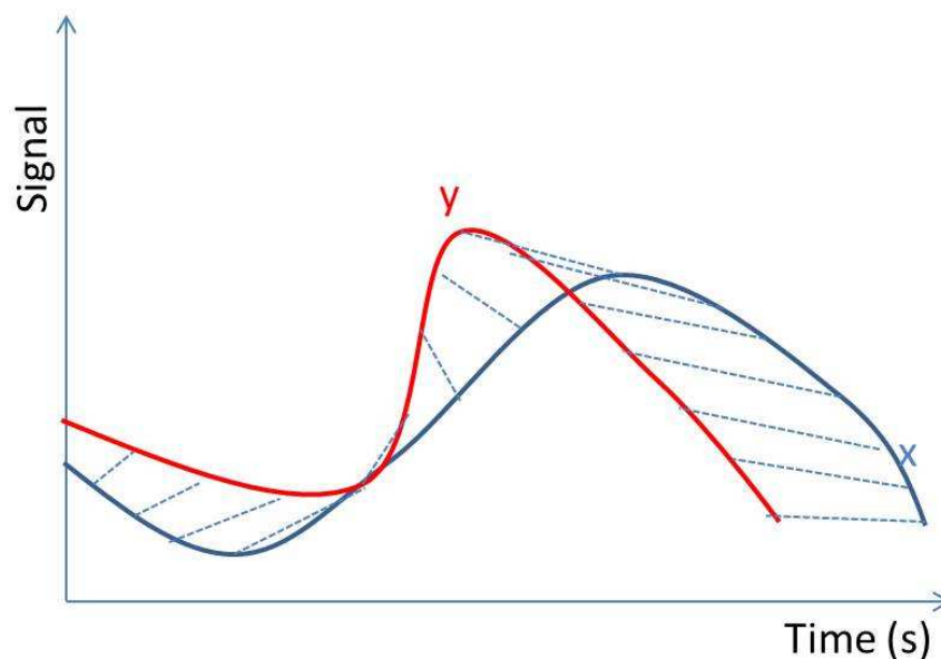
Figure 5.2 - Non-linear time alignment of two signals using Dynamic Time Warping.
