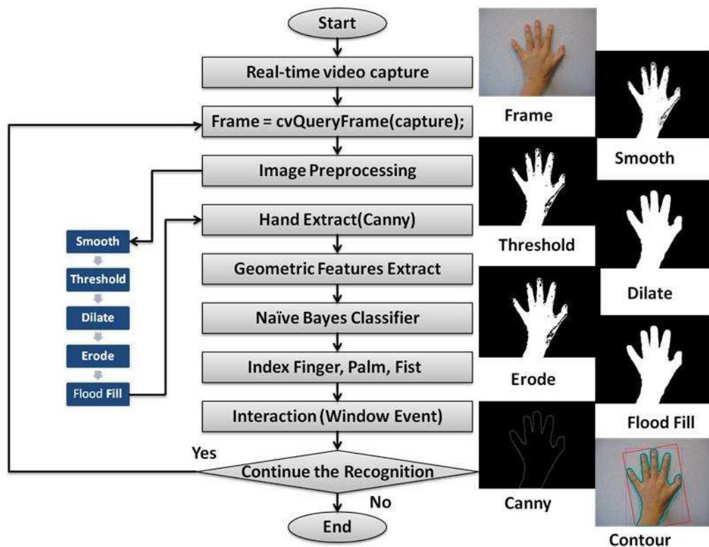
Figure 6.10 The recognition process of the fist-palm gesture.
