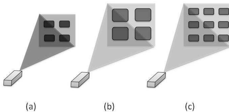
Figure 5.1 Multi-scale interfaces.
