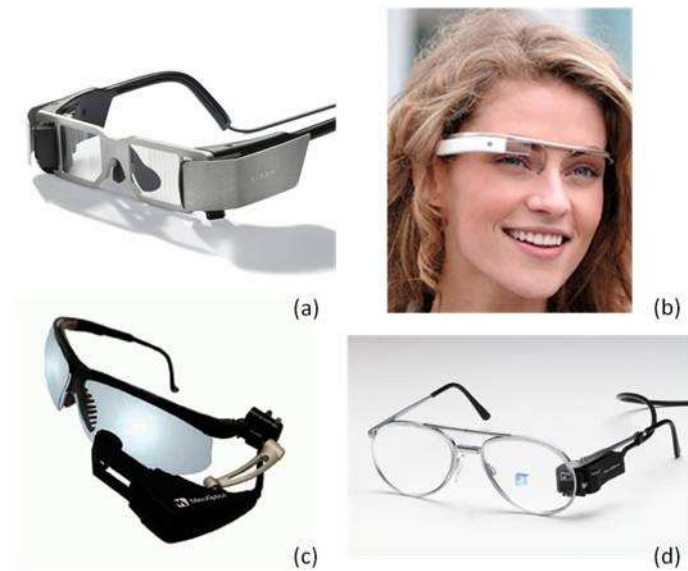
Figure 2.6 Head-worn displays.
