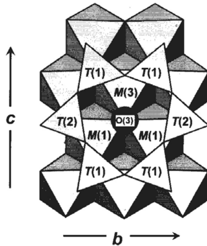
Figure 9 - The O(3) in the C 2/m amphiboles (from Hawthorne et al, 2007).
