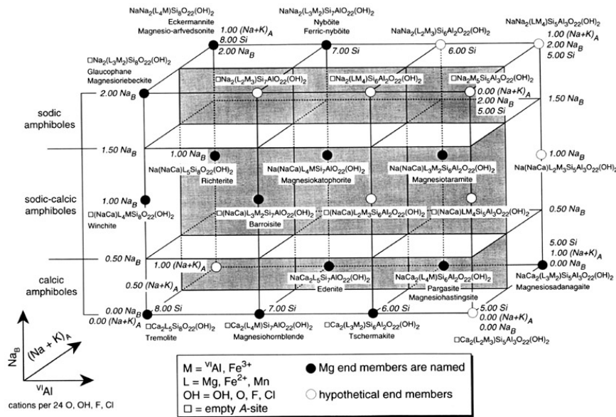
Figure 10 - General classification of the amphiboles, escluding the Mg-Fe-Mn-Li amphiboles (from Leake et al., 1997).
