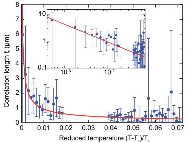
FIG. 3: Divergence of the correlation length \xi as a function of temperature. The red line is a fit of Eq 2 to the data with \nu and T_c as free parameters. Plotted is one data set for a specific temporal offset t_0 . The error bars are \pm SD, according to fits to Eq 1. They also reflect the scattering between different data sets. Inset: Double logarithmic plot of the same data.
