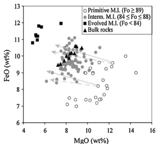
Fig. 4 FeO versus MgO concentrations for Aoba olivine-hosted melt inclusions and bulk rocks corrected for accumulation of olivine back to a Kd_{\text{Ol-Liq}}^{\text{Mg-Fe}2+} value of 0.3. Also shown are MELTS-calculated liquid lines of descent of primitive melt inclusions (Ao17–10 and Ao17–6; Table 2) at 2 kb (dotted arrow) and 5 kb (solid arrow). Oxide concentrations were recalculated on an anhydrous basis
