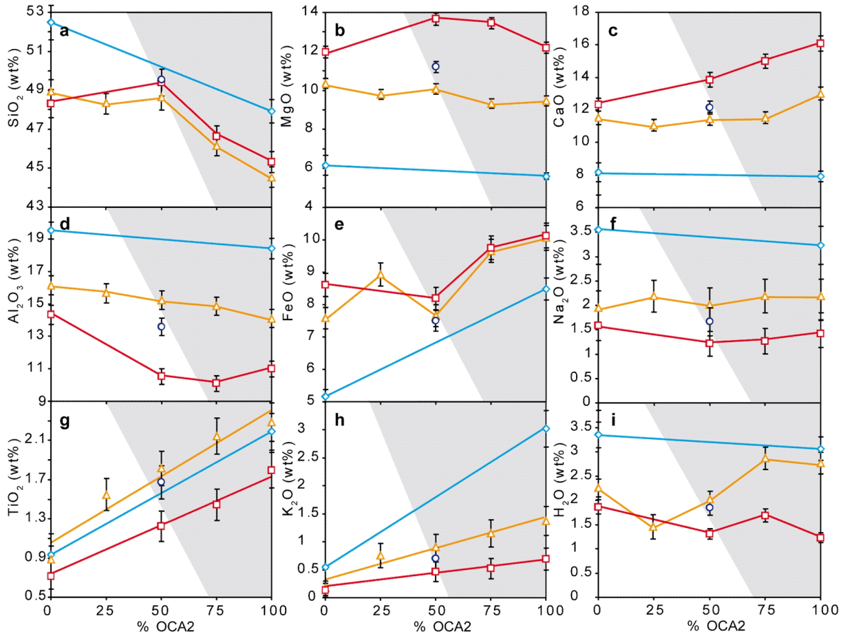
Figure 1: Compositions of experimental glasses (in wt%, with 2 \sigma error bars) as a function of the proportion of OCA2 in the starting materials at 1150°C (diamonds), 1200°C (triangles), 1250°C (circles) and 1300°C (squares). (a – e) Major elements; (f – h) minor elements; and (i) water. The grey and white fields overlap the samples without and with orthopyroxene, respectively.
