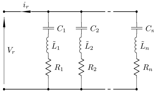
Figure 3.10: Example of a current flowing circuit with the actual value of the inductors.
