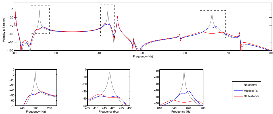
Figure 5.18: Simulated FRF Response of the plate velocity with different types of control
