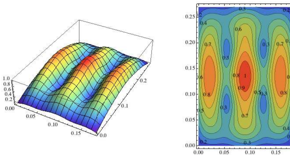
Figure 3.18: Acoustic controllability \tilde{\mathcal{A}}_{in} of a simply supported plate
