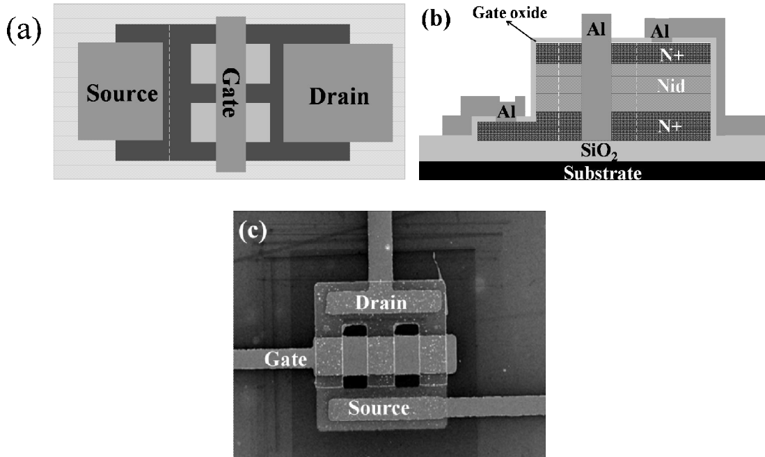
Figure 2-14: (a) Top view, (b) side view of the final VTFT after etching the deposited Al, and (c) SEM image of the fabricated three-tooth VTFT.
