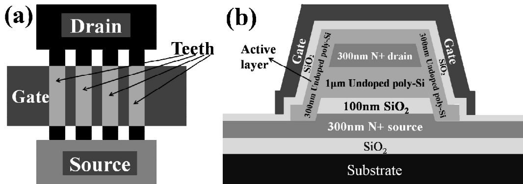
Figure 3-14: (a) The schematic top view of the new VTFT structure, (b) the schematic tooth structure for the new VTFT with a 100 nm \text{SiO}_2 insulating layer.
