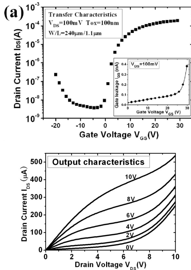
Figure 3-17: Electrical characteristics of the new VTFT involving a 100 nm \text{SiO}_2 barrier that limits the drain-source leakage current: (a) transfer characteristics, and (b) output characteristics.
