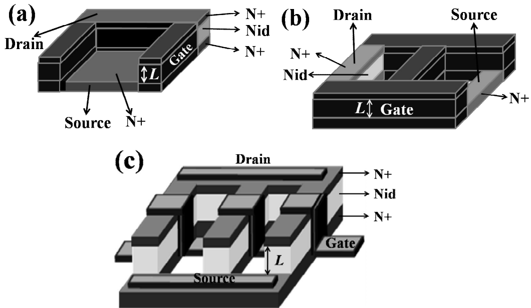
Figure 2-8: Schematic views of (a) the U-shaped VTFT, (b) the H-shaped VTFT, and (c) the comb-shaped VTFT.
