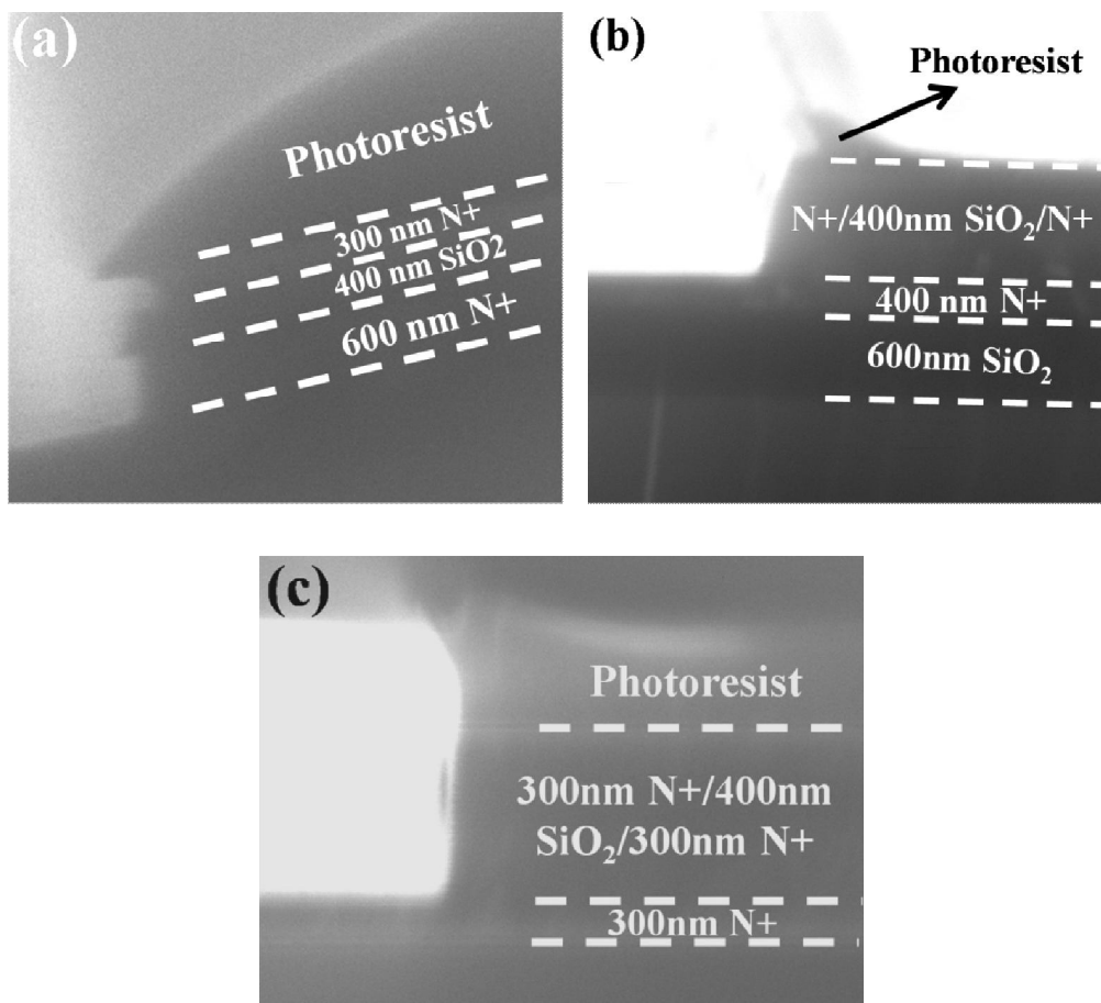
Figure 3-13: SEM images of different RIE tests for the poly-Si/400 nm SiO 2 /poly-Si sidewalls. (a) poly-Si layers are etched by SF 6 , SiO 2 layer is patterned by wet etching, (b) all layers are etched by CF 4 , and (c) the top poly-Si layer are etched by SF 6 , while SiO 2 and the bottom poly-Si layers are etched by CF 4 .
