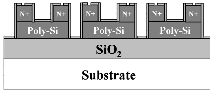
Figure 1-6: Gate oxide deposition and wet etching to make contact openings.
