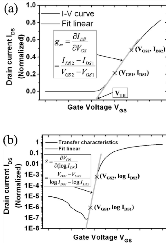
Figure 2-17: I_{DS}-V_{GS} curve (a) in the linear coordinate system, and (b) in the semi-logarithm coordinate system. The electrical parameters could be deduced from the two curves.
