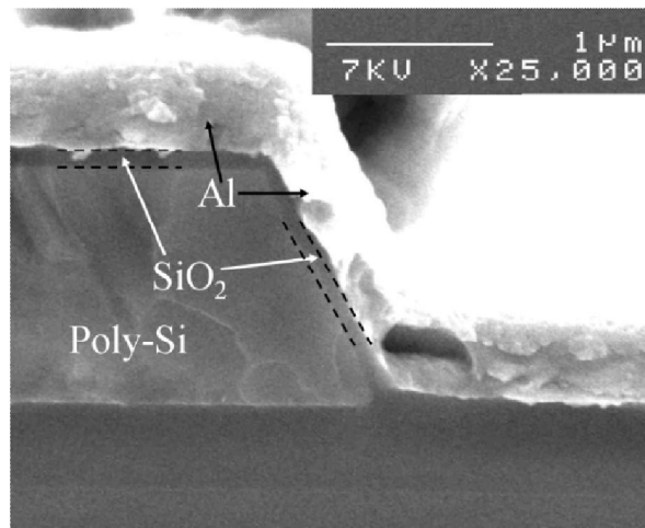
Figure 2-5: The conformal deposition of \text{SiO}_2 is shown, whereas the deposited aluminum shows a higher thickness on the planar surface than on the vertical sidewall.
