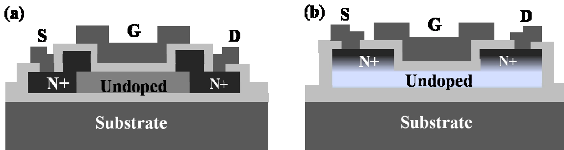
Figure 1-2: Schematic view of (a) a bilayer LTFT, and (b) a monolayer LTFT [24].
