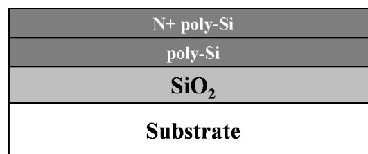
Figure 1-3: Schematic structure after the deposition of two poly-Si layers by LPCVD technique. “N+” stands for the N-type heavily-doped poly-Si layer, and “poly-Si” stands for the undoped poly-Si layer.
