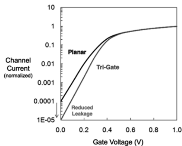
Figure 1-14: I - V measurement of Intel's 22 nm tri-gate FinFET in comparison with its 32 nm planar transistor [7].
