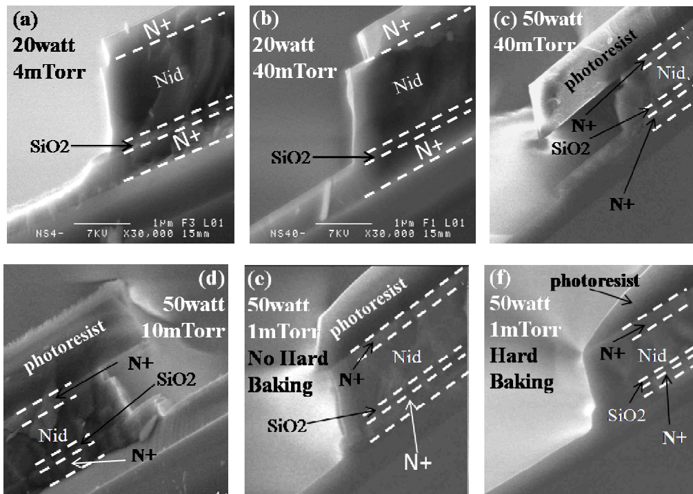
Figure 3-15: SEM image of the sidewalls by RIE under different etching conditions: (a) 20 watt, 4 mTorr, no photoresist is remained after etching, and (b) 20 watt, 40 mTorr, no photoresist is remained after etching. These two conditions cannot be applied for fabrication due to the overetching of photoresist. (c) 50 watt, 40 mTorr, photoresist without hard baking, and (d) 50 watt, 10 mTorr, photoresist without hard baking. These two conditions cannot be applied for fabrication due to the large overetching of the sidewall. (e) 50 watt, 1 mTorr without hard baking, and (f) 50 watt, 1 mTorr with hard baking. These two conditions show better sidewalls, while the sidewall is more linear after hard baking of the photoresist. The \text{SF}_6 gas flow is always set to be 10 sccm.
