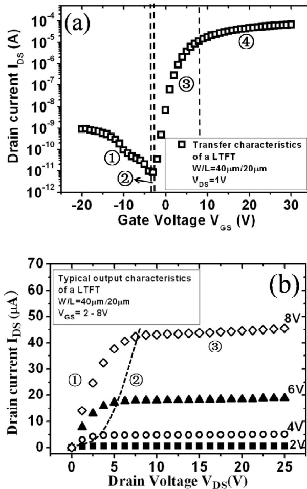
Figure 1-11: (a) Typical Transfer characteristics, and (b) output characteristics of the LTFT fabricated in our laboratory [28].
