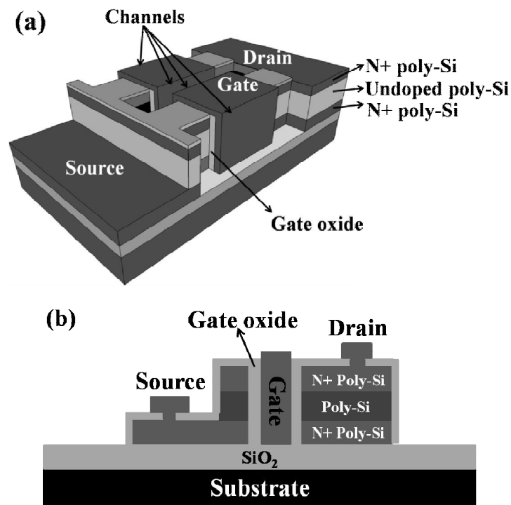
Figure 1-24: (a) 3D view, and (b) side view of the multi-gate VTFT.
