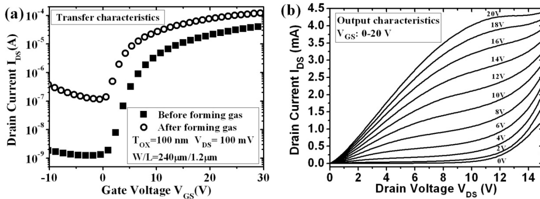
Figure 3-25: (a) Transfer characteristics before and after forming gas, an I_{ON}/I_{OFF} ratio of almost 10^5 is shown before the forming gas treatment, and (b) output characteristics of the new VTFT structure, better saturation is obtained.
