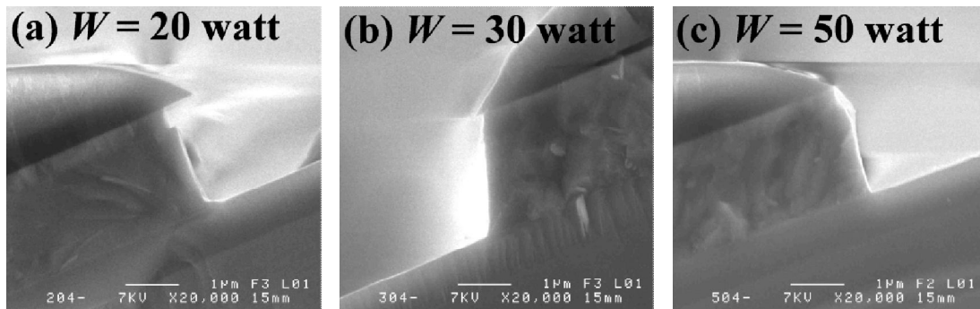
Figure 2-15: SEM images of sidewalls etched by different powers W : (a) W = 20 watt, (b) W = 30 watt, (c) W = 50 watt, pressure P = 4 mTorr, gas flow \Gamma = 10 sccm.
