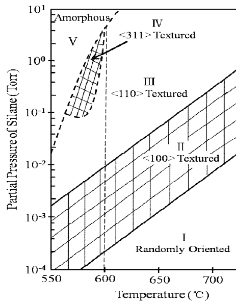
Figure 2-4: Silicon structure deposited by LPCVD under different deposition temperatures and partial pressures of \text{SiH}_4 precursor gas [85]. At 550^\circ\text{C} and 90\text{ Pa} ( 0.675\text{ Torr} ), the silicon is in amorphous state (V zone), while at 600^\circ\text{C} and 90\text{ Pa} ( 0.675\text{ Torr} ), the silicon is poly-Si (III \langle 110 \rangle Textured zone).
