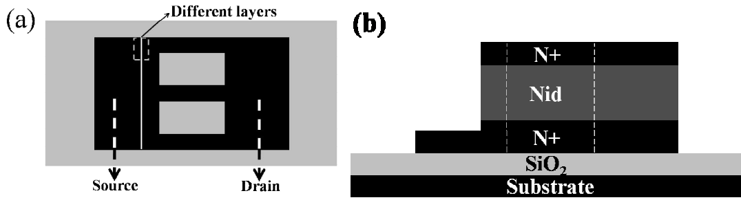
Figure 2-12: (a) Top view, and (b) side view of the VTFT configuration after the second RIE.
