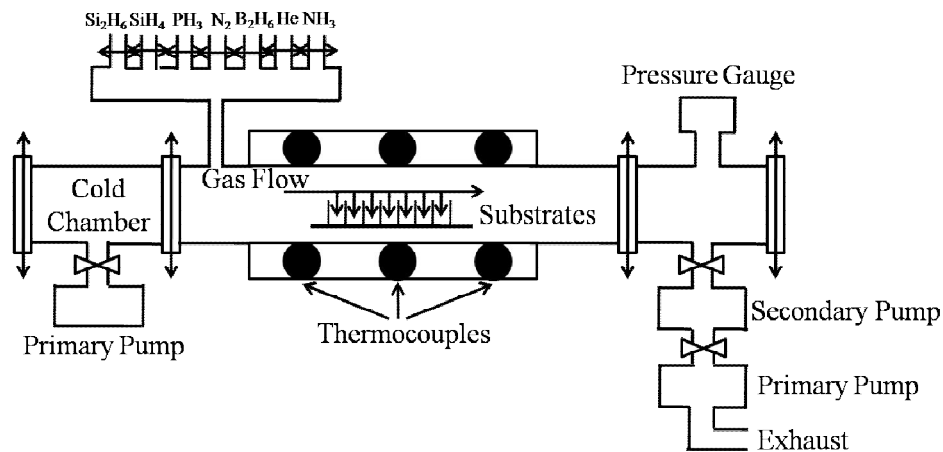
Figure 2-3: Schematic view of a typical horizontal LPCVD system.
