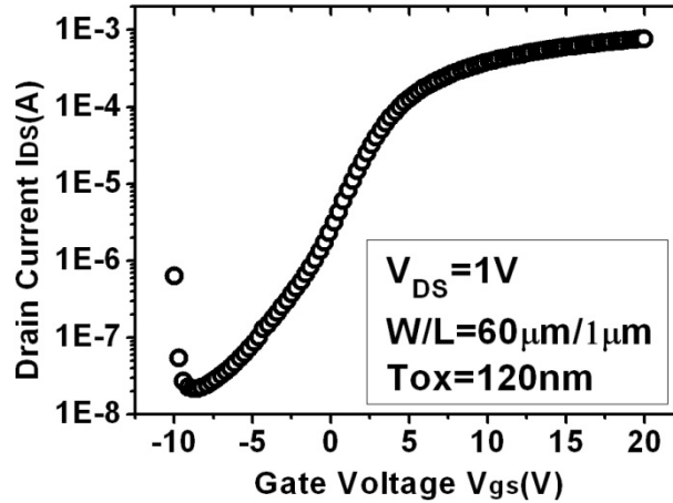
Figure 2-28: Transfer characteristics of the classical VTFT structure after the reduction of the large overlapping area, the off-current reduces that leads to an I_{ON}/I_{OFF} ratio of almost 10^5 .
