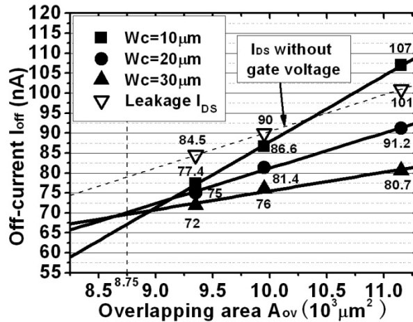
Figure 2-27: Comparison between the drain-source current I_{DS} (without gate voltage) and the off-current I_{OFF} (with gate voltage), the gate voltage helps to suppress the drain current to some degree.
