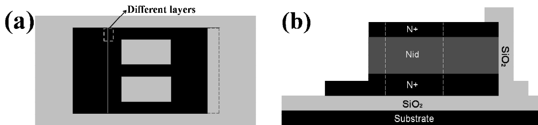
Figure 2-20: (a) The top view, and (b) the side view of the improved structure for the classical VTFT, a 500nm oxide layer is deposited at the backside of the top electrode, which helps to suppress the parasitic channel after electrodes formation.
