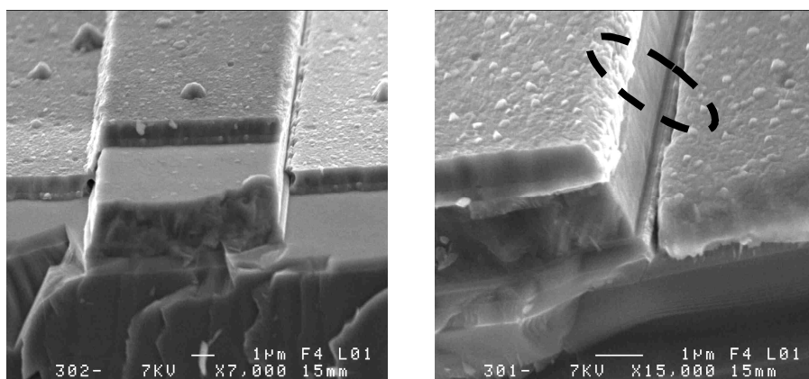
Figure 3-21: (a) Al deposition on the two sidewalls, the left sidewall has a good Al coverage, while the right sidewall shows no Al deposited on the sidewall, (b) the enlarged image of the right sidewall, and “shadow effect” is obviously shown.
