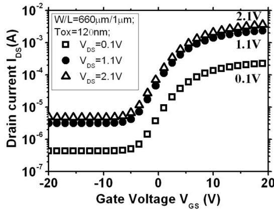
Figure 2-18: Typical transfer characteristics of the first classical VTFT, the high off-current I_{OFF} is due to the large overlapping area and short channel length L .
