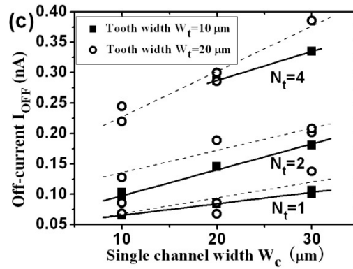
Figure 3-36: The relationship between the off-current I_{OFF} and the geometric parameters: (a) I_{OFF} is proportional to the teeth number N_t , (b) I_{OFF} is proportional to the single channel width W_c , and (c) I_{OFF} increases a little with the tooth width W_t .
