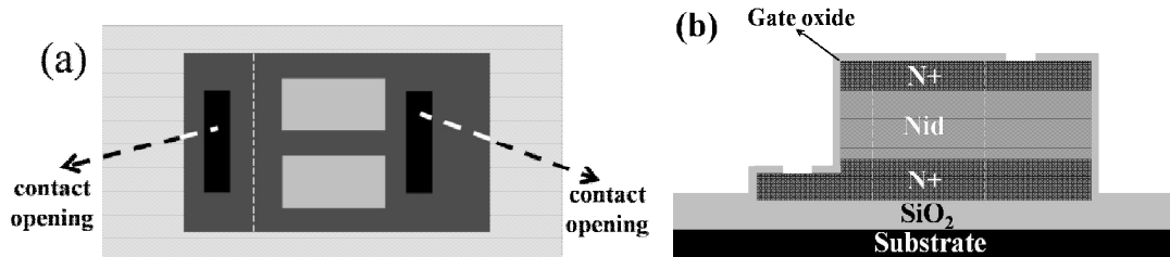
Figure 2-13: (a) Top view, and (b) side view of the VTFT configuration after the gate oxide deposition and making contact openings.
