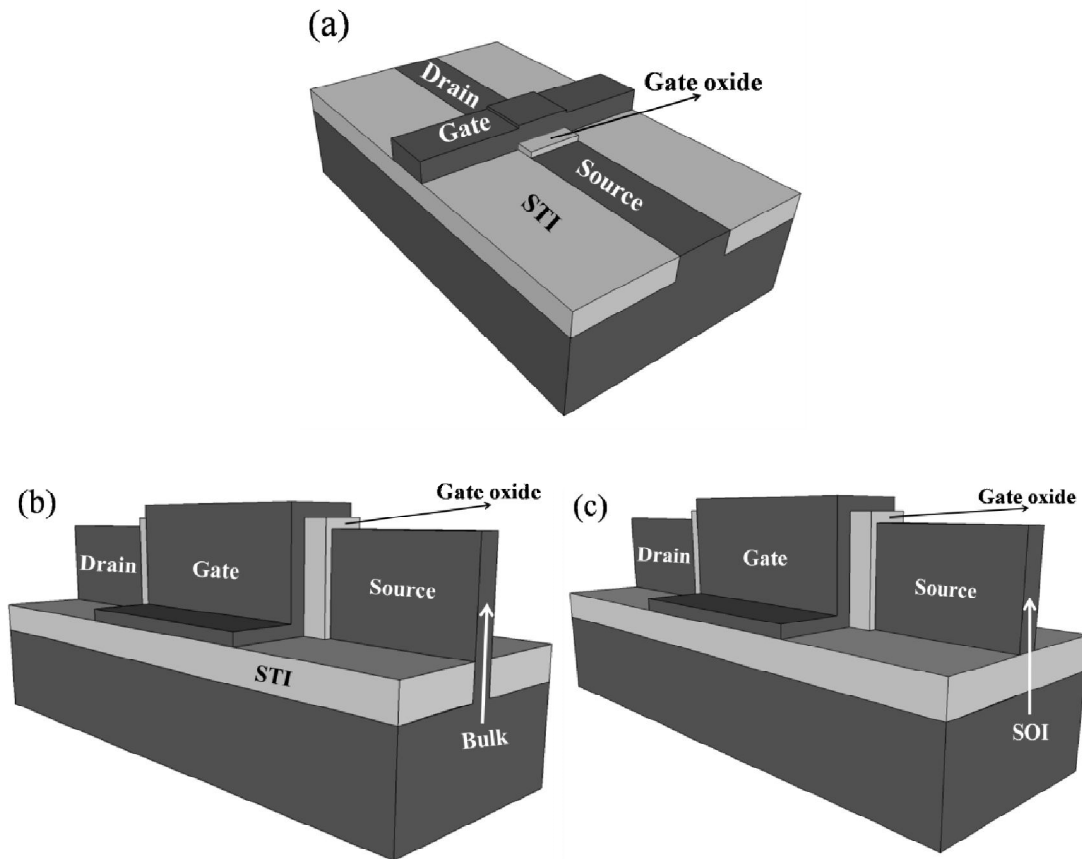
Figure 1-12: Schematic structure of (a) a planar FET, (b) a bulk FinFET, and (c) a SOI FinFET.
