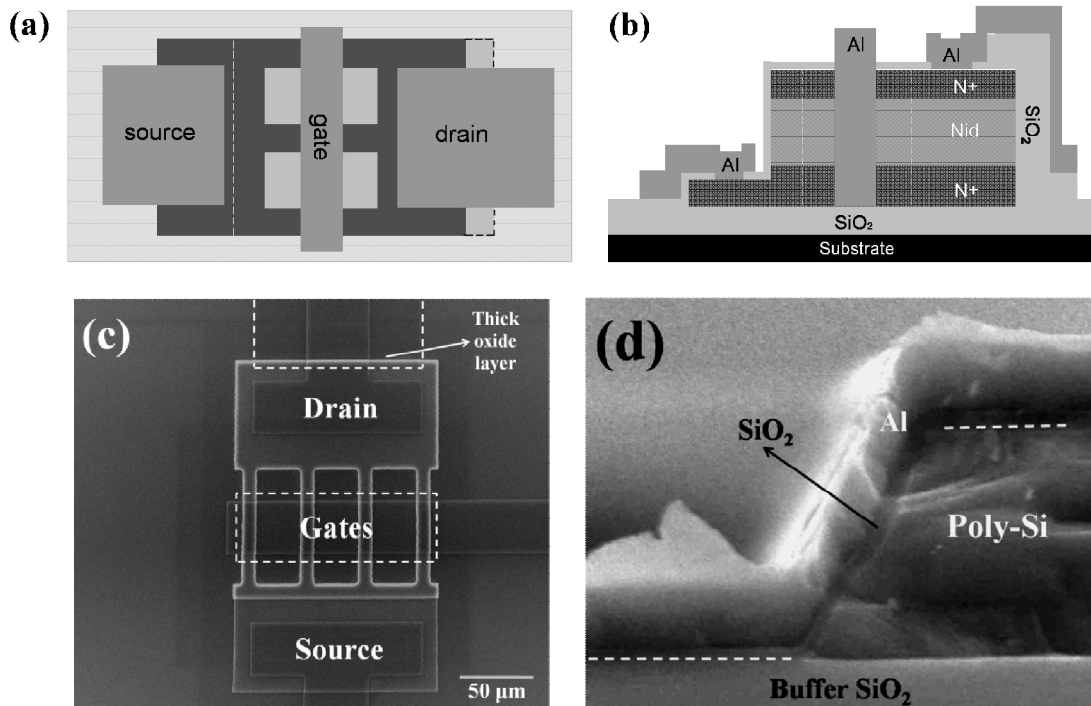
Figure 2-21: (a) The schematic top view, (b) the schematic side view, (c) the SEM image of the improved four-tooth VTFT configuration, the 500 nm thick oxide layer at the backside of the top electrode (signed as drain) enables to suppress the parasitic channel, and (d) the SEM image of the sidewall after the gate oxide and Al layers' deposition, the conformal \text{SiO}_2 layer and the continuous Al layer on the sidewall are observed.
