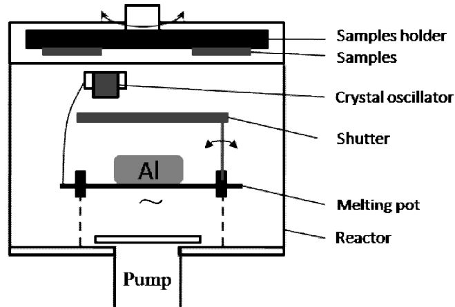
Figure 2-6: Schematic view of Joule effect evaporation for Al deposition.
