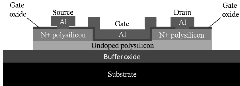
Figure 1-8: Schematic view of the N-type normally-off LTFT.
