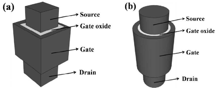
Figure 1-20: Schematic view of the 3D Gate-all-around (GAA) vertical MOSFET, (a) the common GAA vertical FET, and (b) the SiNW-based GAA vertical FET.
