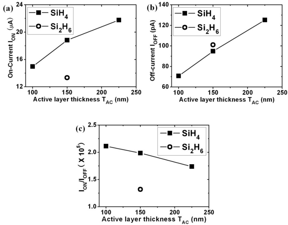
Figure 3-30: (a) On-current I_{ON} , (b) off-current I_{OFF} , and (c) I_{ON}/I_{OFF} relationships with different active layers.
