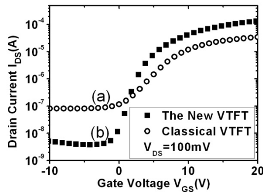
Figure 3-18: Typical transfer characteristics of the classical stacking structure ((a) without an oxide barrier) and the new structure ((b) with an oxide barrier). The first result shows a reduced off-current I_{OFF} and an increased I_{ON}/I_{OFF} ratio.
