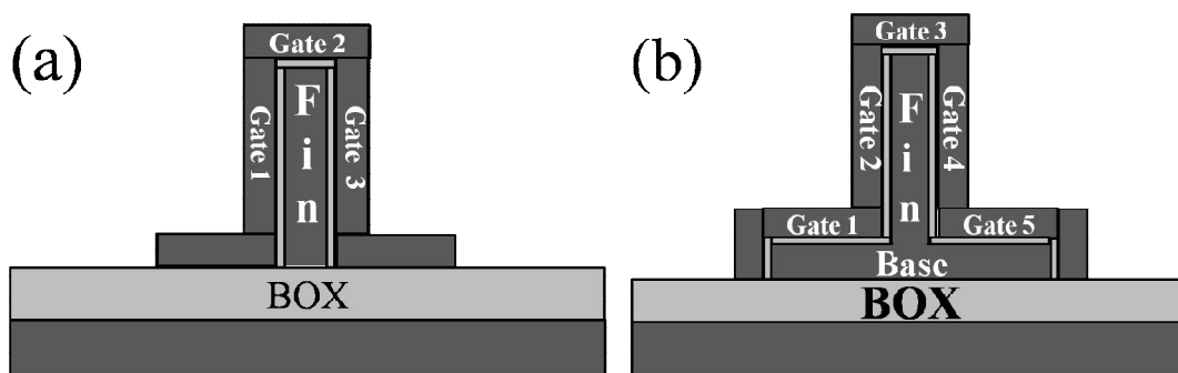
Figure 1-15: cross-section view of the gate part for (a) the SOI FinFET, and (b) the inverted-T channel FET (ITFET).
