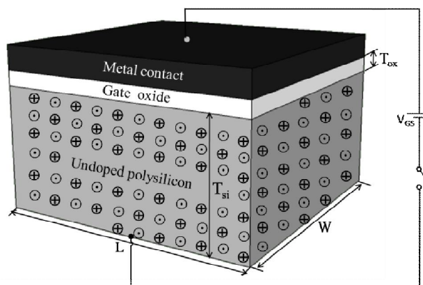
Figure 1-9: The MOS structure of a LTFT, the geometric parameters are shown. No channel is formed, thus the LTFT is at the off-state.
