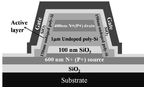
Figure 3-31: Schematic view of a basic tooth for the N(P)-type VTFT, a 100 nm SiO 2 insulating layer is adopted, the top and bottom heavily-doped layers are 400 nm and 600 nm, respectively, the active layer thickness T_{AC} is 150 nm, while the gate oxide thickness T_{OX} is 70 nm.
