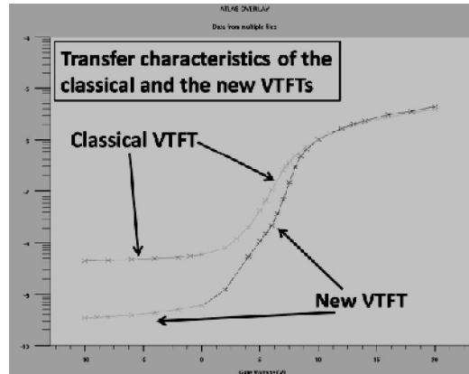
Figure 3-3: Simulated transfer characteristics comparison between the classical and the new VTFTs. The off-current I_{OFF} has been reduced by the barrier layer.
