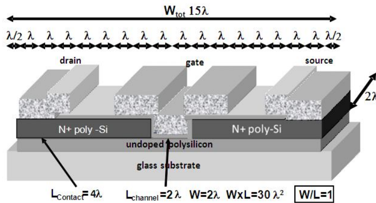
Figure 1-22: Schematic cross-sectional view of a LTFT, the device dimension is 15\lambda \times 2\lambda , while channel width and channel length ratio W/L = 2\lambda/2\lambda = 1 .
