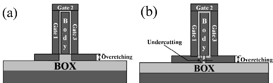
Figure 1-16: Schematic structures of (a) Pi-gate FET, and (b) Omega-gate FET.
