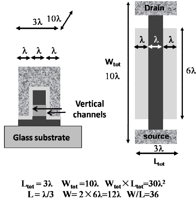
Figure 1-23: Schematic cross-sectional and top view of a VTFT, the device dimension is 3\lambda \times 10\lambda , while channel width and channel length ratio W/L = 12\lambda/(\lambda/3) = 36 .
