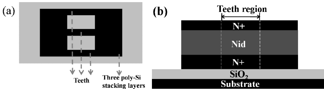
Figure 2-11: (a) Top view, and (b) side view of the comb-shaped VTFT configuration after the first RIE step.
