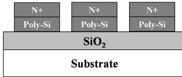
Figure 1-4: The first RIE step to form the poly-Si islands, whose dimensions would determine the sizes of the LTFTs.
