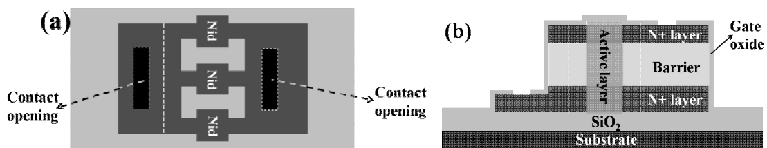
Figure 3-10: (a) Top view, and (b) side view of the new VTFT after gate oxide deposition and contact openings.
