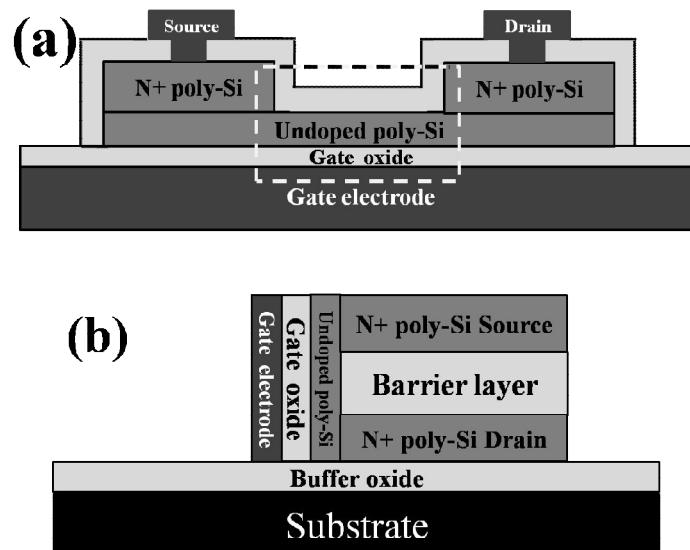
Figure 3-5: Schematic view of (a) the back-gate LTFT structure, and (b) the new VTFT structure. The new VTFT could be seen as rotating the back-gate LTFT 90°.
