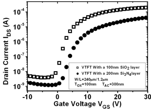
Figure 3-26: Transfer characteristics comparison between the new VTFTs with different insulating layers.
