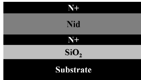
Figure 2-10: The deposited layers for the classical VTFT. The buffer \text{SiO}_2 is deposited by APCVD, while the three poly-Si layers are deposited by LPCVD technique, “N+” stands for the N-type heavily-doped poly-Si layer, while “Nid” stands for the undoped poly-Si layer.
