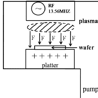
Figure 2-7: Schematic diagram of the RIE reactor, the plasma is generated by RF generator under a low pressure.
