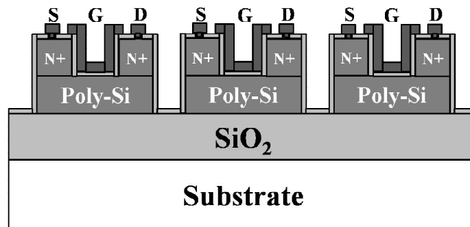
Figure 1-7: Schematic structure of the final LTFTs, the deposited Al is etched and the contacts are formed.
