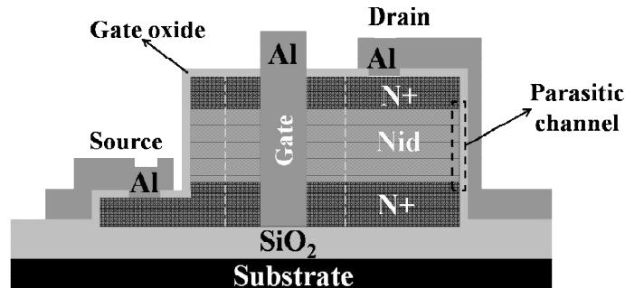
Figure 2-19: Schematic side view of the classical VTFT, the parasitic channel is observed at the backside of the top electrode.
