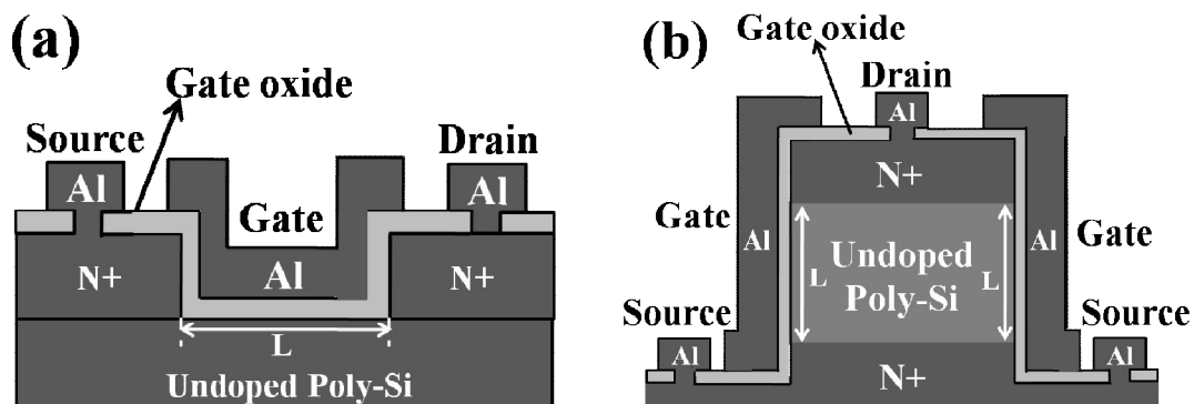
Figure 1-21: Schematic view of (a) the N-type LTFT, and (b) the N-type VTFT, the two types of TFTs are compatible with the classical CMOS technology.
