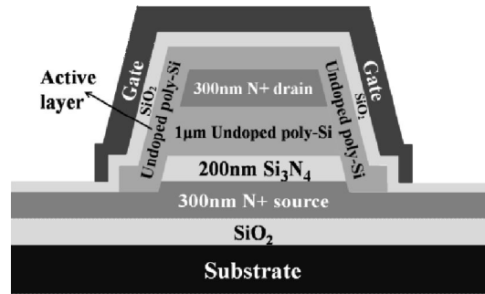
Figure 3-22: Schematic tooth structure for the new VTFT with a 200 nm \text{Si}_3\text{N}_4 insulating layer.
