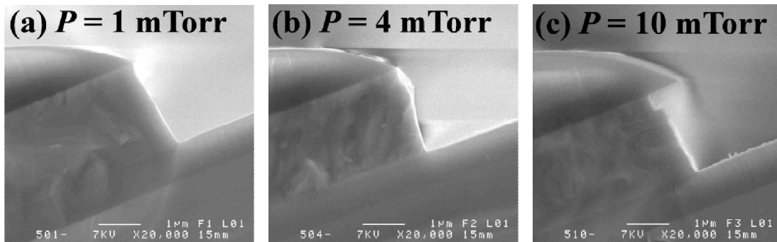
Figure 2-16: SEM images of sidewalls etched by different pressures P : (a) P = 1 mTorr, (b) P = 4 mTorr, (c) P = 10 mTorr, power W = 50 watt, gas flow \Gamma = 10 sccm.
