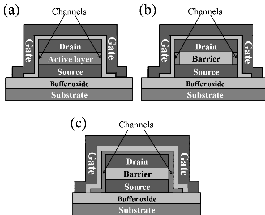
Figure 3-1: Schematic view of the tooth structure for (a) the classical VTFT, and (b) the improved classical VTFT, and (c) the new VTFT.
