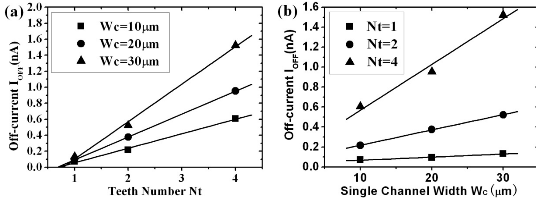
Figure 3-28: (a) Off-current I_{OFF} relationship with teeth number N_t , and (b) Off-current I_{OFF} relationship with single channel width W_c .
