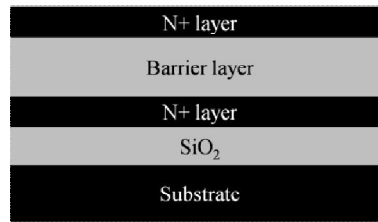
Figure 3-6: The deposition layers for the new VTFT, there is a barrier layer between two heavily-doped poly-Si layers deposited by LPCVD technique.
