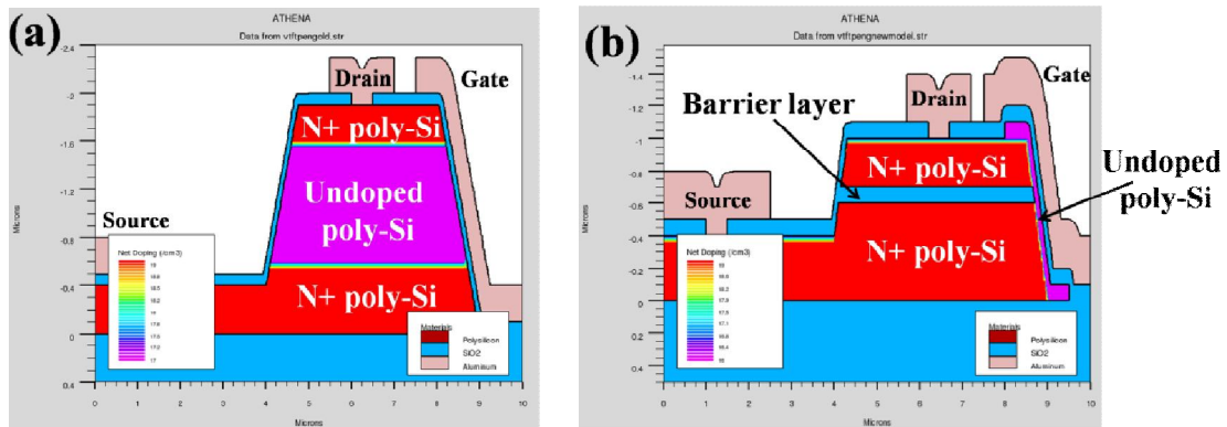
Figure 3-2: Simulated structure of (a) the classical VTFT, and (b) the new VTFT. The classical VTFT shows a large overlapping area between source and drain, while for the new VTFT, the overlapping area is suppressed by the barrier layer. “N+ poly-Si” stands for the N-type heavily-doped poly-Si.
