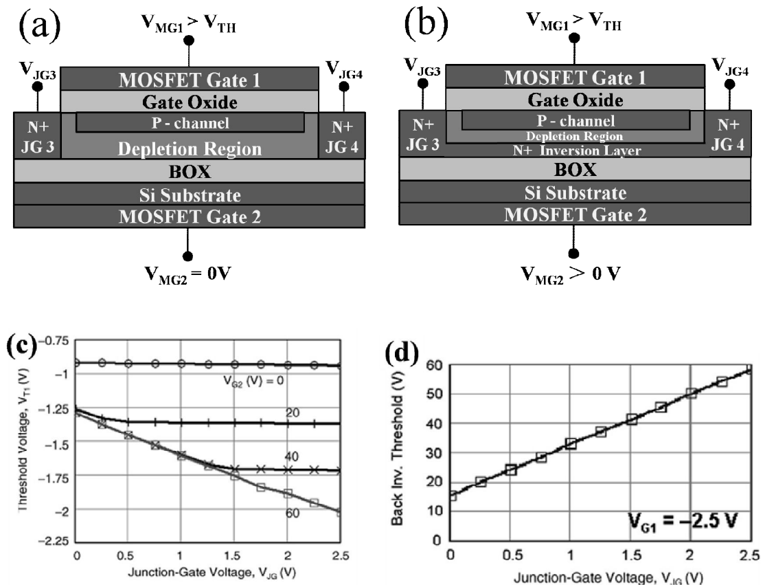
Figure 1-18: The schematic view of four-gate FET (a) with the top gate working, (b) with the double gate working, (c) the top gate threshold voltage V_{T1} and (d) the back gate threshold voltage V_{T2} modulated by different junction-gate voltages V_{JG} .
