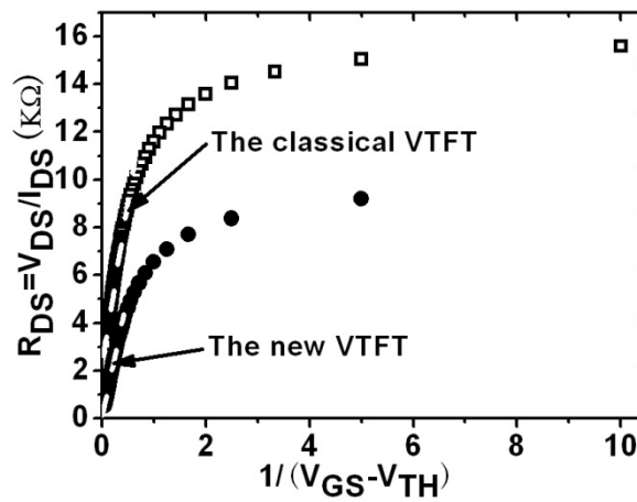
Figure 3-20: The relationship of R_{DS} and the 1/(V_{GS} - V_{TH}) , the access resistances R_{ACC} and the mobilities \mu'_{FE} could be extracted.
