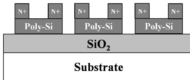
Figure 1-5: The second RIE is carried out to form source and drain of the LTFTs.
