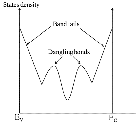
Figure 2-2: Schematic model of poly-Si energy states distribution.
