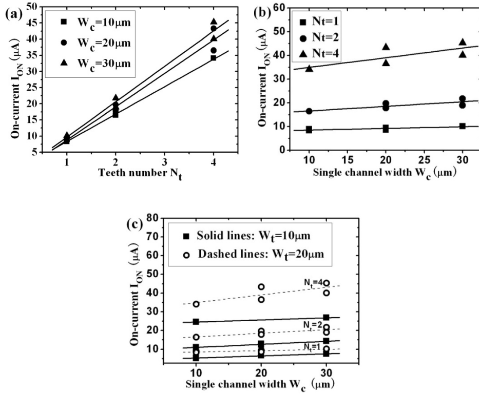
Figure 3-35: The relationship between the on-current I_{ON} and the geometric parameters: (a) I_{ON} is in proportion to the teeth number N_t , (b) I_{ON} is independent of the single channel width W_c , and (c) I_{ON} increases a little with the tooth width W_t .
