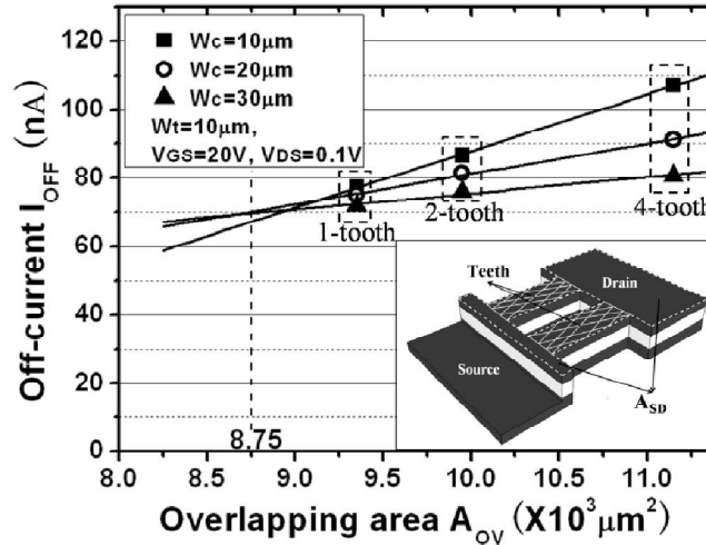
Figure 2-25: The relationship between the off-current I_{OFF} and the total overlapping area A_{OV} : I_{OFF} is proportional to A_{OV} . For the same teeth number N_t , the off-current I_{OFF} is also reduced by the increase of the single channel width W_c . The inset shows the schematic of the classical VTFT structure, the total overlapping area A_{OV} is marked with the dashed lines.
