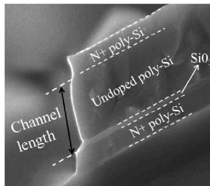
Figure 3-16: SEM image of the sidewall of the tooth after RIE.
