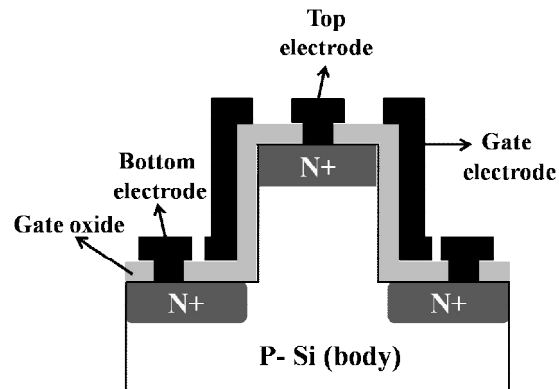
Figure 1-19: Schematic view of a vertical MOSFET.
