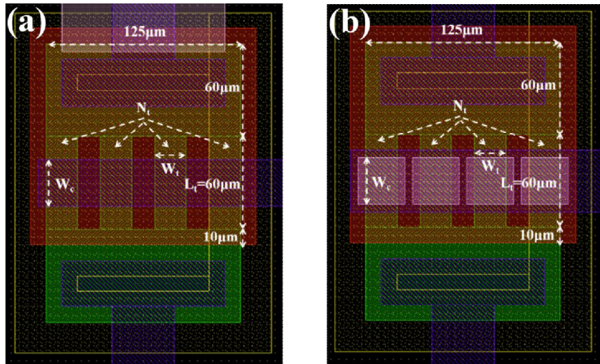
Figure III-1: Masks designs for (a) classical VTFT structure, and (b) the new VTFT structure.
