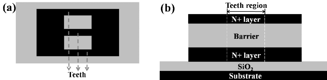
Figure 3-7: (a) Top view, and (b) side view of the new VTFT after the first RIE, the geometric dimension of the new VTFT is defined.
