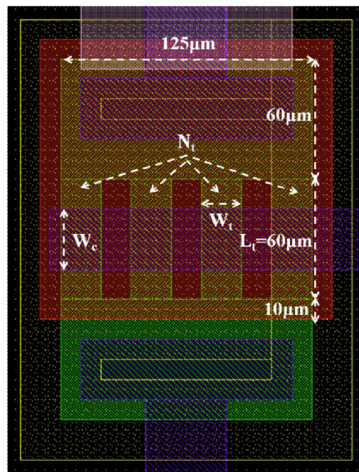
Figure 2-22: The five-mask design of a four-tooth classical VTFT, different geometric parameters are marked in the figure.
