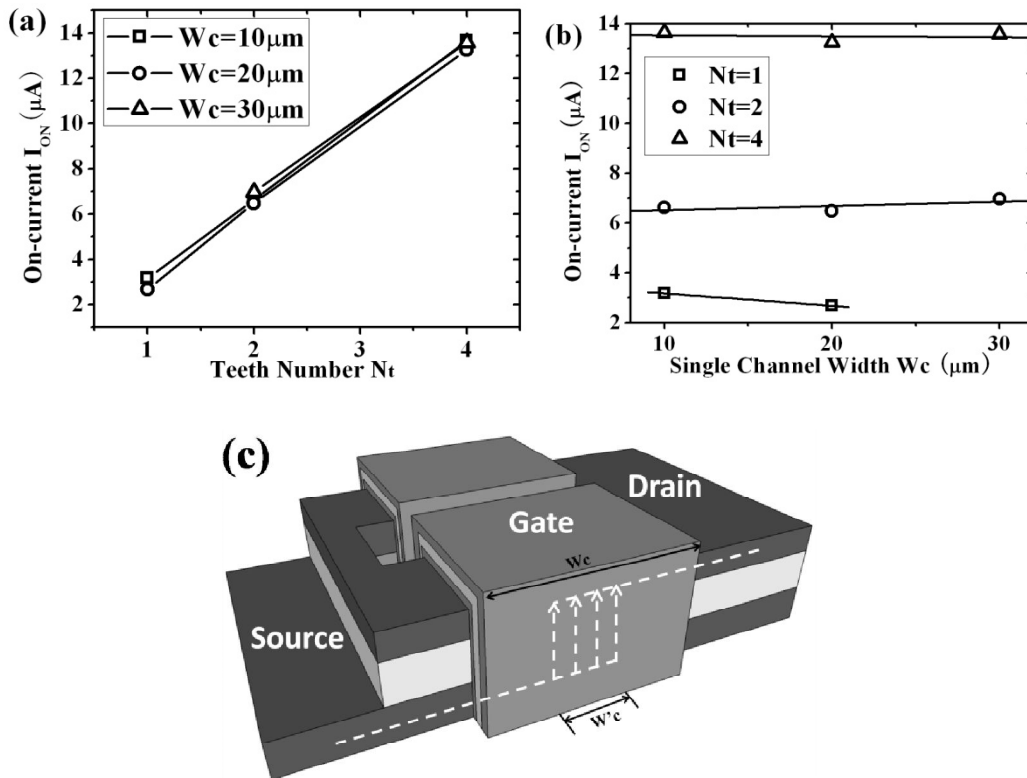
Figure 3-27: On-current I_{ON} relationship with (a) teeth number N_t , (b) single channel width W_c . The on-current is proportional to N_t , while it is independent of W_c , and (c) the efficient current path for the new VTFT, where the efficient single channel width W'_c is marked.
