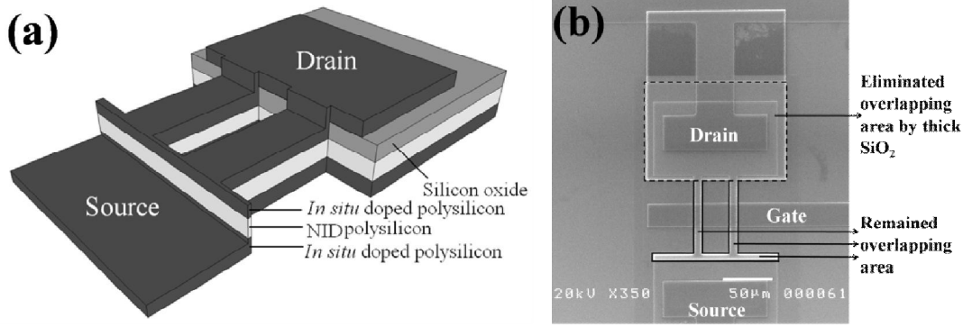
Figure 2-26: (a) Three-dimensional, and (b) SEM images of the two-tooth classical VTFT after the overlapping area reduction, the reduction is mainly obtained by the introduction of a thick oxide layer at the drain side.
