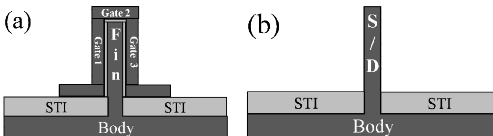
Figure 1-13: cross-sectional schematic view of the FinFET: (a) gate part, and (b) source/ drain part.
