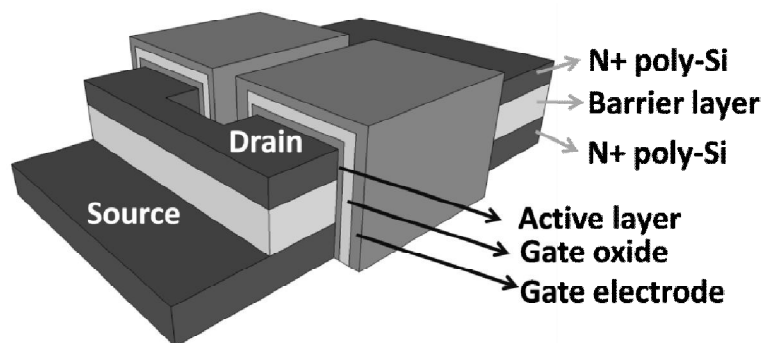
Figure 3-4: Three-dimensional view of the new VTFT structure, “N+ poly-Si” stands for the N-type heavily-doped poly-Si layer.
