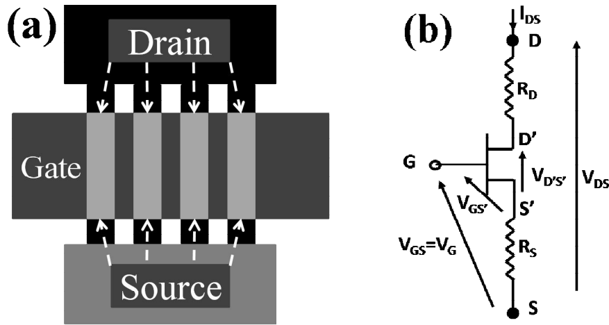
Figure 3-19: (a) The top view of a VTFT, where the access resistance R_{ACC} is shown as the dashed arrows, and (b) the schematic circuit diagram of a basic TFT.
