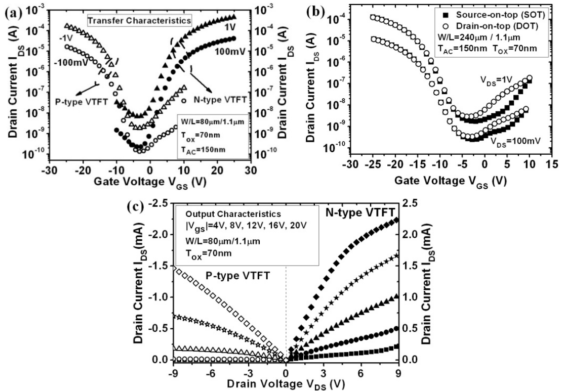
Figure 3-32: (a) Transfer characteristics of the P and N-type VTFTs, (b) transfer characteristics for source-on-top (SOT) and drain-on-top (DOT) structure, and (c) output characteristics of the P and N-type VTFTs.
