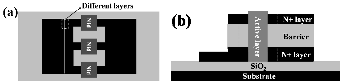
Figure 3-9: (a) Top view, and (b) side view of the new VTFT after the third RIE of the deposited active layer, which enables to form the channels on the sidewalls, “Nid” stands for the undoped (non-intentionally doped) poly-Si active layer.
