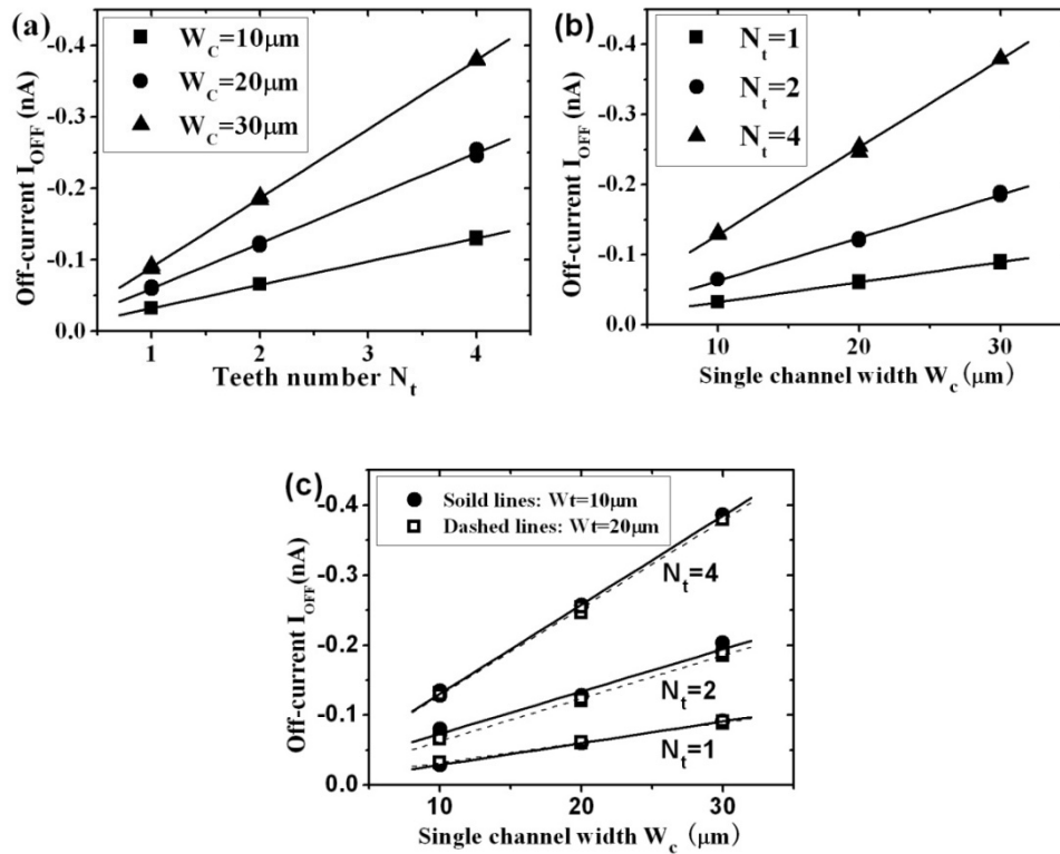
Figure 3-34: The relationships of I_{OFF} with different geometric parameters: (a) I_{OFF} is proportional to the teeth number N_t , (b) I_{OFF} is in proportion to the single channel width W_c , and (c) I_{OFF} is independent of the tooth width W_t .
