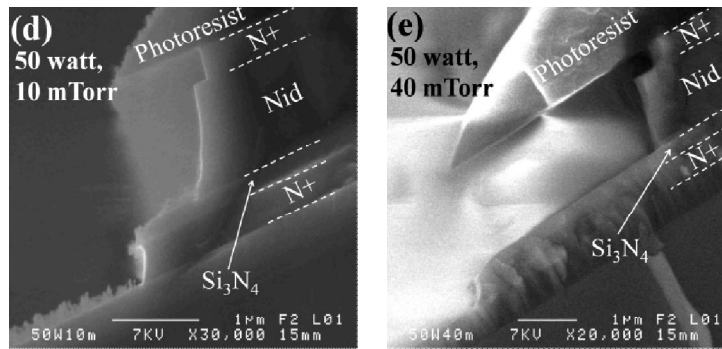
Figure 3-23: SEM image of the sidewalls by RIE under different etching conditions: (a) 30 watt, 10 mTorr; (b) 50 watt, 1 mTorr; (c) 50 watt, 4 mTorr; (d) 50 watt, 10 mTorr; (e) 50 watt 40 mTorr. For the conditions of (a), (d), (e), they cannot be applied for the VTFTs fabrication due to the large lateral overetching. For the conditions of (b) and (c), the former shows a much better sidewall. The \text{SF}_6 gas flow is always set to be 10 sccm.
