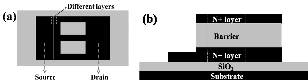
Figure 3-8: (a) Top view, and (b) side view of the new VTFT after the partial etching by the second RIE, source and drain regions could be accessed to.
