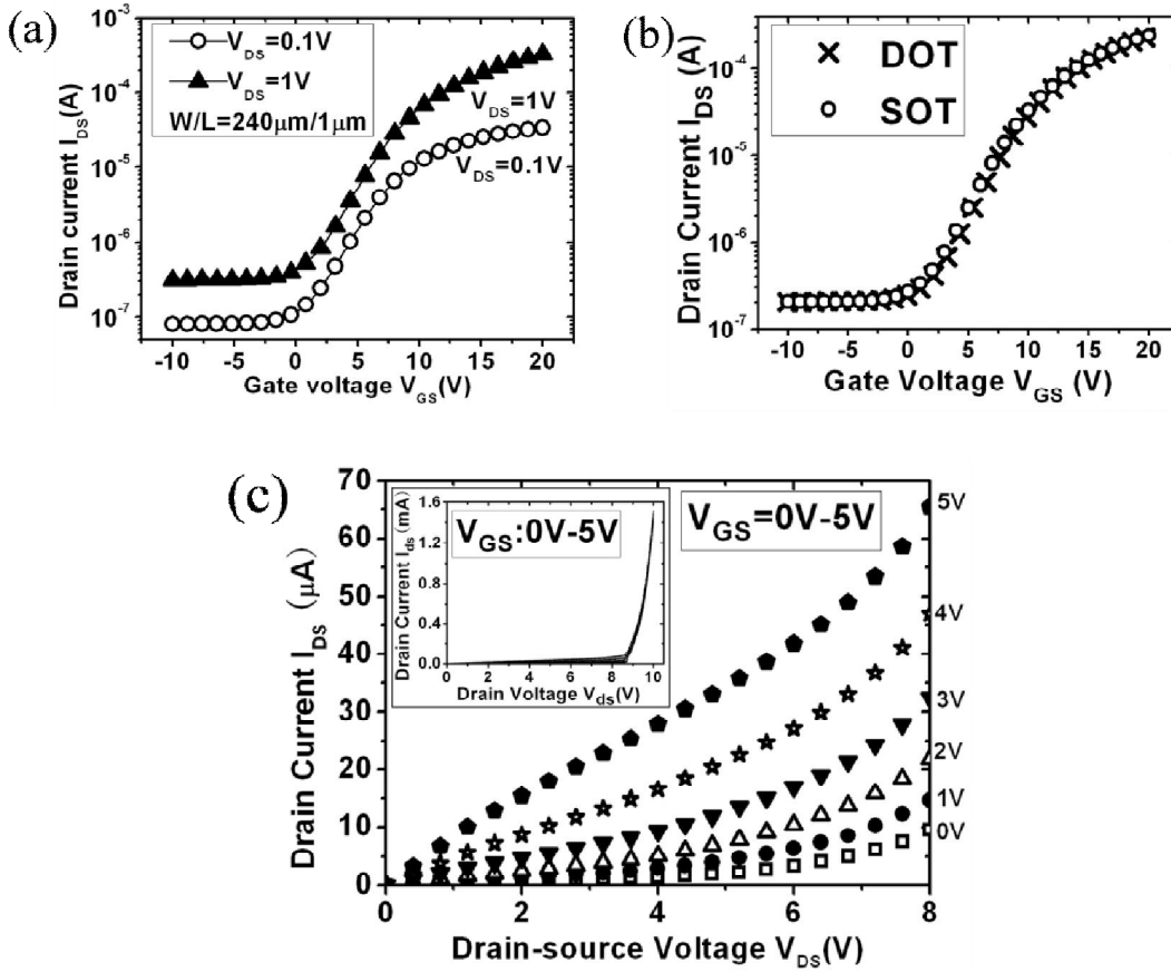
Figure 2-23: (a) Typical transfer characteristics, (b) symmetric transfer characteristics for DOT and SOT structures, (c) output characteristics of the classical VTFTs after the parasitic channel suppression, the inset in figure 2-23 (c) shows the strong kink effect when the drain voltage V_{DS} is higher than 8.5V.
