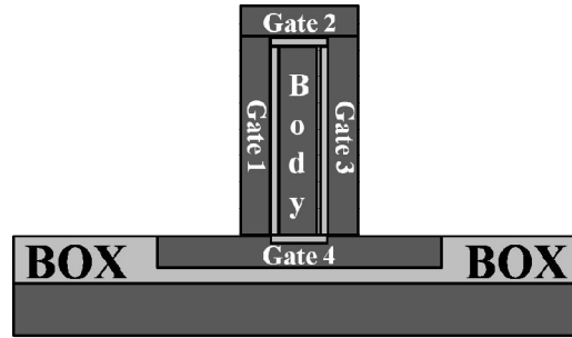
Figure 1-17: Cross-sectional view of the gate part for the gate-all-around (GAA) structure.
