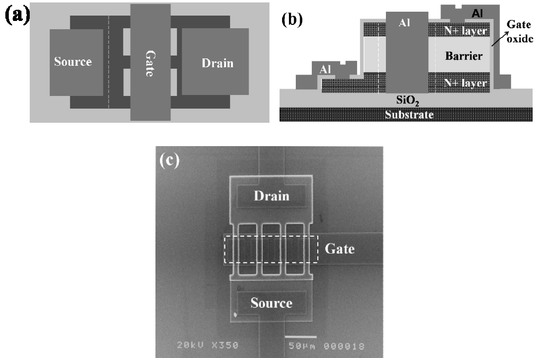
Figure 3-11: (a) Schematic top view, (b) side view of the final VTFT configuration, and (c) SEM top view of the fabricated four-tooth VTFT.
