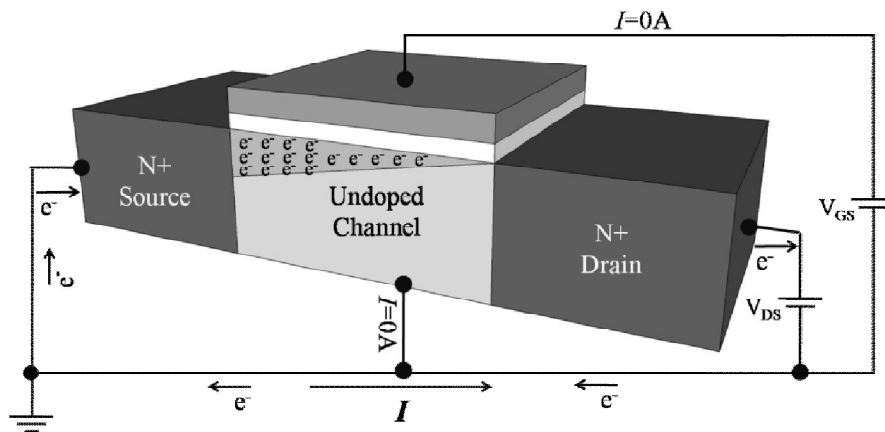
Figure 1-10: The electronic circuit of the LTFT, the channel is formed under the gate forward voltage V_{GS} , and the LTFT is at the on-state.
