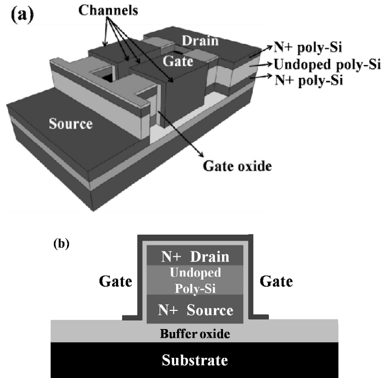
Figure 2-9: The classical VTFT structure: (a) the 3D view of a two-tooth VTFT, and (b) the basic structure of a VTFT tooth.
