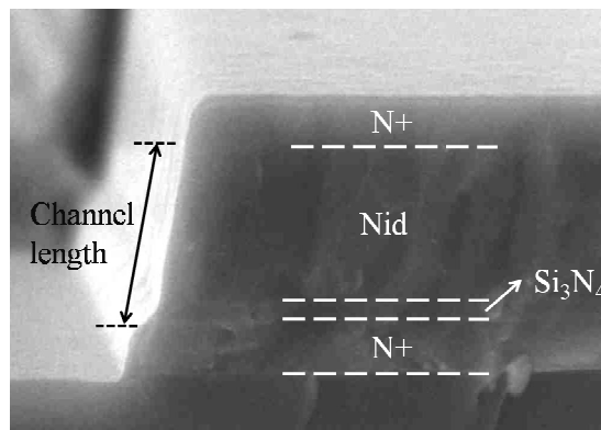
Figure 3-24: SEM image of the etched sidewall for the new VTFT with a 200 nm \text{Si}_3\text{N}_4 insulating layer.
