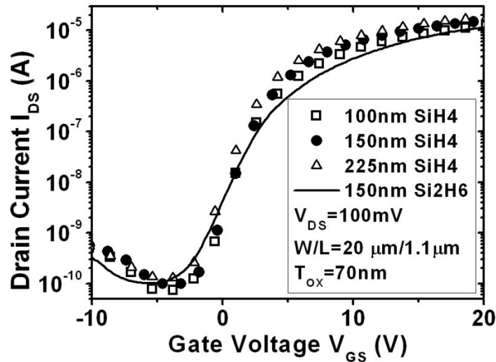
Figure 3-29: Transfer characteristics for different active layers.
