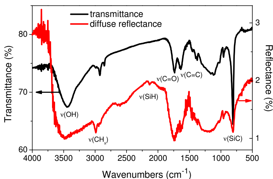
Figure 3.8: FTIR spectra (transmittance and diffuse reflectance) of palletized and ground SiC samples.
