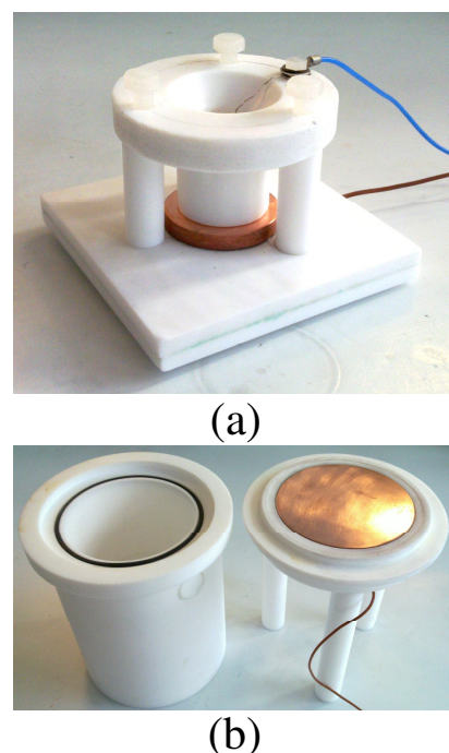
Figure 2.1: Etching cells for (a) small and (b) large quantity nano-SiC fabrication.
