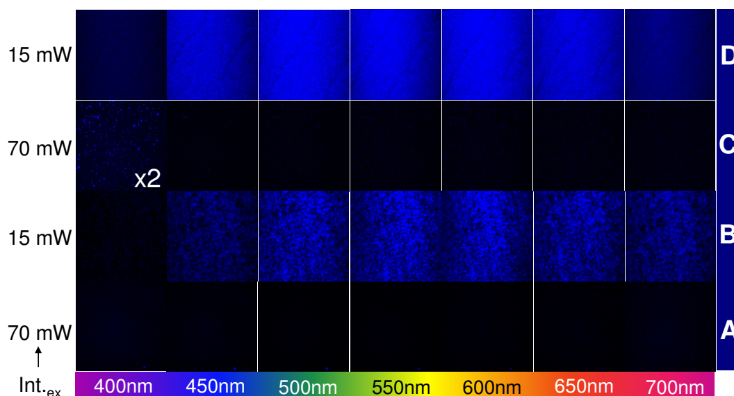
Figure 4.18: Fluorescence microscopy images of SiNx (a), nano-Ag/SiNx (b), SiC NPs/SiNx (c) and SiC NPs/nano-Ag/SiNx (d) samples, for SH (400nm) and several TPPL wavelengths (450, 500, 550, 600, 650 and 700 nm) with corresponding excitation ( \lambda = 800 nm) laser power.
