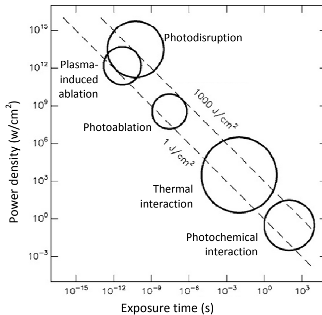
Figure 5.1 Map of laser-tissue interactions as a function of exposure time. The circles give only a rough estimate of the associated laser parameters, taken from [85]
