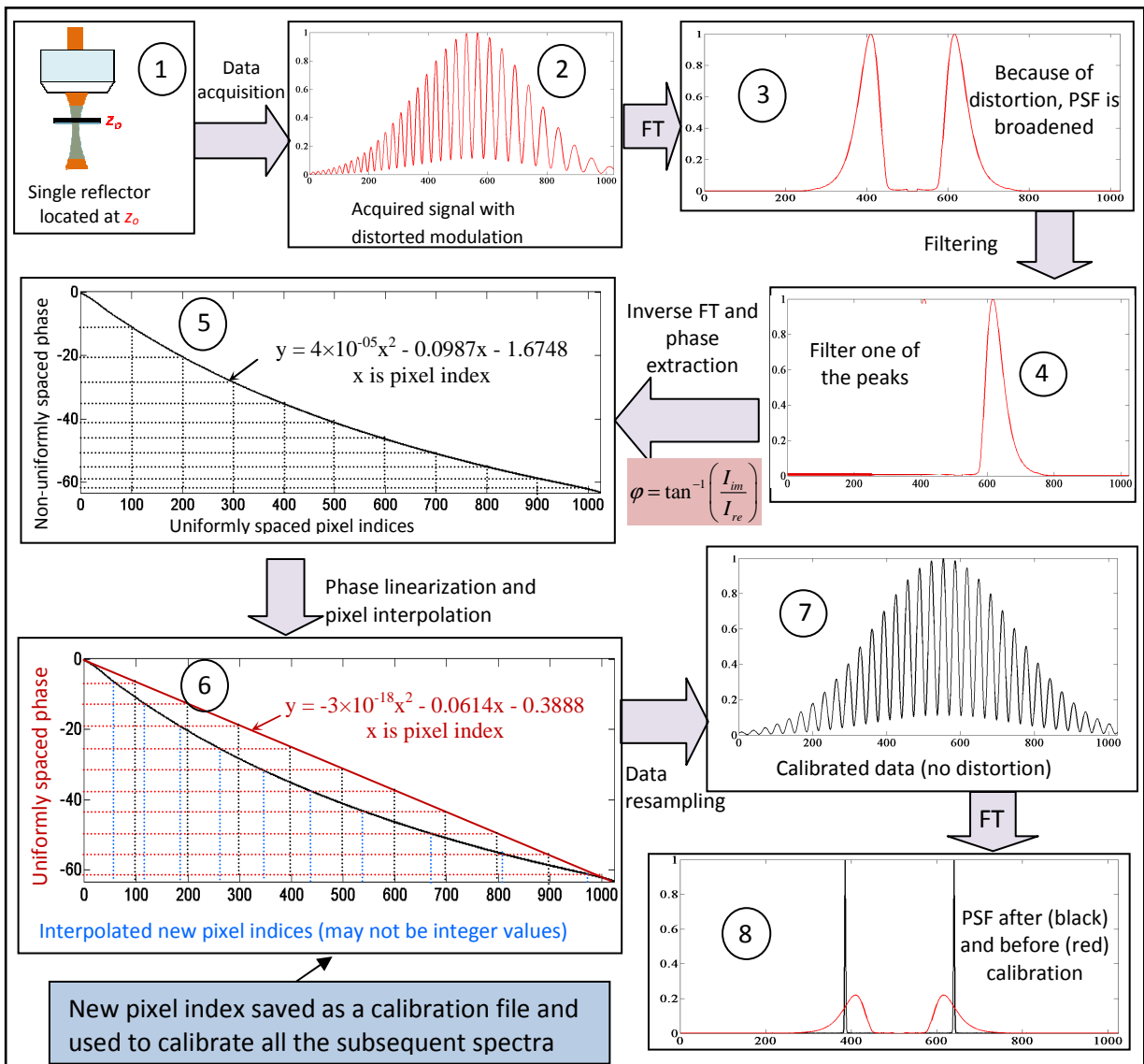
Figure 3.23 Numerical calibration procedure: starting with a distorted signal in panel 2 that is non-uniformly spaced in \sigma , a signal with uniformly spaced dataset is obtained in panel 7 via a numerical method of spectral calibration by extracting and linearizing the non-linear phase as explained in panel 3 to 6. After applying the Fourier transform, the corrected signal gives a narrow axial PSF (step 8) compared to the one shown in panel 3.
