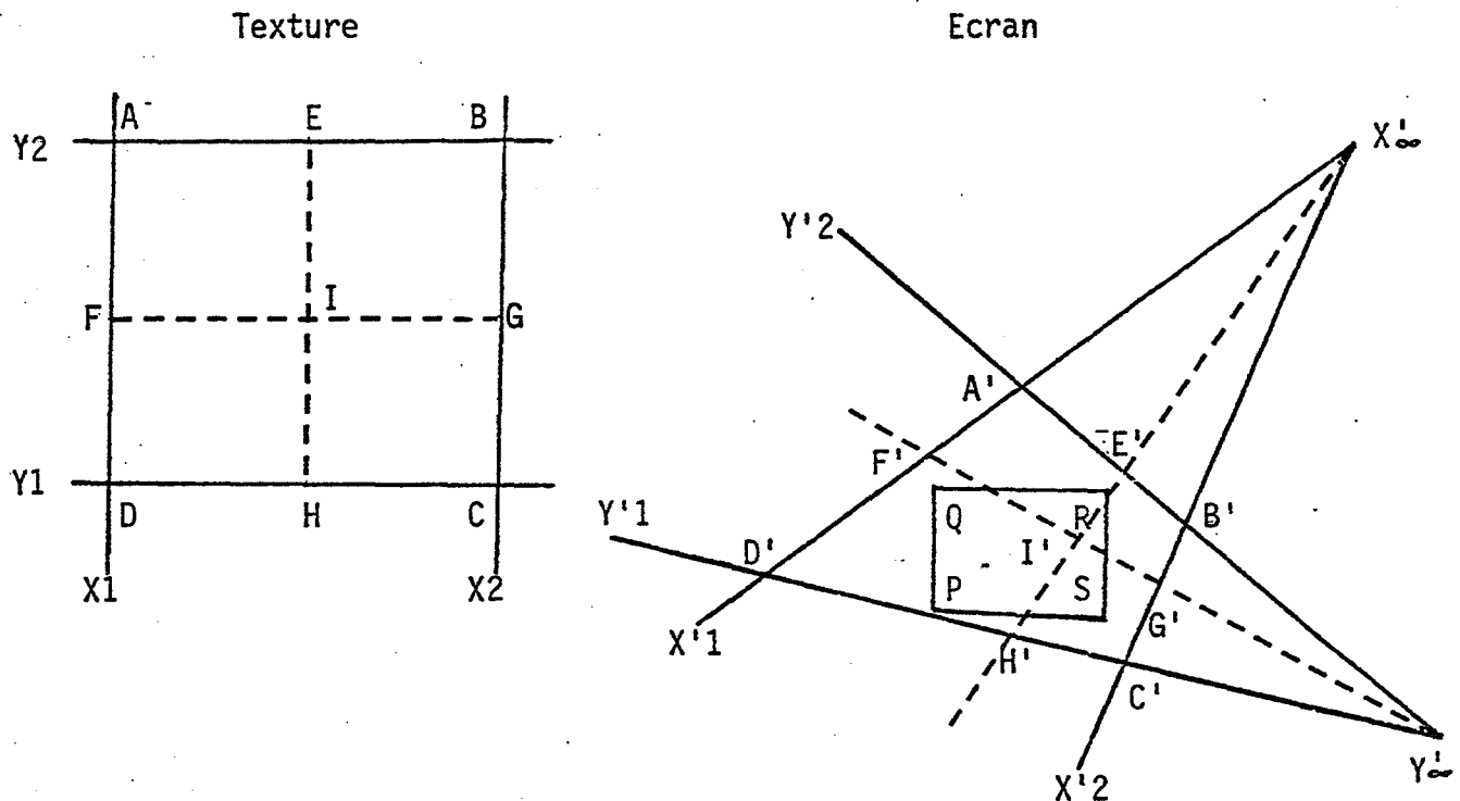
Figure 4-17 : Transformation perspective
