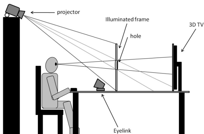
Figure 4.1: Schematic representation of the experimental apparatus used in the study. Observers seated facing the 3D display. The illuminated frame was placed in between. Drawing is not to scale.
