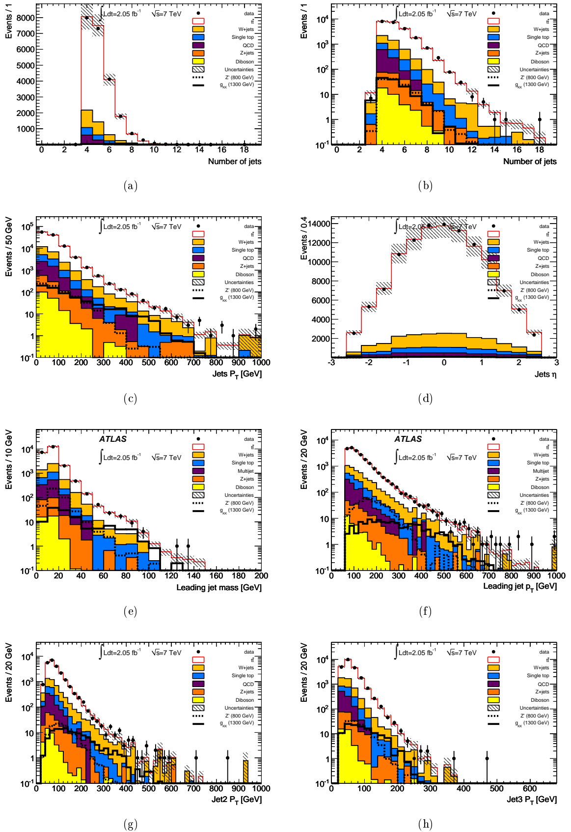
Figure 6.9: Number of jets with p_T > 20 GeV in (a) linear and (b) logarithmic scales, jets (c) p_T and (d) \eta distributions, (e) leading jet mass, (f) leading jet p_T , (g) second jet p_T and (h) third jet p_T after all selection criteria were applied. The grey hashed area shows the total background normalization uncertainty.
