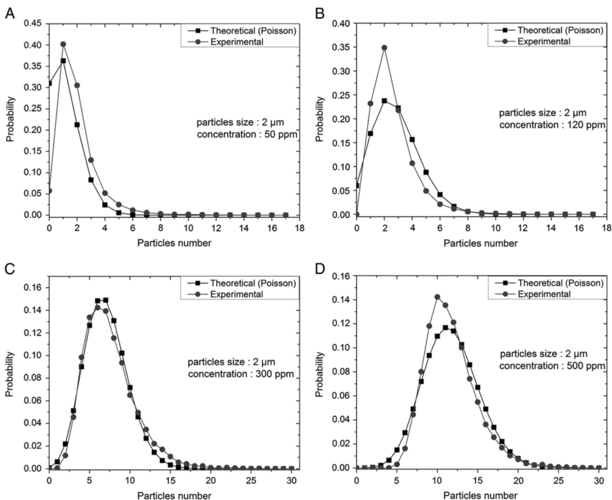
Fig. 9. Comparison of theoretical and experimental probabilities for 2µm Al 2 O 3 particles at different concentrations.
