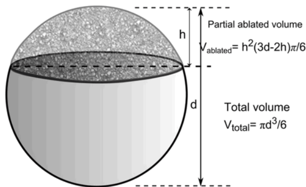
Fig. 10. Schematic view of partial particle ablation.
