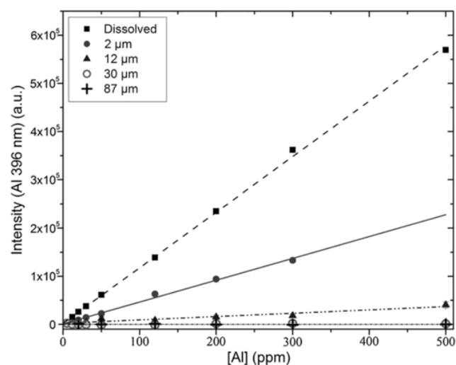
Fig. 3. Signal intensity of Al 396.1 nm line versus aluminum concentration in a solution and in suspensions of different diameter \text{Al}_2\text{O}_3 particles.
