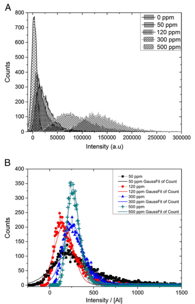
Fig. 7. Histogram of intensities for 2 μm Al 2 O 3 particles: (A) at different concentrations, (B) normalized intensities by Al concentration at different concentrations. The intensities and the normalized intensities obtained with 10,000 shots were classified in 600 channels.
