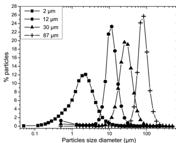
Fig. 2. Particle size diameter distribution for sifted \text{Al}_2\text{O}_3 powders with mean diameter of d_{50} = 2, 12, 30, 87\ \mu\text{m} .
