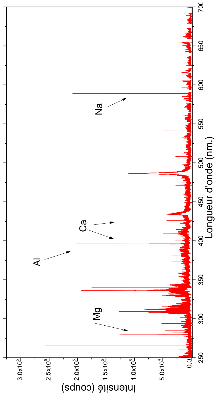
Spectre LIBS de la Bentonite Sigma-Aldrich Ref 285234.
