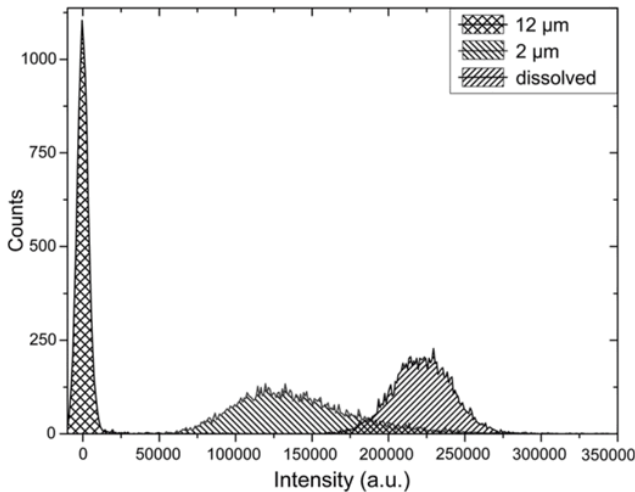
Fig. 5. Histograms of signal intensities obtained for dissolved aluminum solution, 2 μm Al 2 O 3 particles and 12 μm Al 2 O 3 particles in suspension at the same total Al concentration of 500 ppm. The intensities obtained with 10,000 shots were classified into 450 channel of 1000 a.u. width.
