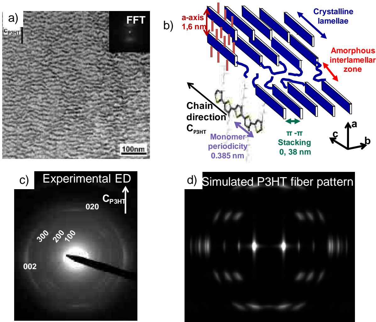
Figure 1-2: (a and c): TEM bright field (TEM-BF) image and corresponding electron (ED) diffraction pattern of a P3HT film grown by directional epitaxial crystallization on TCB. The BF image shows clearly the lamellar structure of the film with alternating crystalline domains (dark) and amorphous interlamellar zones (clear). The ED pattern is a typical fiber pattern. (b) schematical representation of the lamellar structure of a semi-crystalline P3HT film and crystallographic directions of the unit cell axes. (d) Simulated fiber pattern for a P3HT fiber with c P3HT as fiber axis Reproduced from (1).
