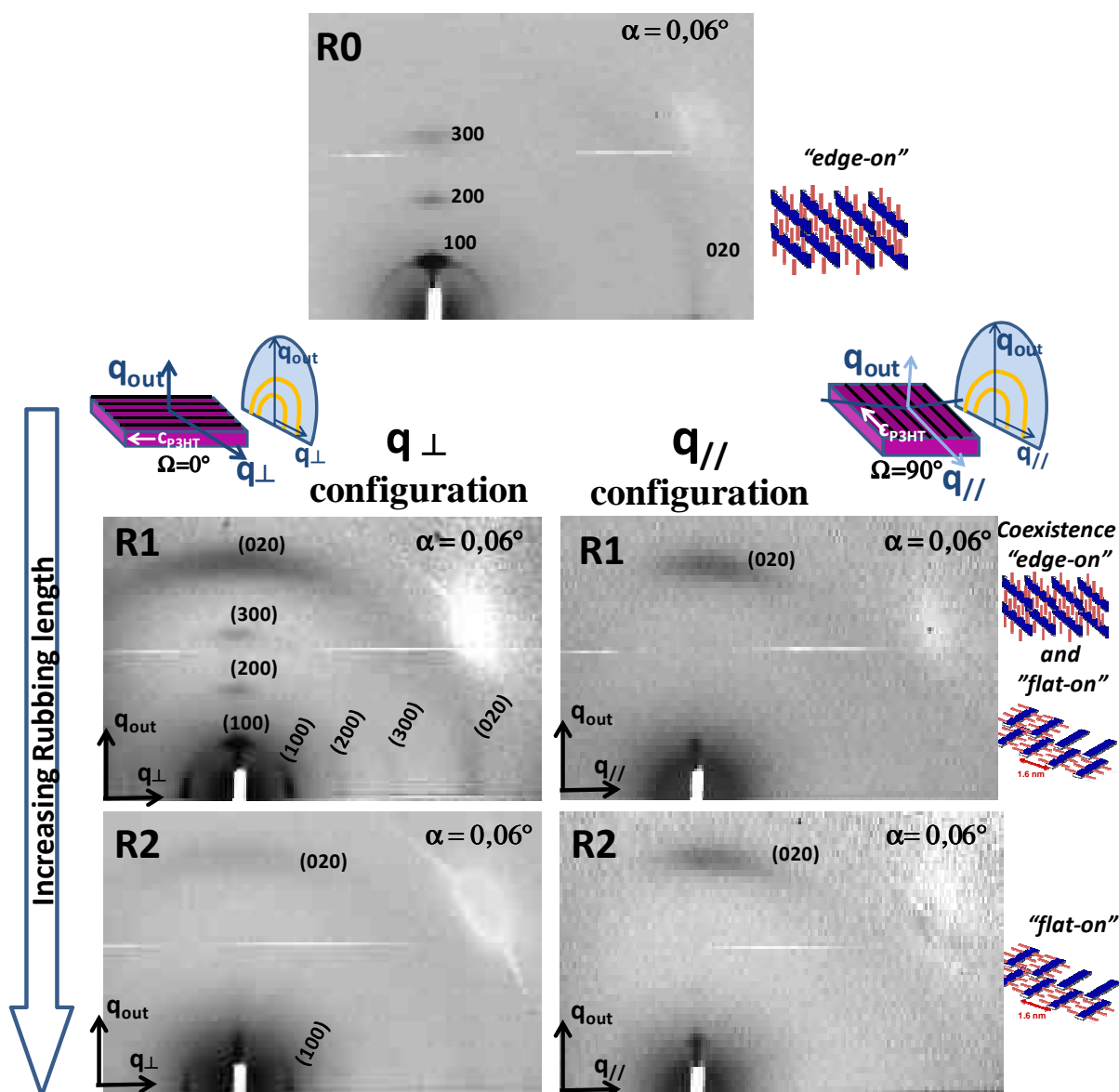
Figure 3-5 : 2D GIXD pattern of a medium- M_w sample before (R0) and after one (R1) and two (R2) rubbing cycles. The two scattering configurations q // R and q \perp R were used. The incidence angle of the beam was \alpha=0,06^\circ .
