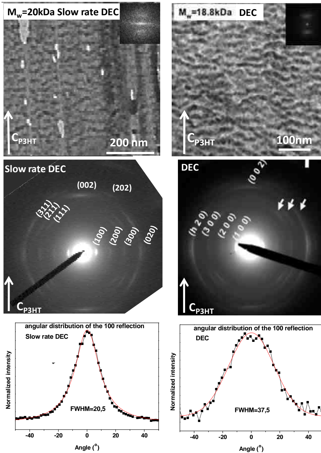
Figure 7-1 : (up) BF TEM images of a medium- M_w (20 kDa) P3HT thin film grown by slow DEC and a equivalent P3HT sample grown by the initial DEC method (reproduced from(4)). (middle) Corresponding ED patterns of the slow-DEC and DEC sample. (bottom) azimuthal angle distributions of the (100) reflections.
