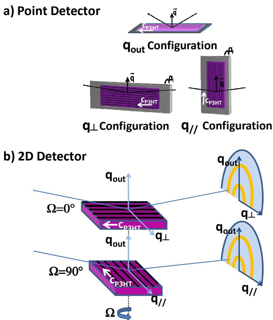
Figure 1-3: (a) Scattering configurations used for the GIXD measurements with the point detector. (b) Scattering configurations used with the 2D detector. \vec{q}_{\perp} is defined as the scattering vector perpendicular to the \vec{c}_{P3HT} direction and \vec{q}_{//} is defined as the scattering vector parallel to the \vec{c}_{P3HT} direction and the \vec{q}_{out} vector is along the sample's surface normal.
