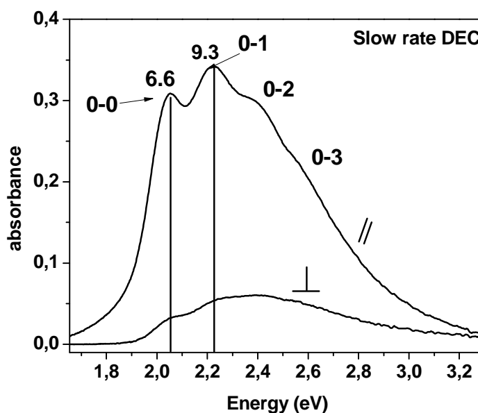
Figure 2-9: UV-vis absorbance spectra of P3HT thin films (medium- M_w ) prepared by slow-DEC in TCB for the incident light polarized parallel ( \parallel ) and perpendicular ( \perp ) to c_{TCB} . The numeric values in the figure correspond to the measured dichroic ratio at two wavelengths. The spectrum is an average spectrum of 5 different locations on a sample.
