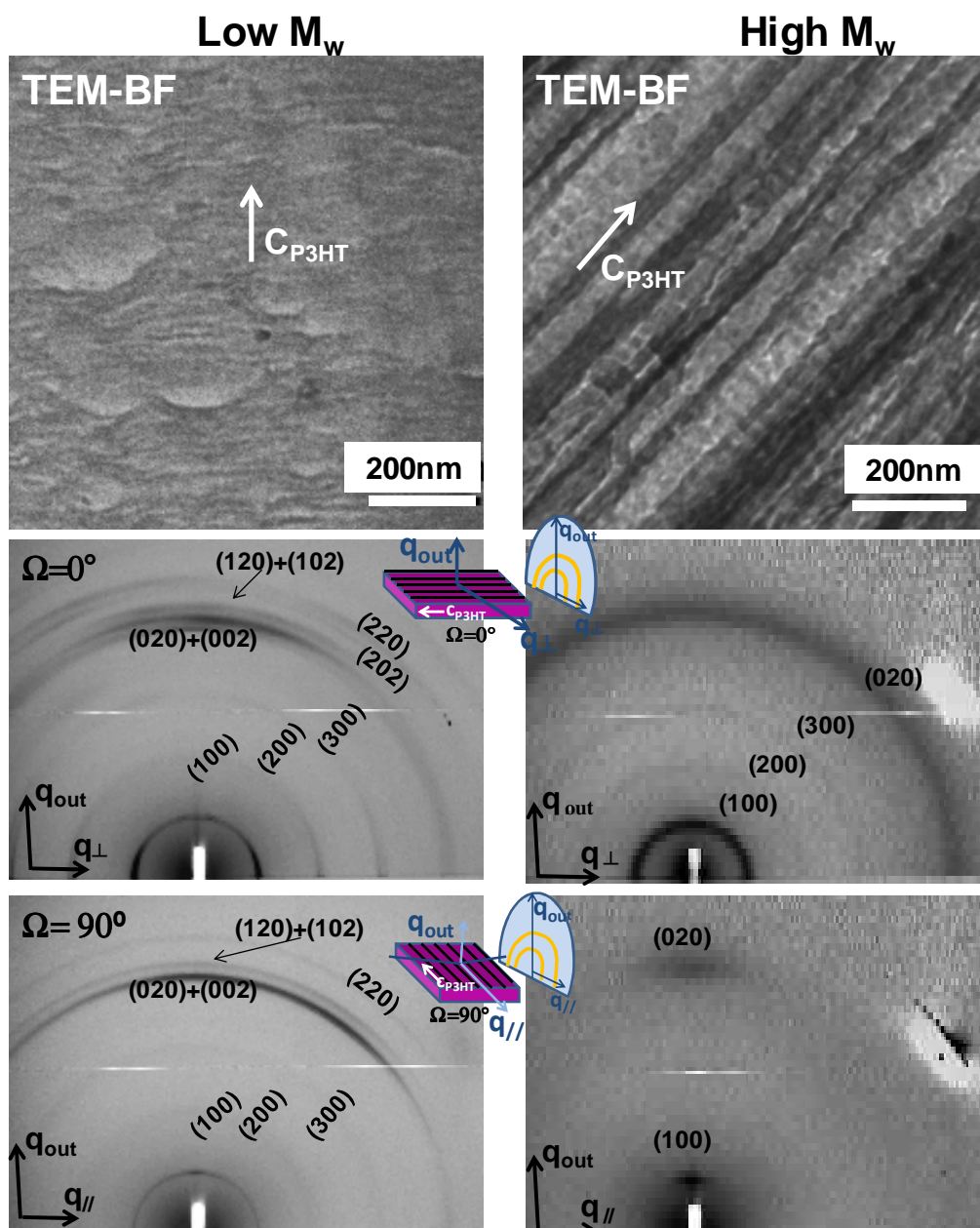
Figure 2-3: (Top) TEM- BF images of a low and high- M_w sample (middle) 2D GIXD pattern of a low and high- M_w sample the scattering vector \mathbf{q}_\perp \perp \mathbf{c}_{P3HT} . (bottom) 2D GIXD pattern of a low and high- M_w sample the scattering vector \mathbf{q}_\parallel \parallel \mathbf{c}_{P3HT} . For means of comparison the results of the low- M_w are redisplayed.
