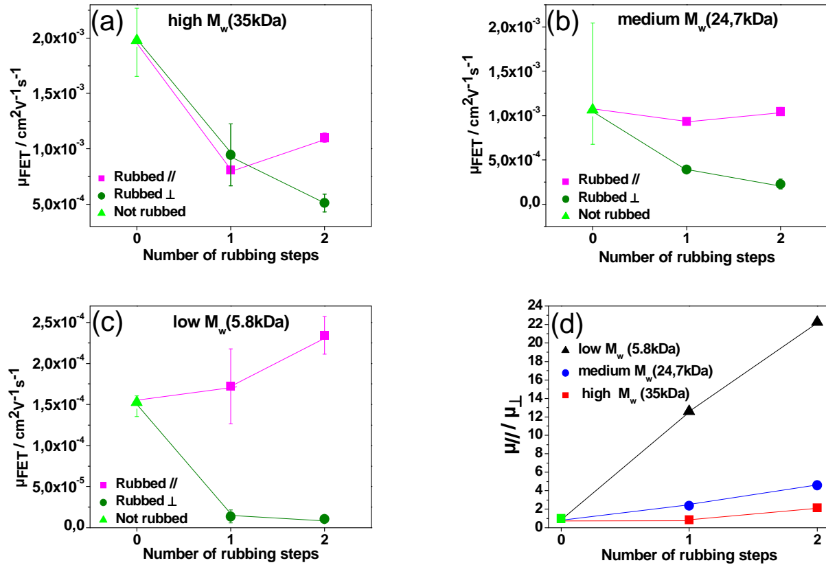
Figure 4-9: Measured field effect mobility parallel ( \mu_{\parallel} ) and perpendicular ( \mu_{\perp} ) to the rubbing direction as a function of rubbing steps for P3HT with different molecular weights (a) high M_w=35 kDa, (b) medium M_w=24.7 kDa and (c) low M_w=5.8 kDa. (d) Ratio of \mu_{\parallel} and \mu_{\perp} as a function of rubbing steps for the three different molecular weights.
