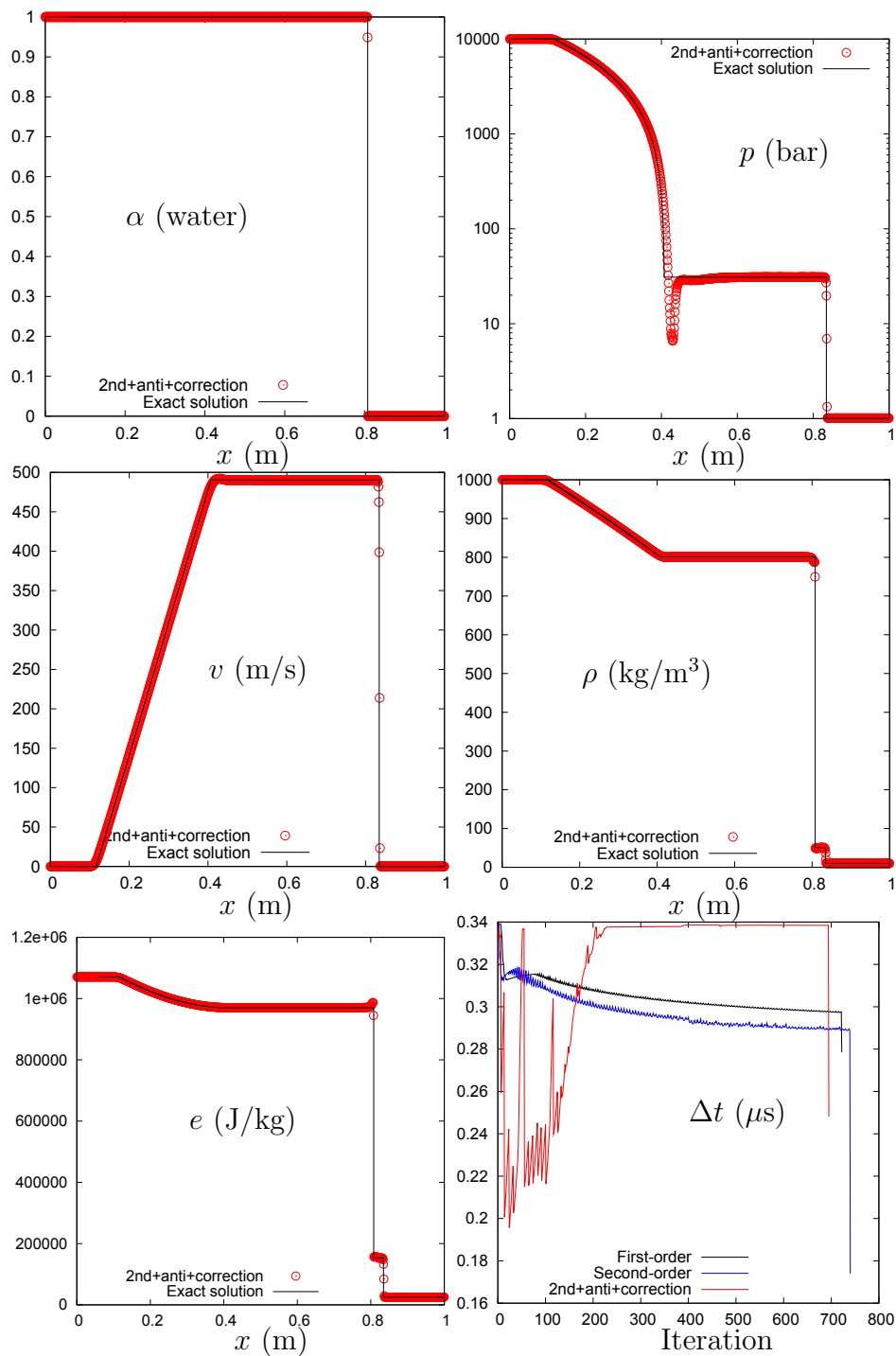
Figure 3.8: Limited second-order DEM method (minmod) with corrected anti-diffusive approach for water gas shock tube with impermeable interface ([Petitpas 07]). 1000 computational cells. t = 220 \mu\text{s} . CFL = 0.9. Residual phase volume fraction is set as 10^{-6} .
