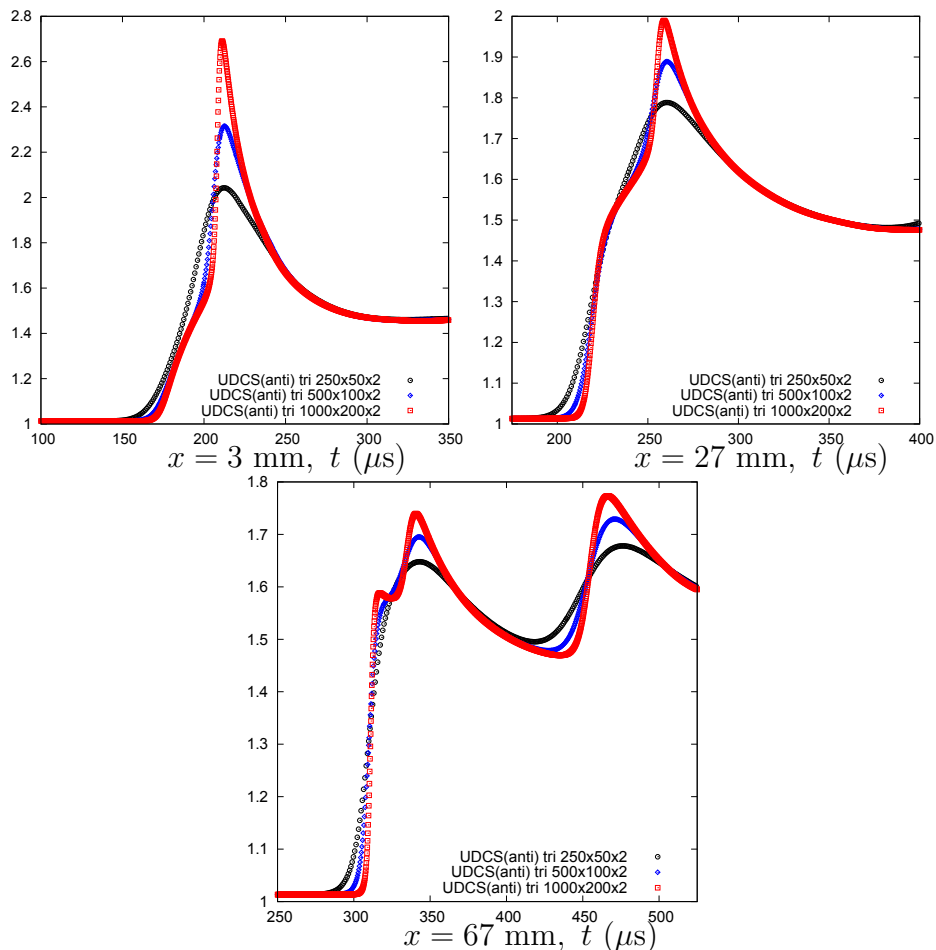
Figure 5.7: Air-R22 shock cylinder interaction test. Time history of pressure in three locations: x = 3 \text{ mm} , x = 27 \text{ mm} , and x = 67 \text{ mm} downstream of the R22 gas bubble along the axis of symmetry. Anti stands for UDCS anti-diffusive approach. tri stands for triangular mesh.
