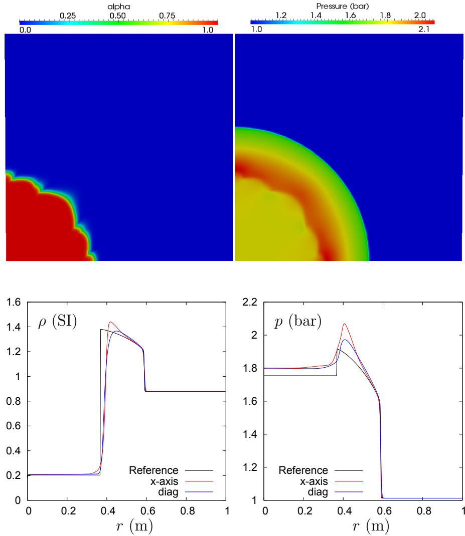
Figure 5.14: Propagation of a 1D line-symmetric steady flame. (Quasi) second-order UDACS + RDEM, with minmod reconstruction for all primitive variables (second-order explicit Runge-Kutta scheme for time discretization). On the top: the volume fraction of the burnt gas and the pressure. On the bottom: the plots of density over axis and diagonal, and that of pressure. The reference solution is obtained using a 1D line-symmetric solver and the UDACS anti-diffusive approach.
