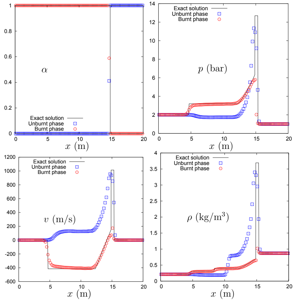
Figure 4.4: UDCS anti-diffusive RDEM method (minmod for \rho , v , p ) is used for shock tube of Chapman-Jouguet deflagration front. A 100 cells uniform mesh is used. CFL = 0.9. Time t = 4.0 ms. Individual phase variables are plotted.
