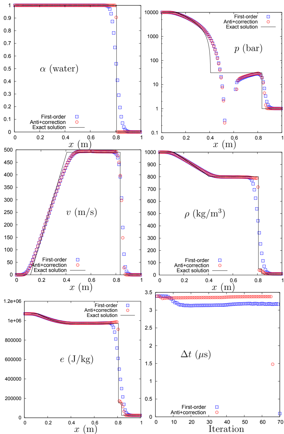
Figure 3.6: First-order DEM method with corrected anti-diffusive approach for water gas shock tube with impermeable interface ([Petitpas 07]). 100 computational cells. t = 220 \mu\text{s} . CFL = 0.9. Residual phase volume fraction is set as 10^{-6} .
