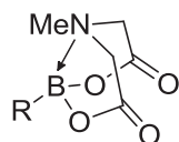
Figure 2 Structure d'un boronate MIDA.
