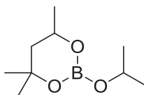
Figure 8 MPBO i Pr 4.
