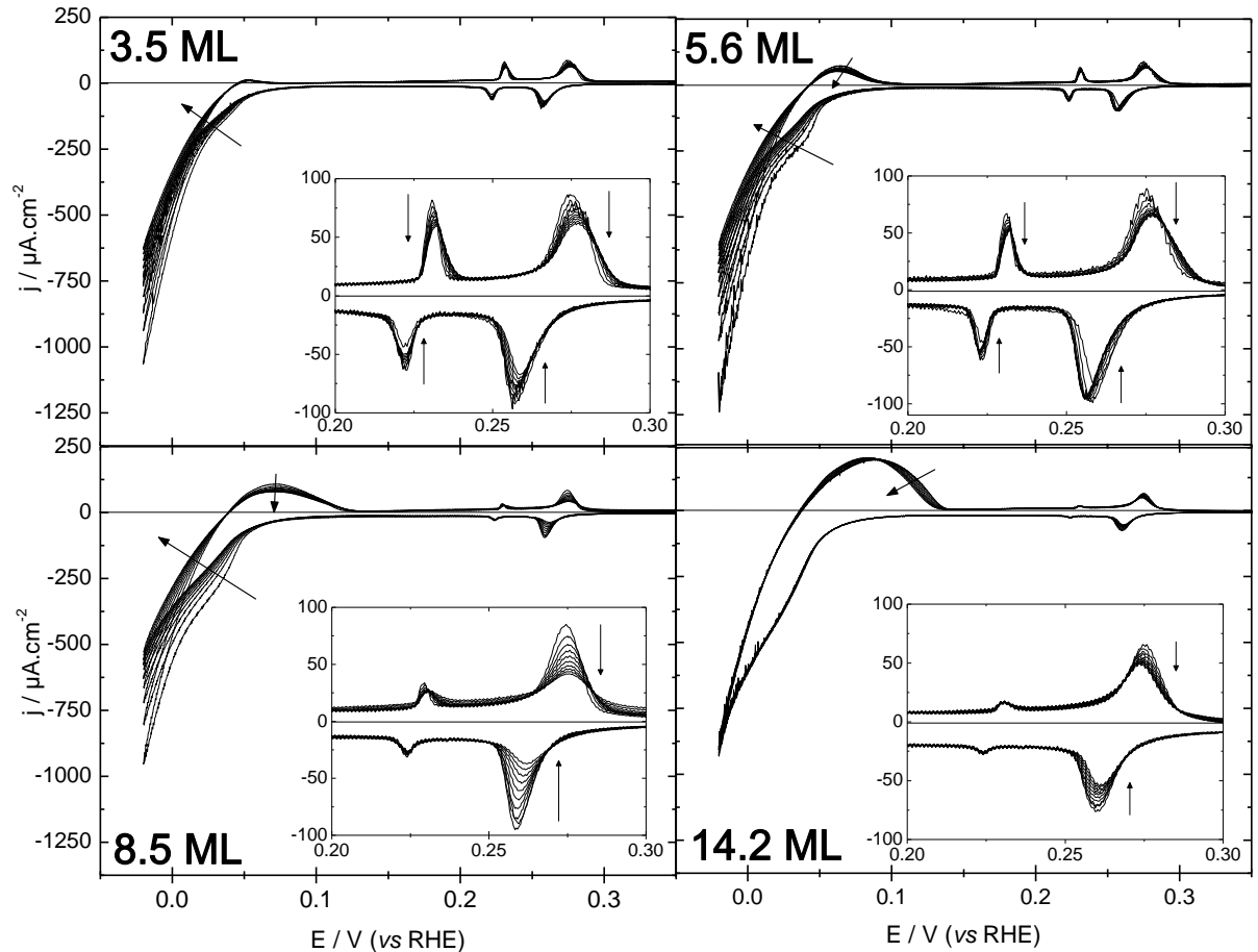
Figure 4.16 : Ageing process: 10 first cycles for hydrogen insertion/desinsertion on \text{Pd}_{x\text{ML}}/\text{Pt}(111) in 0.1 \text{ M H}_2\text{SO}_4 at 10 \text{ mV}\cdot\text{s}^{-1} and 800 \text{ rpm} . Insets: enlargement of high potential region.
