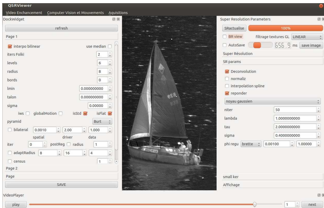
Figure C.2 – Interface SRViewer
