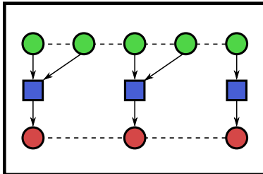
Figure 2.14 – Pattern down-sampling
