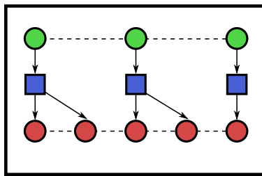
Figure 2.16 – Pattern up-sampling
