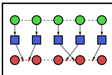
Figure 2.19 – Pattern Vote
