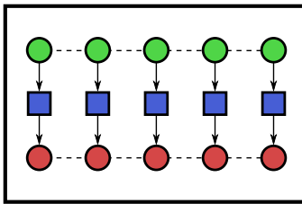
Figure 2.10 – Pattern pixel-à-pixel
