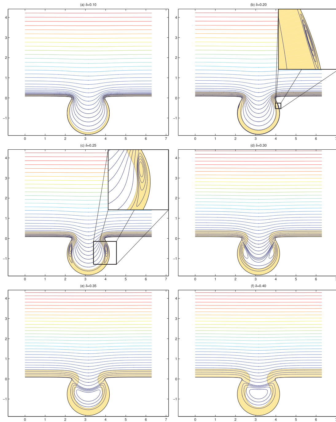
FIGURE 4.6 – Streamlines corresponding to the mapping (4.42) for different values of the boundary layer width \delta , \delta = 0.1 (a), \delta = 0.2 (b), \delta = 0.25 (c), \delta = 0.3 (d) \delta = 0.35 (e) and \delta = 0.4 (f). The boundary layer width is symbolised by the coloured area near the boundary. (The distance between two streamlines is arbitrary)
