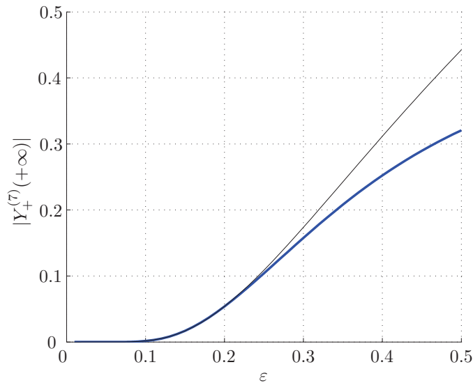
FIGURE 2.4 – Final amplitude |Y_+^{(7)}(+\infty)| as a function of \varepsilon . Computation (bold line), fitted \mathcal{A}e^{-\mathcal{C}/\varepsilon} curve (thin line).
