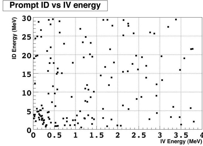
Figure 5.10: ID energy as a function of the IV energy for IVT events. Since the IVT rely on the high multiplicity the FNs are created by their parent muon, the tagged FN is a separated event from the one interacting in the ID. An excess of events in E_{ID} \lesssim 5 MeV and E_{IV} \lesssim 1 MeV suggest some background contaminate the IVT sample.
