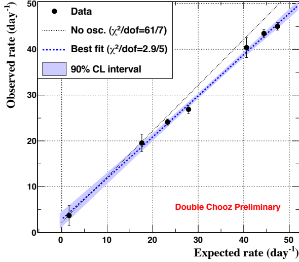
Figure 4.14: Observed \bar{\nu}_e rate as a function of the non-oscillated expected rate. The dashed line show the fit to the data, the dotted line shows the expectation in case of null-oscillation hypothesis. The extrapolation to zero reactor power, i.e zero expected rate, of the fit to the data point provide a background measurement of 2.9 \pm 1.1 event per day.
