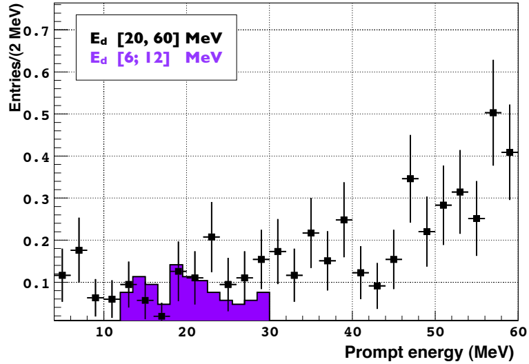
Figure 5.30: Comparison between SM prompt spectrum obtained by selecting the delayed candidate at high energy, [20, 60] MeV, and low energy, [6, 12] MeV. The prompt spectra are in agreement within uncertainty.
