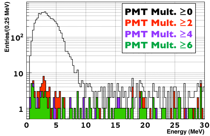
Figure 5.11: Prompt energy spectrum for different IVT multiplicity condition. The IVT based on the number of IV PMT hit allows then to tag FN events produced with high multiplicity by a muon interacting outside the detector. The tagging efficiency is measured between 33 % and 23 %, depending on the multiplicity condition. An excess of events in E_{ID} \lesssim 5 MeV suggest some background contaminate the IVT sample.
