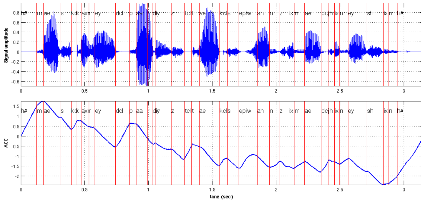
Figure 5.2: top : The speech signal "Masquerade parties tax one's imagination" from the TIMIT database and bottom : the ACC functional of Eq. (5.9). The functional is detrended by subtracting its global mean.
