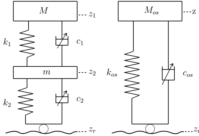
Figure 5.1: DSS model and equivalent OSS model
