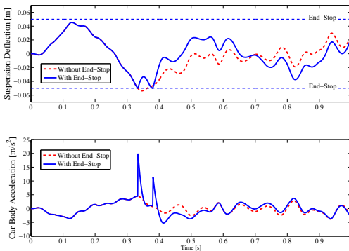
Fig. 2. Time history of the suspension deflection (top) and the body acceleration (bottom), with and without the end-stops.
