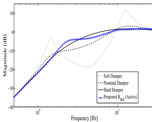
Figure 4.19: Bode diagram: dynamic tire deflection (z_{us} - z_r)/z_r (Road Holding Controller K_{RH} ).
