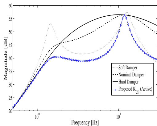
Figure 4.15: Bode diagram: vehicle body acceleration \ddot{z}_s/z_r (Comfort controller K_{CF} ).
