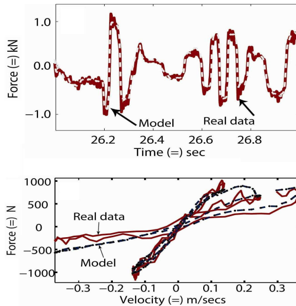
Figure 3.6: Model's force v.s real data
