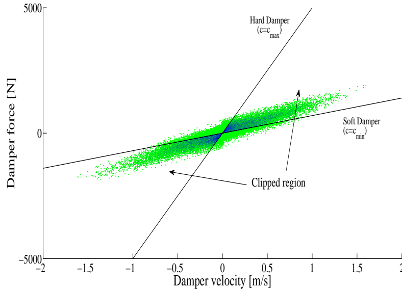
Figure 4.11: Damper Force v.s Damper Velocity. The active forces are present in all the plane while the semi-active forces are limited in the clipped region.
