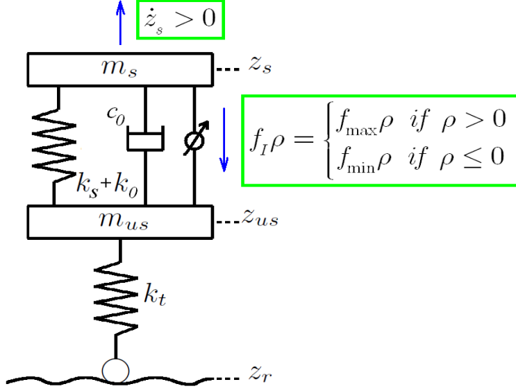
Figure A.1: Illustration of the extended Skyhook control for MR damper
