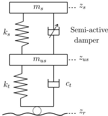
Figure 6.4: Model of quarter vehicle with a semi-active damper.
