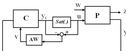
Figure 6.2: Closed-loop plant with anti-windup controller.
