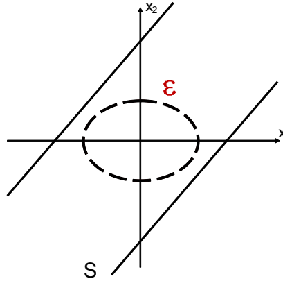
Figure 2.12: Invariant set approach for stability: \mathcal{S} validity region of saturation, \mathcal{E} contractive set
