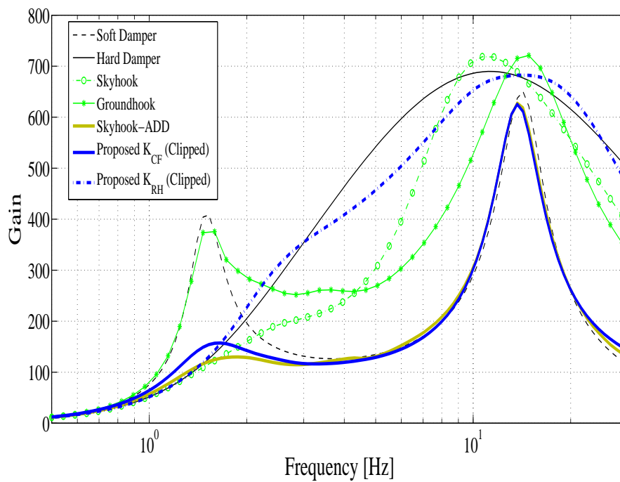
Figure 4.20: Nonlinear frequency responses \ddot{z}_s/z_r (nonlinear simulation).
