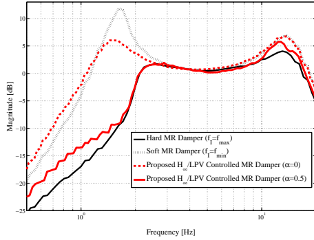
Fig. 8. Frequency responses z_{def}/z_r
