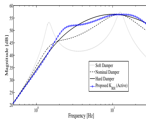
Figure 4.18: Bode diagram: vehicle body acceleration \ddot{z}_s/z_r (Road Holding Controller K_{RH} ).
