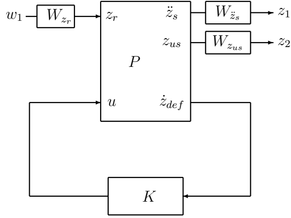
Figure 4.5: Control Block Diagram for Strong Stabilization Approach
