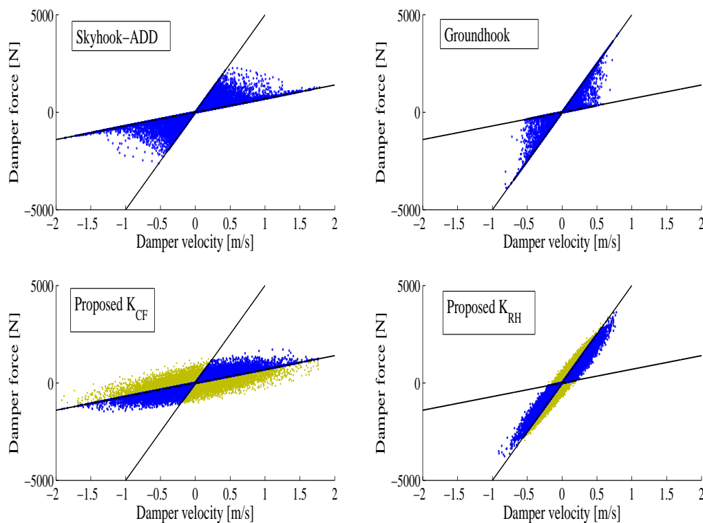
Figure 4.25: Comparison of the Force-Velocity characteristics.
