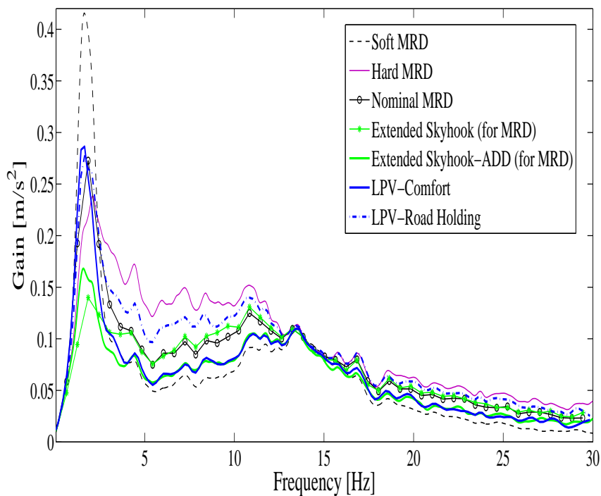
Figure 3.24: Spectrum of z_s (test with a load transfer condition).
