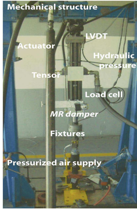
Figure 3.4: Experimental test-rig for MR damper parameter identification
