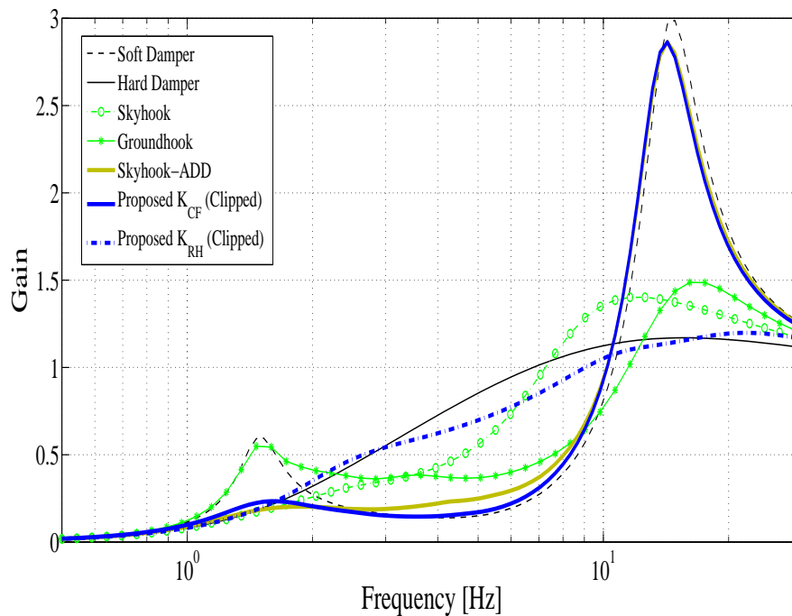
Figure 4.21: Nonlinear frequency responses z_{us} - z_r/z_r (nonlinear simulation).
