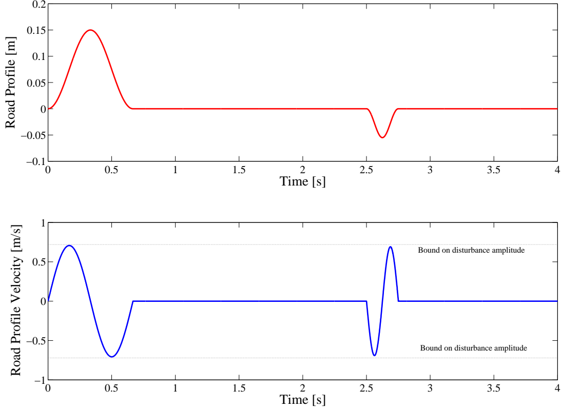
Figure 6.5: Road Profile.
