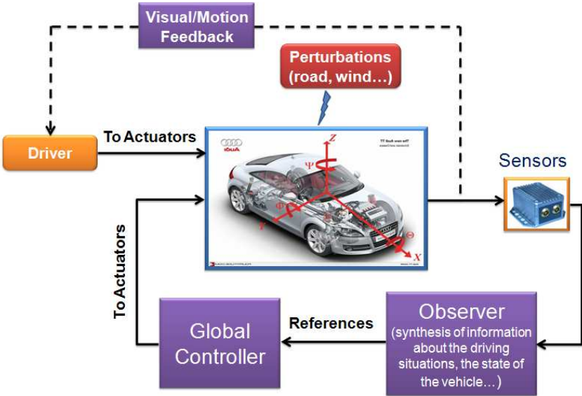
Figure 7.2: Global chassis control
