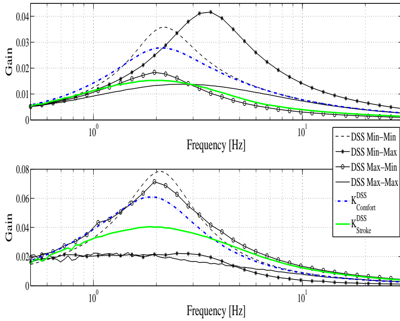
Figure 5.10: DSS system - Nonlinear frequencies responses (z_1 - z_2)/\dot{z}_r (Top) and (z_2 - z_r)/\dot{z}_r (Bottom).
