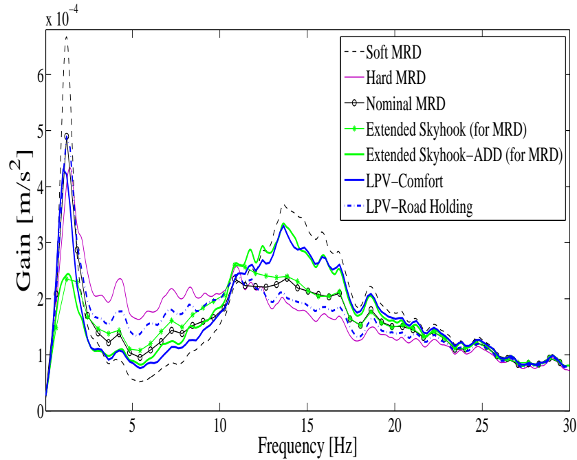
Figure 3.22: Spectrum of z_{us} - z_r (test with an increase of 75% in sprung mass).
