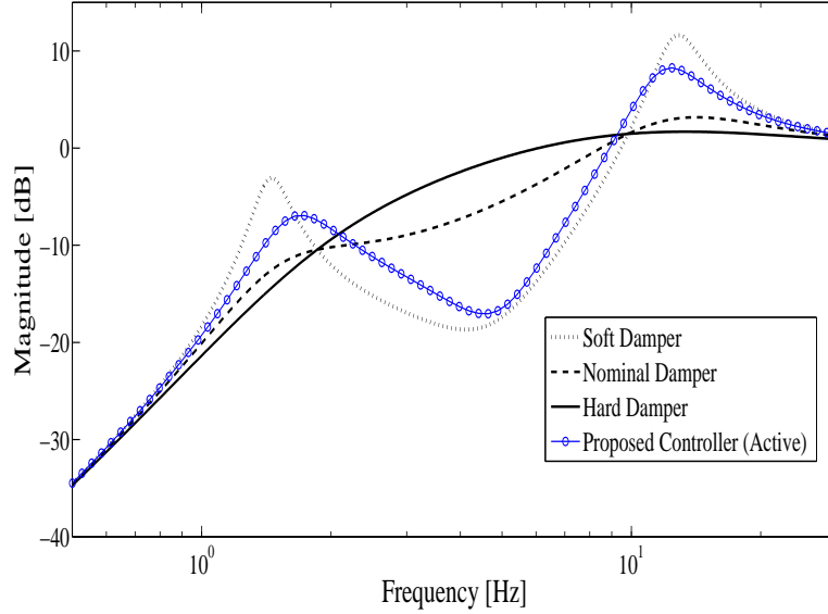
Figure 4.10: Bode diagram (z_{us} - z_r)/z_r .
