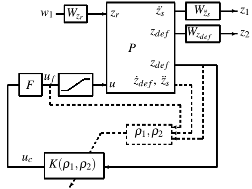
Fig. 6. Structure for H_\infty /LPV controller design.
