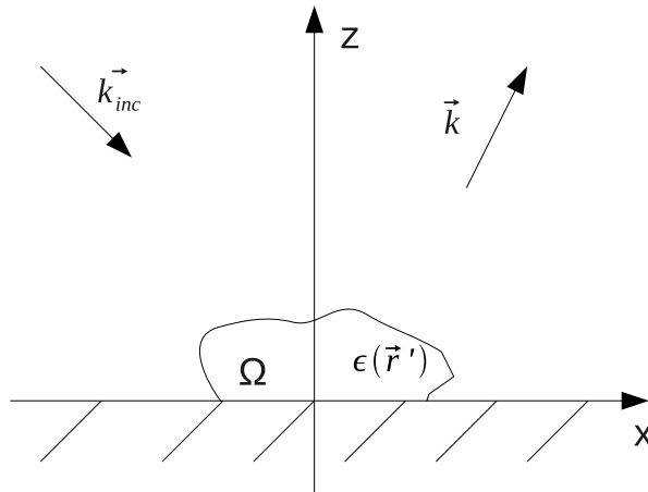
Figure 4.1: Sketch of the mirror-assisted Tomographic Diffraction Microscopy. The sample is illuminated successively by several incident plane waves with wave vectors \mathbf{k}_{\text{inc}} . For each incident plane wave, the diffracted field is measured for all \mathbf{k} directions that are accessible through the objective.
