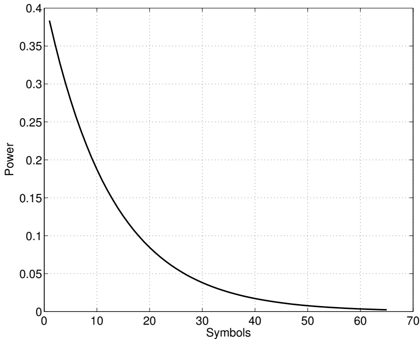
Figure 2.11: Power profile of the column precoder when L = l = 1 , |h_{p,0}/h_{p,1}| < 1 .
