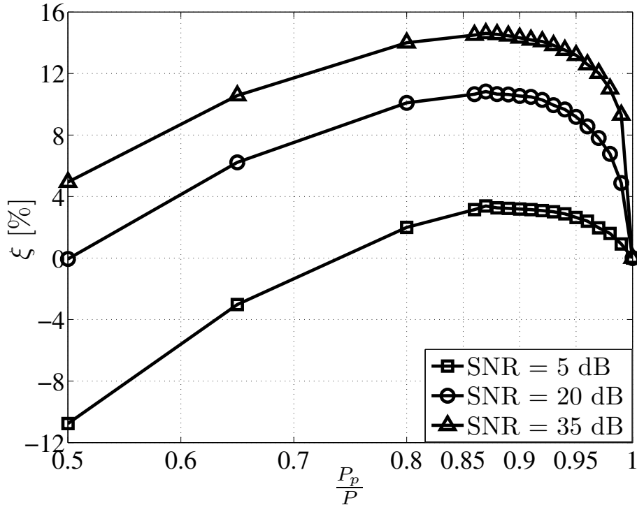
Figure 7.2: Percent energy efficiency change w.r.t. the legacy OFDM FBS for a uniform Rayleigh fading channel.
