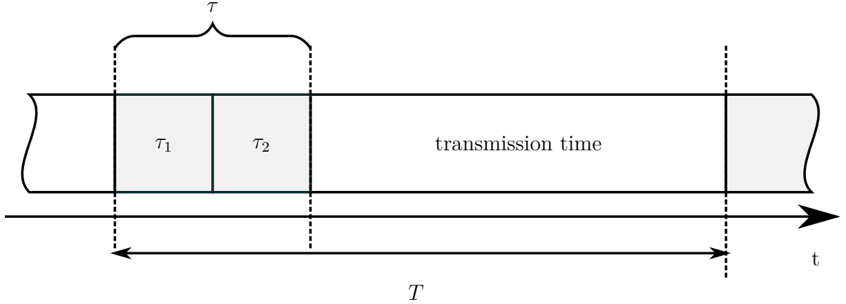
Figure 5.1: Channel estimation and transmission times.
