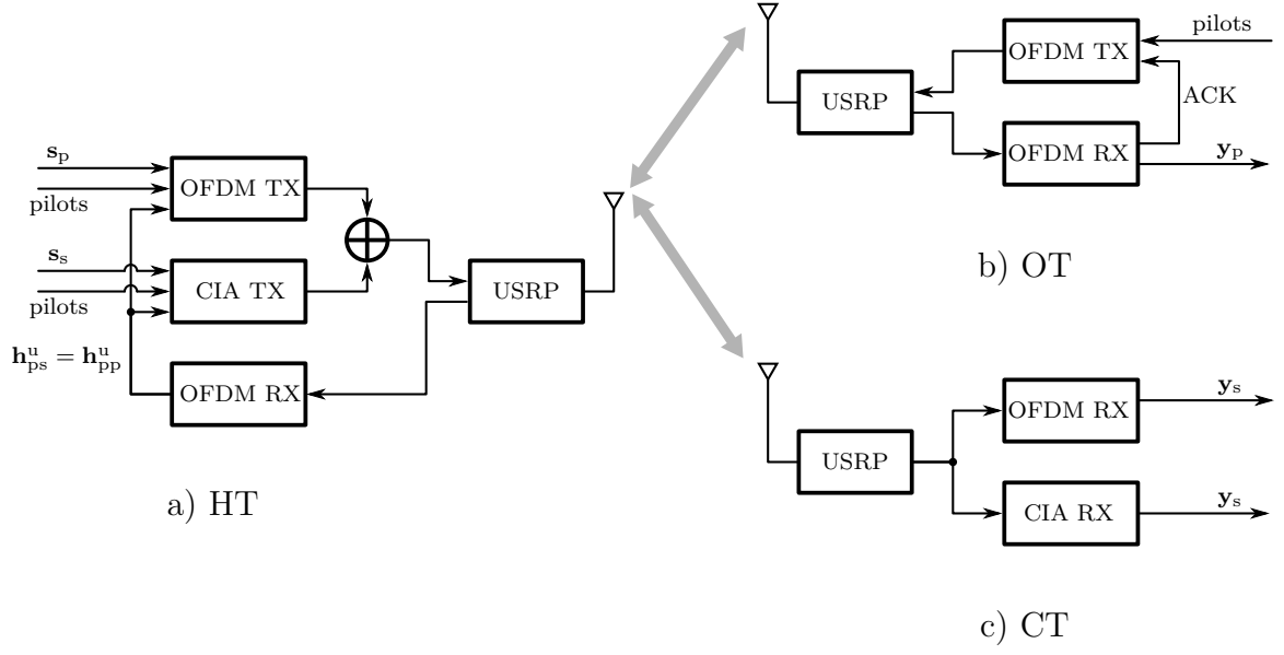
Figure 8.2: Transceivers structure.
