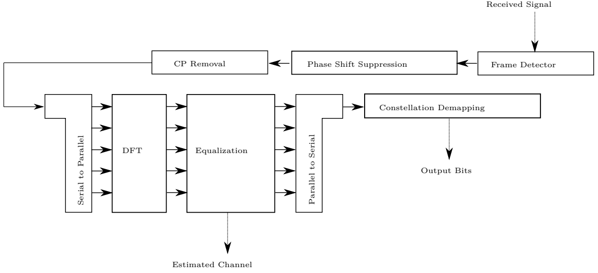
Figure 2.5: VFDM RX block diagram.
