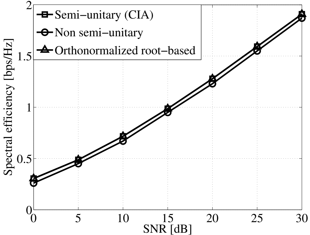
Figure 3.2: Spectral efficiency of the secondary link. Uniform PDP.
