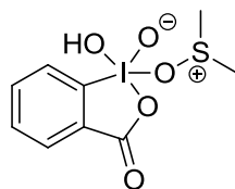
Figure 8 : IBX-DMSO
