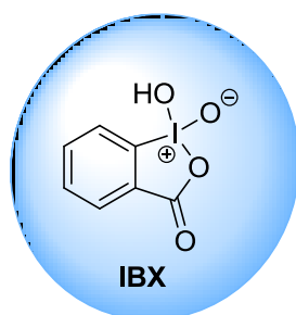
Figure 5 : Acide o -iodoxybenzoïque
