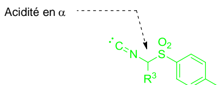
Figure 4 : TosMIC
