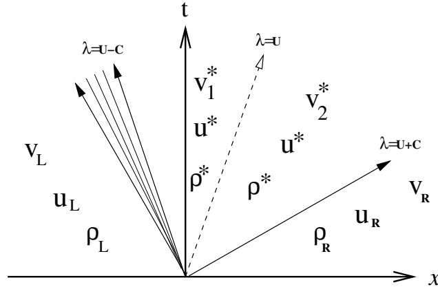
FIG. 3.3 – Intermediate states for u , \rho and v
