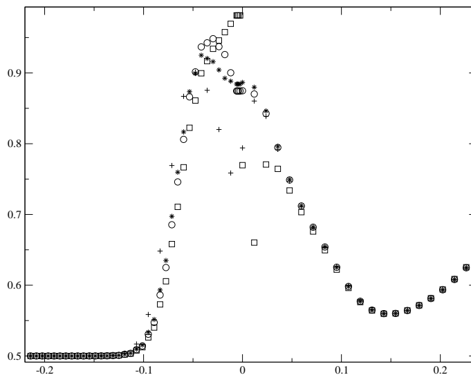
FIG. B.2 – Solution for the density on the line y=0 . Crosses stand for the two-dimensional reference solution, stars stand for the natural interface model (which does not respect the (NSC)), circles stand for the non conservative admissible interface model and squares stand for the conservative admissible interface model.
