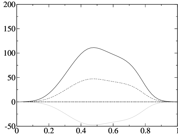
FIG. C.5 – Riemann problem 1: velocity U_r and imaginary part of eigenvalues. (no drag) - 50 cells
