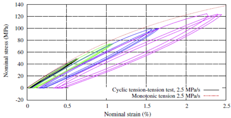
(a) 3 cycles per stress level (50, 75, 100, 125 MPa)
