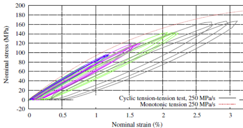
(b) 3 cycles per stress level (40, 70, 95, 120, 140 MPa)
