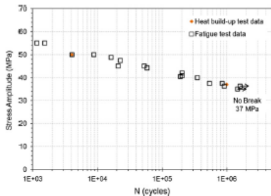
Fig. 7. Fatigue curve obtained for ISO527 samples, R = 0 , f_0 = 1 Hz.
