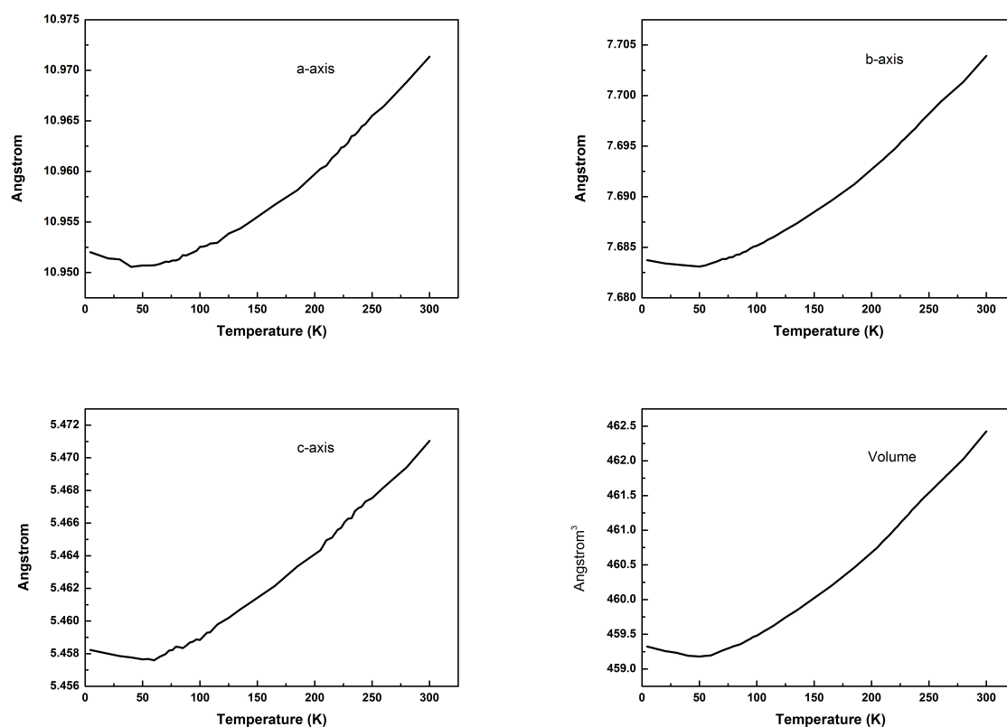
Figure 5.17.: Lattice parameter and volume change versus temperature of \text{Sr}_4\text{Fe}_4\text{O}_{11}
