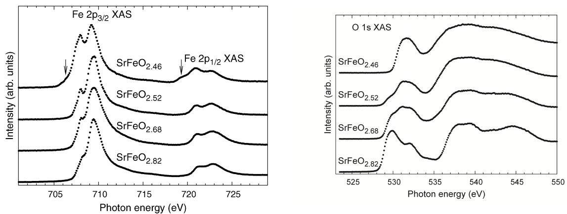
Figure 4.6.: The figures are reproduced from Ref. [67]. The left panel shows the Fe- L_{2,3} edge x-ray absorption spectra of polycrystalline \text{SrFeO}_{2.46} , \text{SrFeO}_{2.52} , \text{SrFeO}_{2.68} and \text{SrFeO}_{2.82} . The arrows indicate features formed by \text{Fe}^{2+} ions. The right panel depicts oxygen- K edge x-ray absorption spectra of these compounds.
