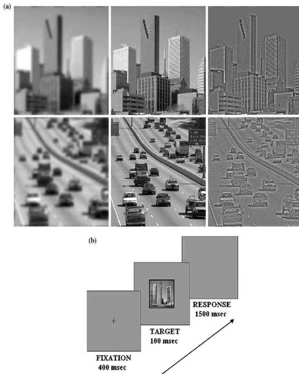
Fig. 2 a Examples of the filtered and non-filtered images of cities (top line) and highways (bottom line). From left to right: images are filtered in low spatial frequency (<math><4</math> cycles/degree), non-filtered, and filtered in high spatial frequency (>6 cycles/degree). b Time course of
