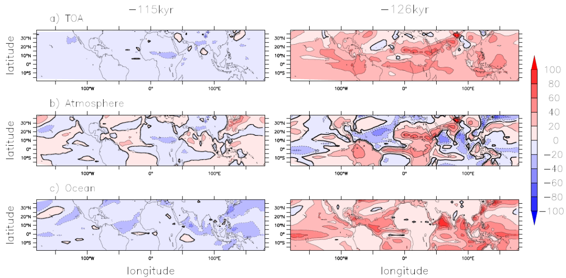
Fig. 10. Characteristics of the change in the ocean-atmosphere heat budget for 115 ka (left and 126 ka (right) and (a) Change in the net heat flux at the top of the atmosphere ( \text{W/m}^2 ) computed as the budget between shortwave and longwave radiation (positive downward), (b) the change in the total heat budget of the atmosphere ( \text{W/m}^2 ), considering a humid atmosphere, and (c) the change in the heat fluxes (positive downward) at the ocean surface ( \text{W/m}^2 ).
