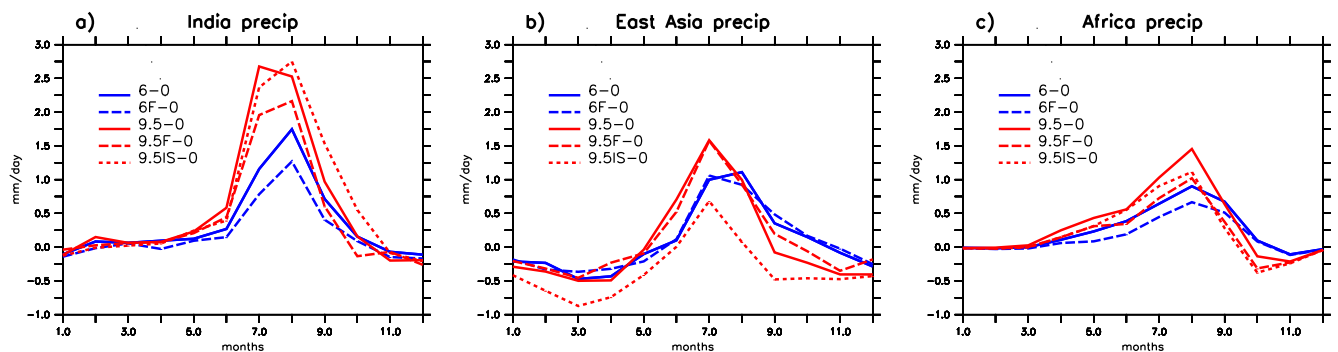
Figure 4. Seasonal cycle of continental rainfall (mm/day) difference with 0kyr BP for 6, 6F, 9.5, 9.5F, 9.5IS over a) India, b) East Asia, c) Africa
