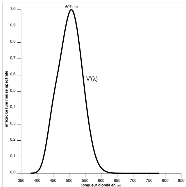
Figure 20: Efficacité relative spectrale scotopique
