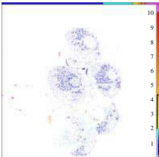
Figure 91: Sans cohérence spatiale
