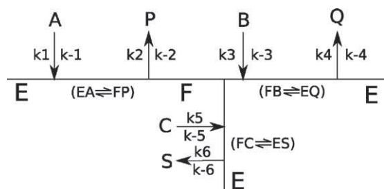
Fig. 1. Cleland representation. The enzyme (E), the acyl enzyme (F), the ester (A), the (R) and (S) alcohols (respectively B and C), the leaving alcohol product (P), the (R) and (S) ester products (respectively Q and S).
