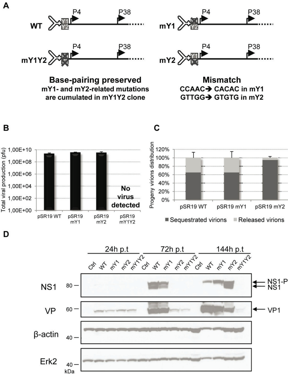
Figure 3: Effect of Y1- and/or Y2-box mutation on H-1 PV life cycle and NS1 protein expression.
