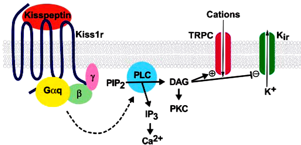
Figure 7. Proposed mechanism of neuronal depolarization by kisspeptin binding to its receptor, Kiss1r. Kisspeptin binding to its GPCR, Kiss1r, activates the G protein, Gα q , and PLC to cleave phosphatidylinositol 4,5-bisphosphate (PIP 2 ) into IP 3 and DAG. DAG activates a signal cascade by activating PKC, whereas IP 3 mobilizes calcium ions (Ca 2+ ), which participate in the cascade by activating other proteins. Membrane depolarization is caused by activation (+) of nonselective TRPC cation channels and inhibition (-) of inwardly rectifying potassium channels (K ir ), possibly through involvement of DAG. [Adapted from (Oakley et al., 2009)]
