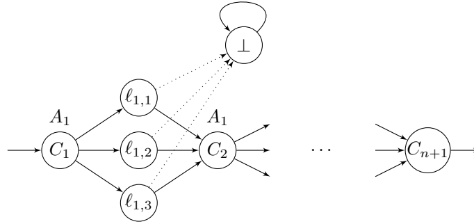
Figure 4.4: Module M(\phi) , where \phi = C_1 \wedge \dots \wedge C_n and C_i = \ell_{i,1} \vee \ell_{i,2} \vee \ell_{i,3}
